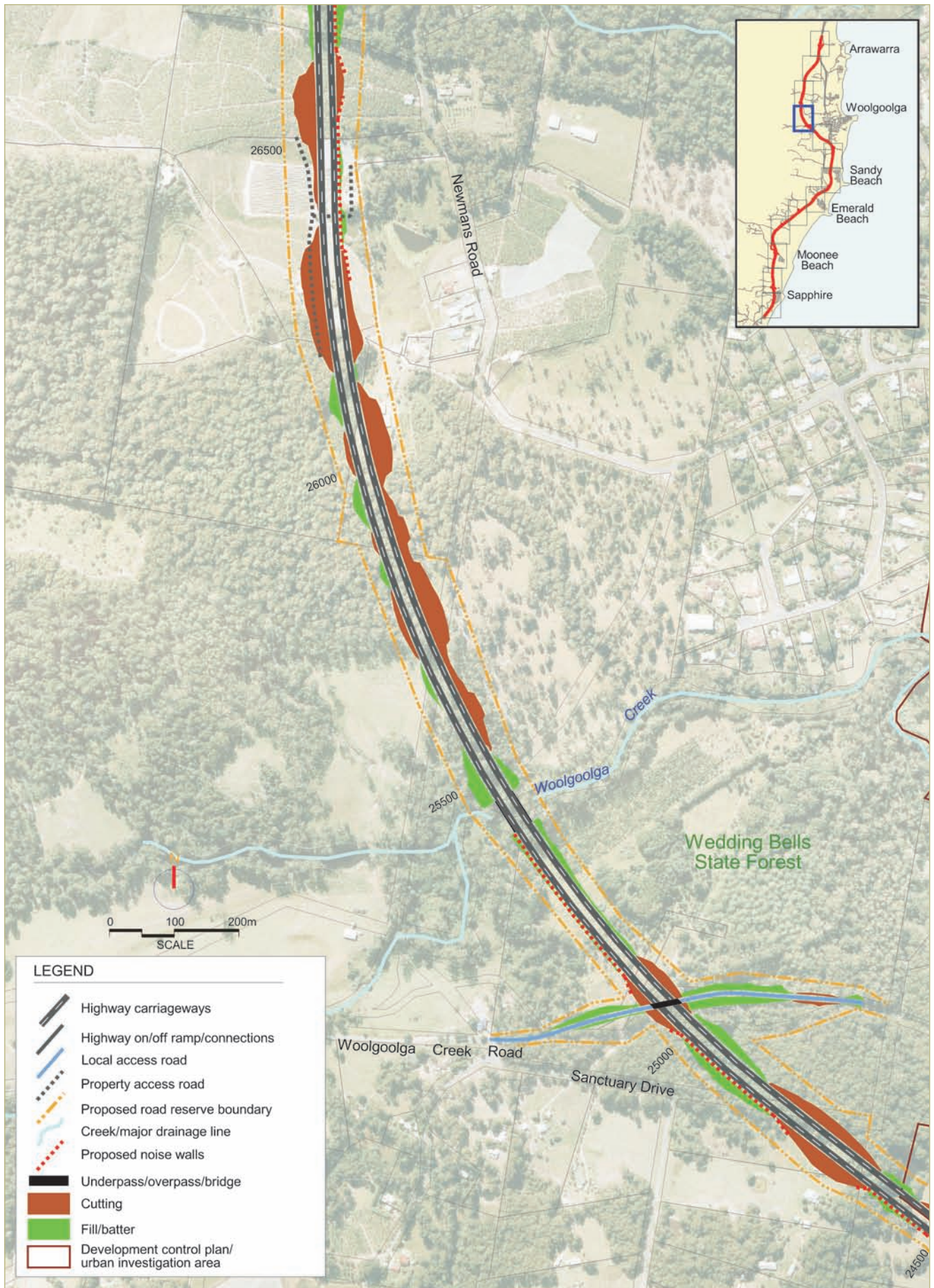
FIGURE 7.2j PROPOSED DESIGN
