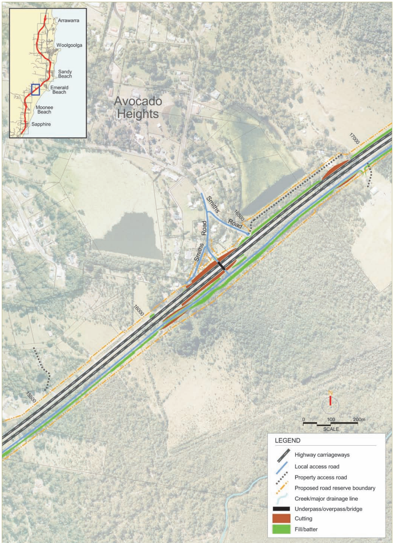
FIGURE 7.2e PROPOSED DESIGN
