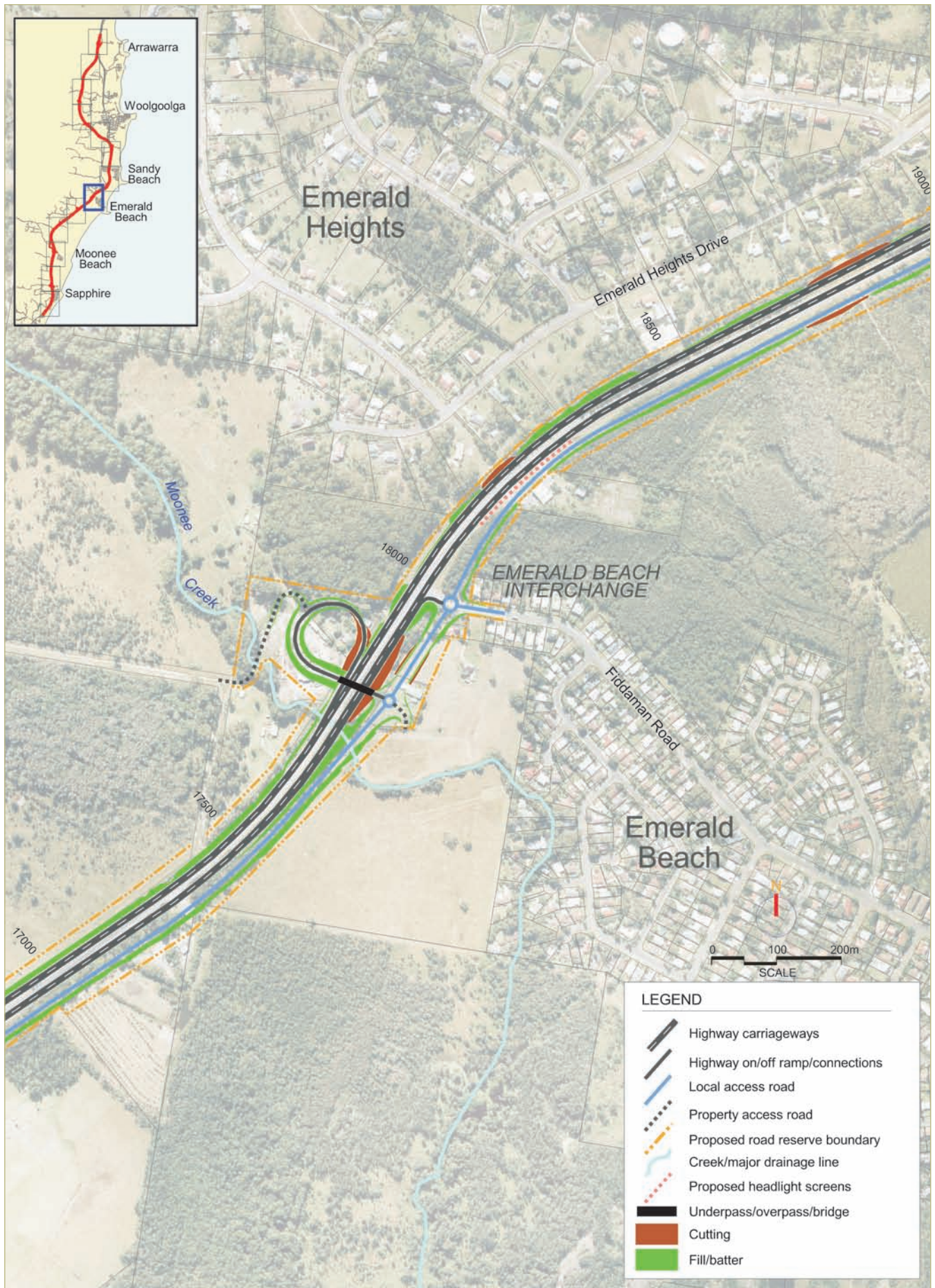
FIGURE 7.2f PROPOSED DESIGN
