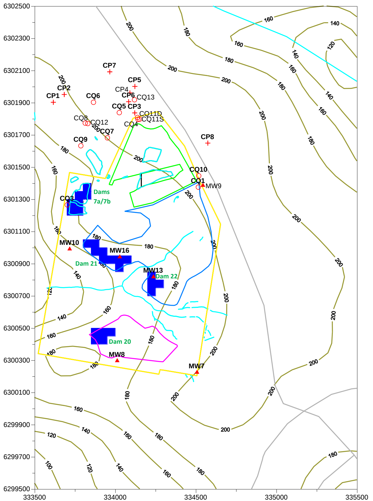
Figure 31. Predicted Watertable Elevation in Hawkesbury Sandstone after 200 Years [mAHD]
