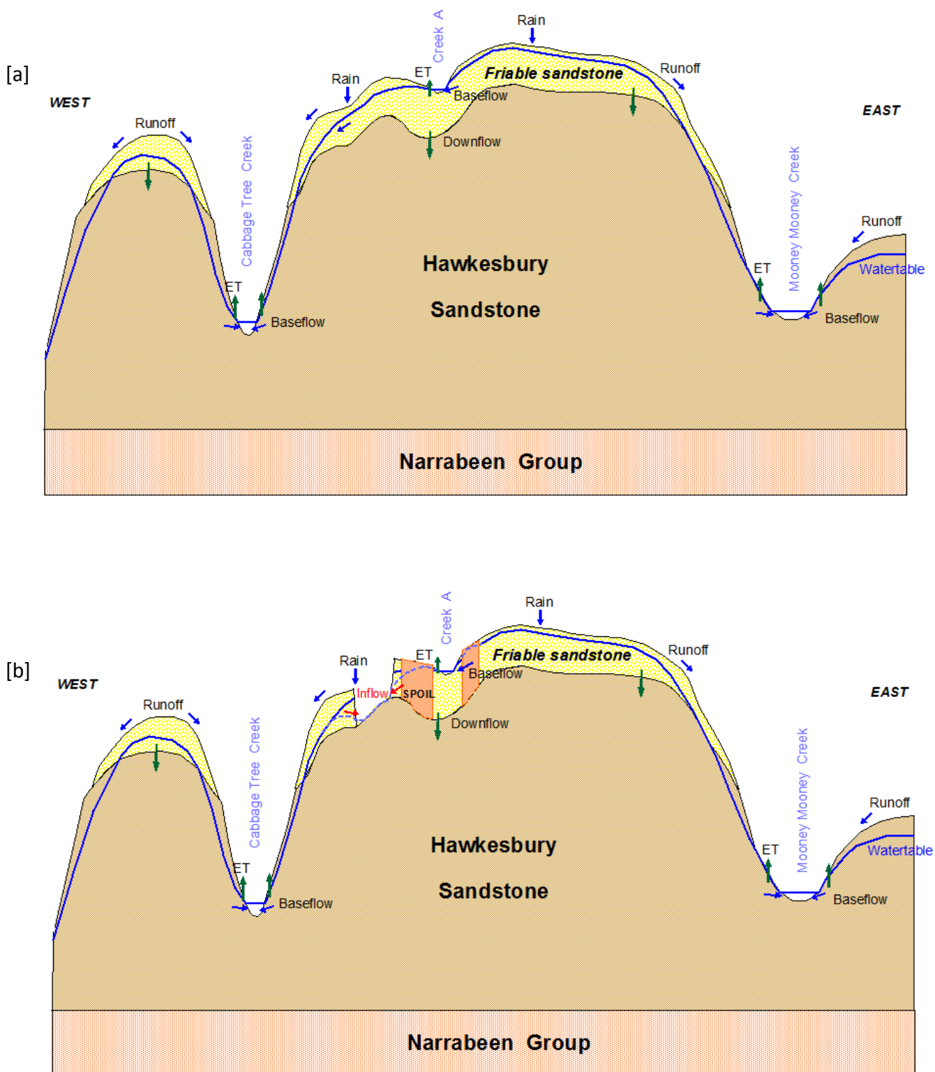
Figure 7. Local Hydrogeological Conceptual Model [a] Before Extraction; [b] During Extraction.
