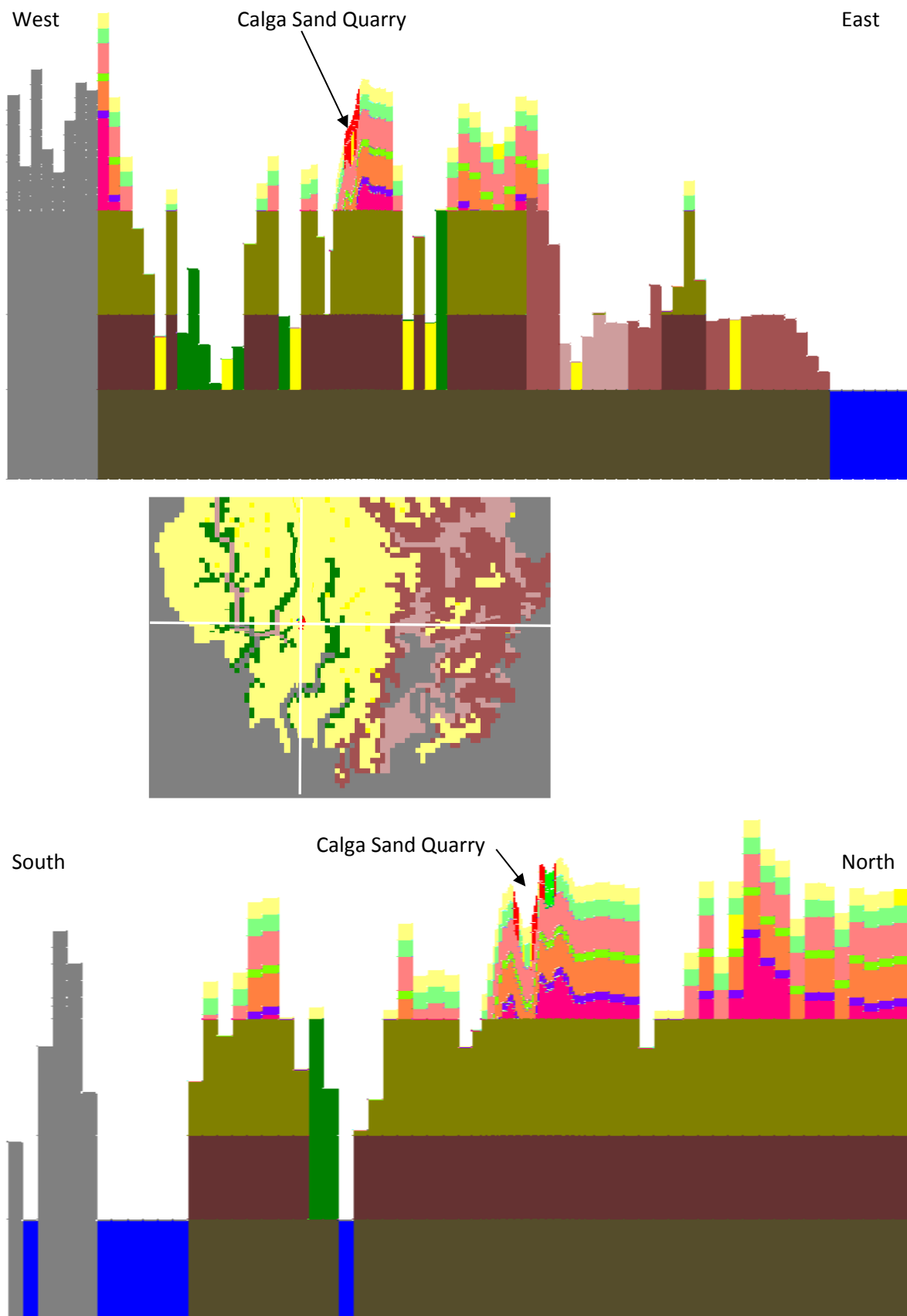
Figure 10. Representative Model Cross-sections through Calga Sand Quarry at Easting 334200 and Northing 6300900
