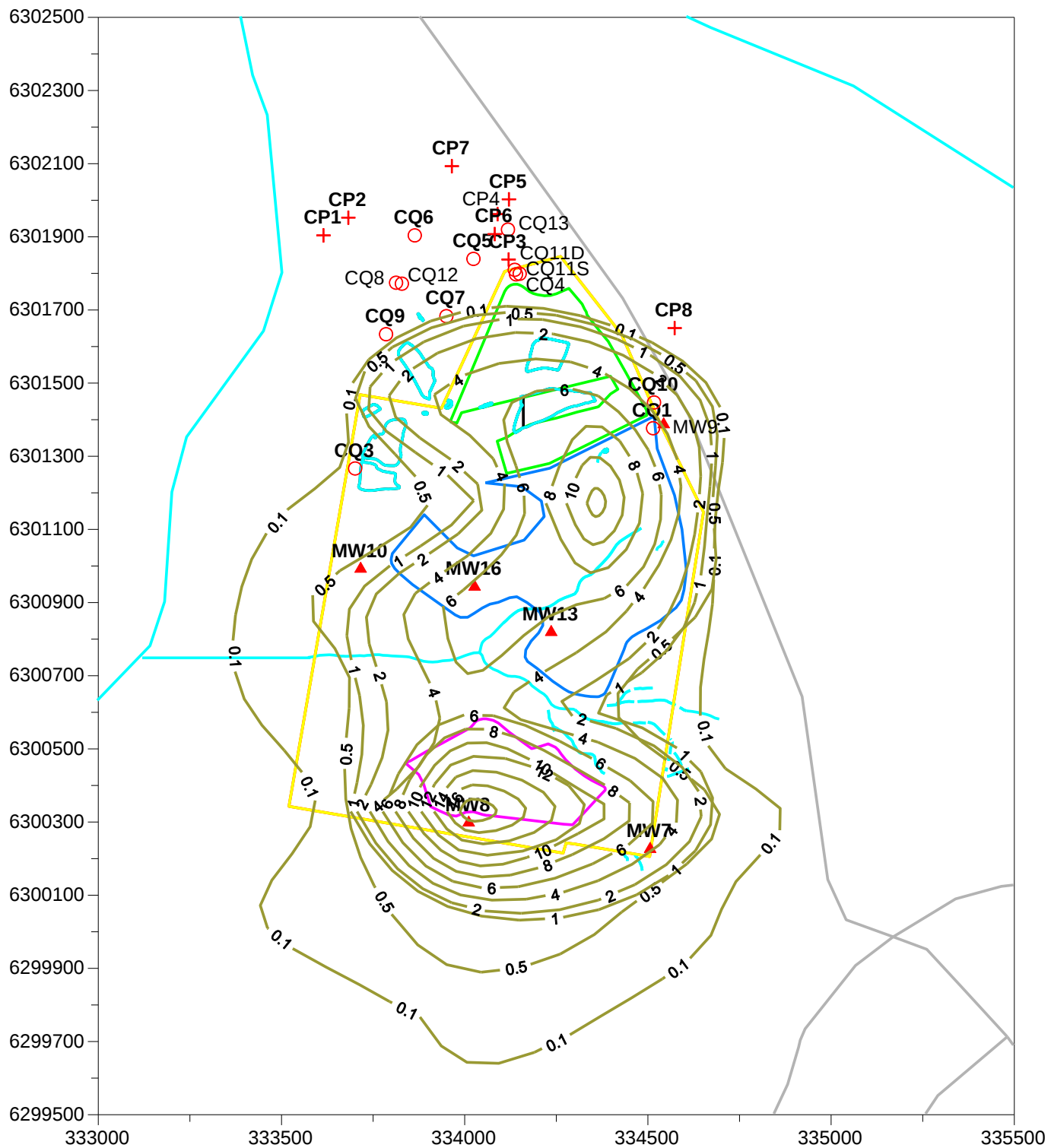
Figure 27. Predicted Watertable Drawdown (m) after 25 Years of Extraction
