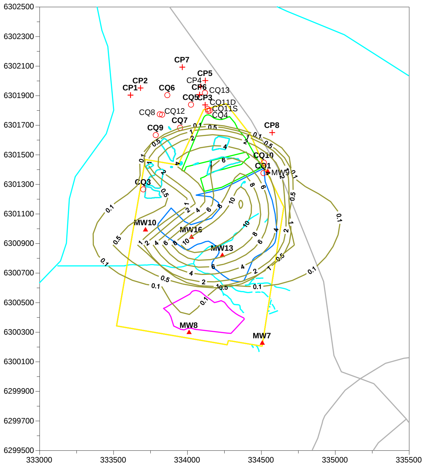
Figure 25. Predicted Watertable Drawdown (m) after 15 Years of Extraction
