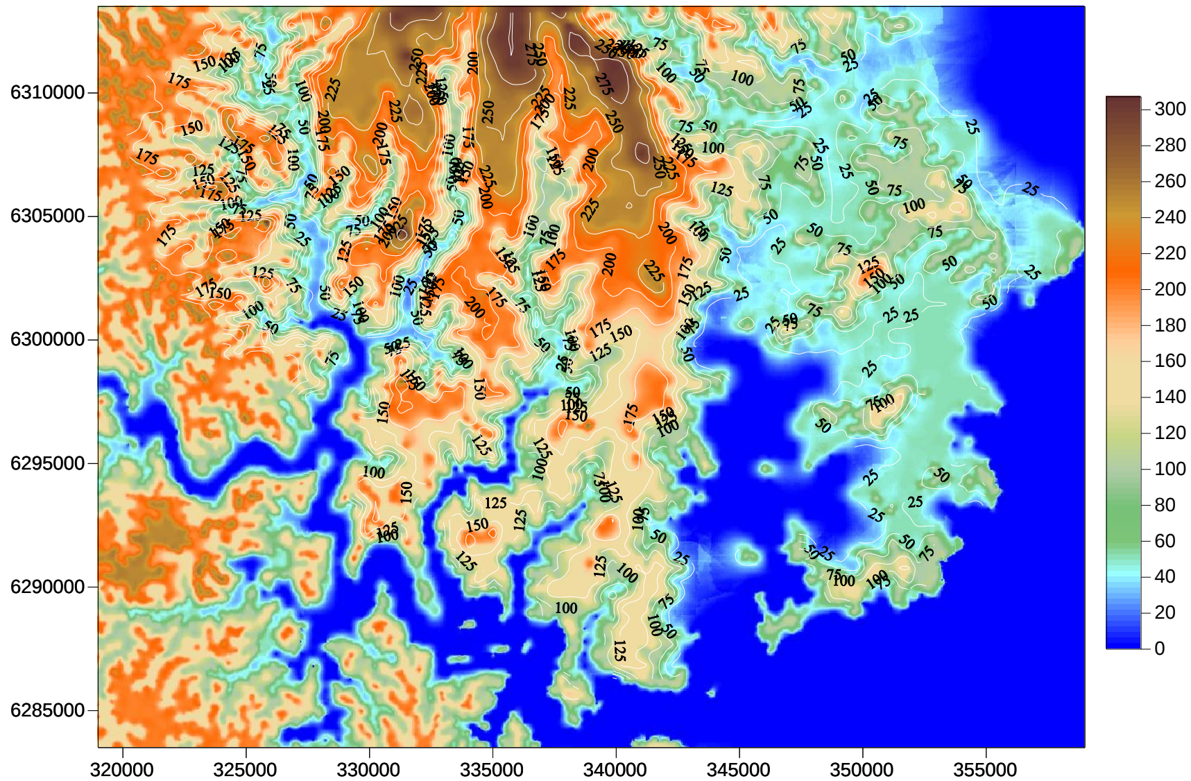
Figure 15. Simulated Steady State Watertable Contours in Model Layer 1 with Topography Underlay [mAHd]
