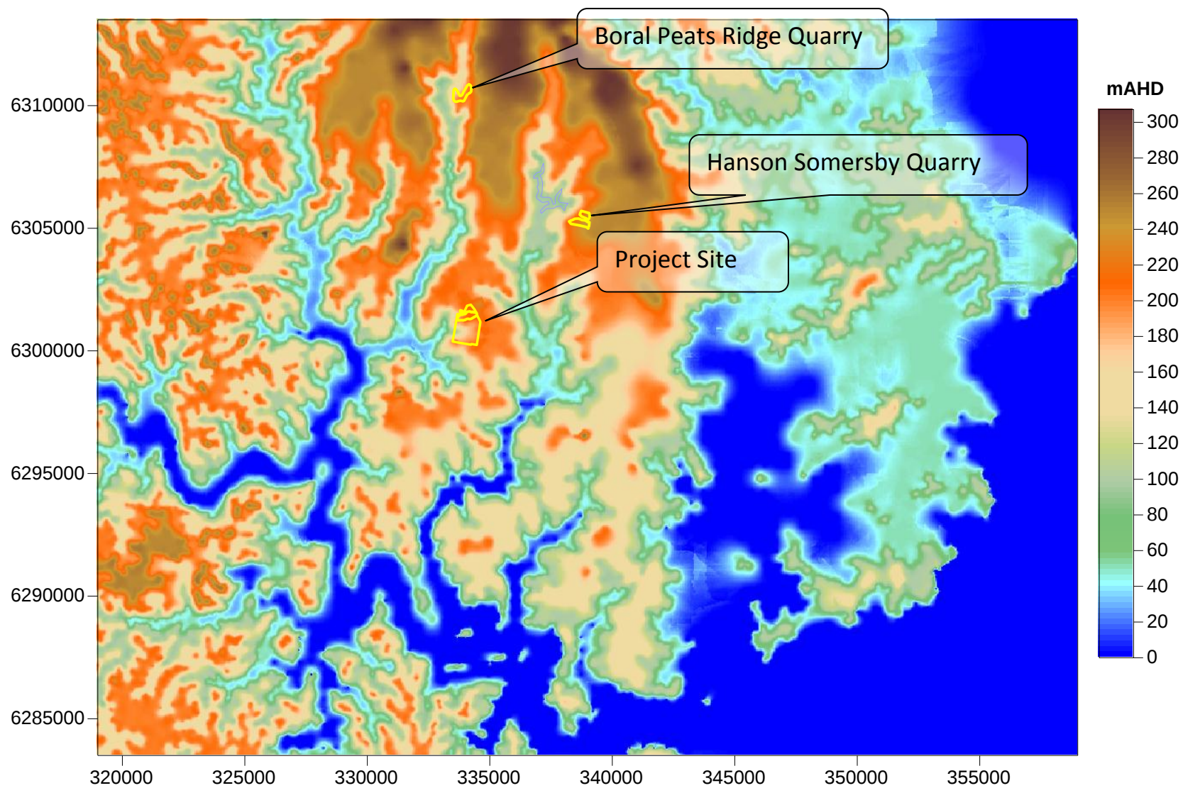
Figure 8. Topography across the Model Domain [mAHD]
