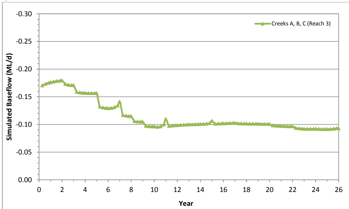
Figure 22. Predicted Baseflow: [a] For all reaches; [b] For Reach 3 (Creeks A, B, C)
