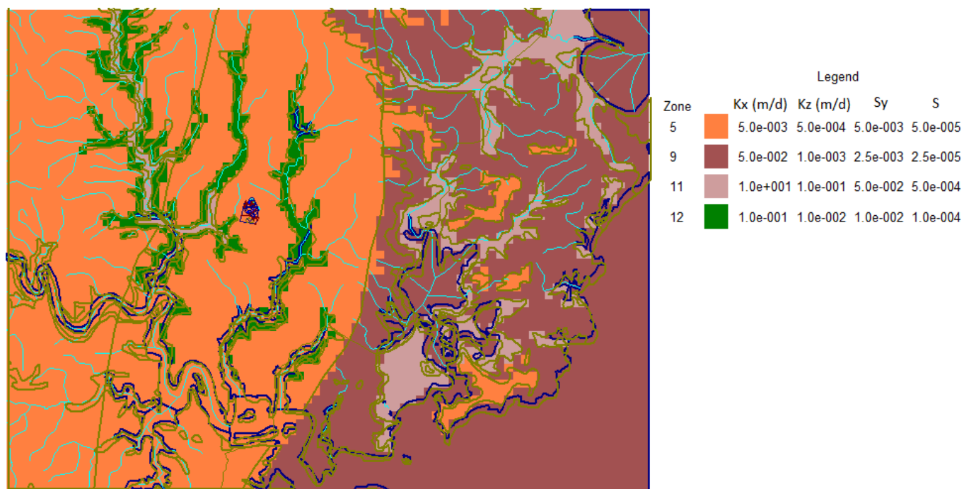
Figure AA-5. Hydraulic Property Zones for Layer 5
