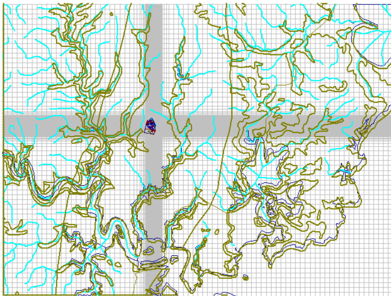
Figure 9. Model Grid with Geological Boundaries, Watercourses and Project Site. [cell dimension 50-500m]
