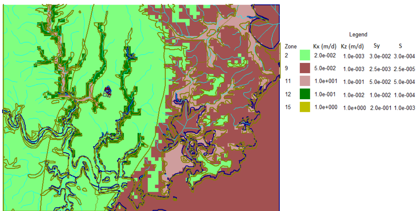
Figure AA-2. Hydraulic Property Zones for Layer 2
