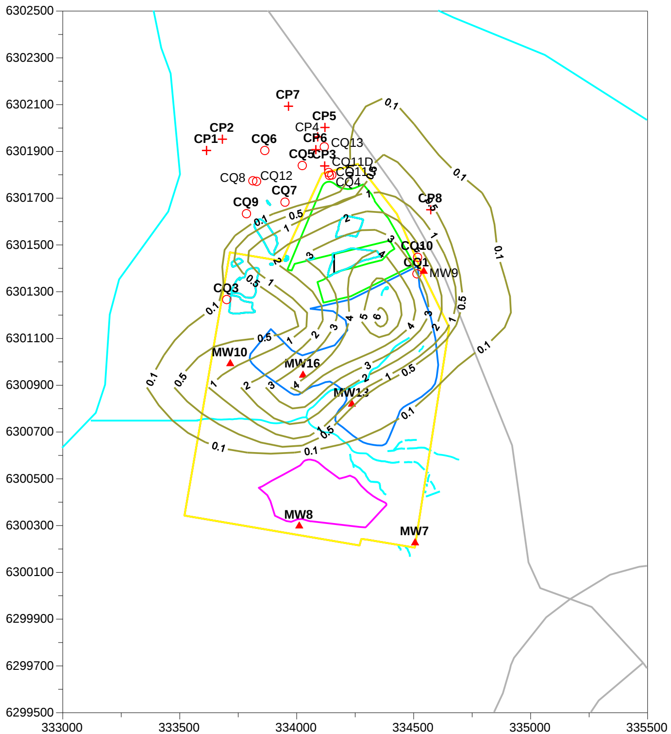
Figure 23. Predicted Watertable Drawdown (m) after 5 Years of Extraction
