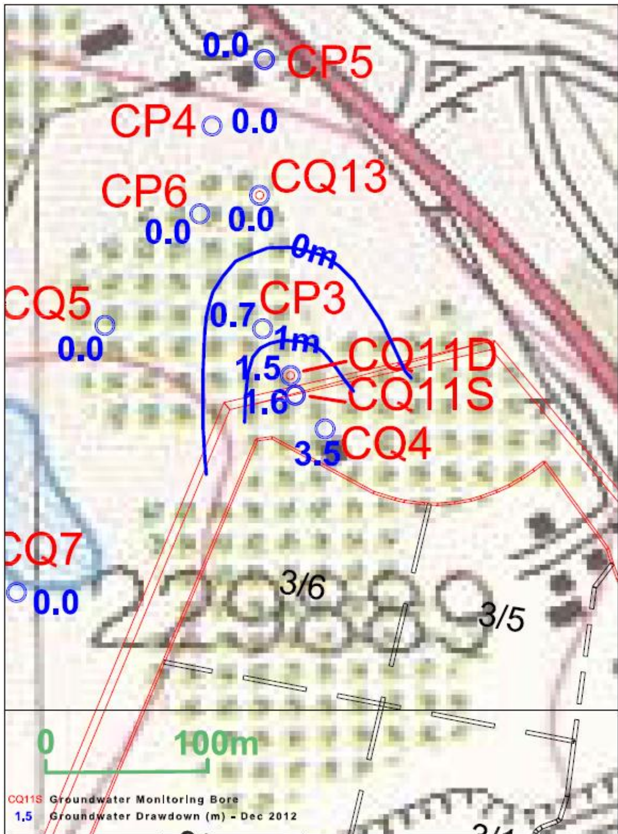
Figure 5. Groundwater Drawdown Attributed to Quarry Activity [after Dundon, 2013]
