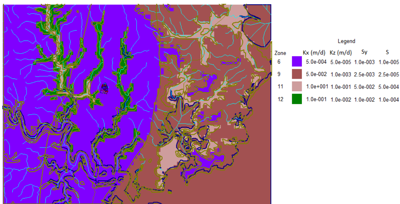
Figure AA-6. Hydraulic Property Zones for Layer 6
