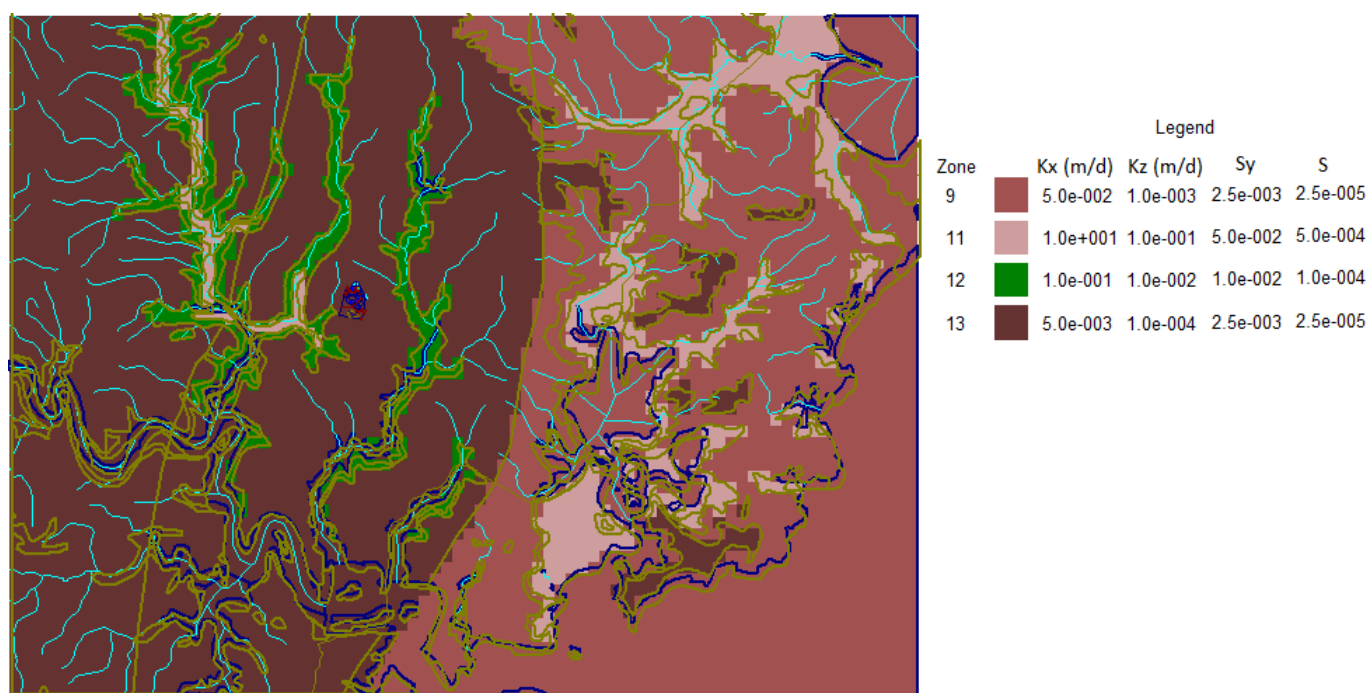
Figure AA-9. Hydraulic Property Zones for Layer 9
