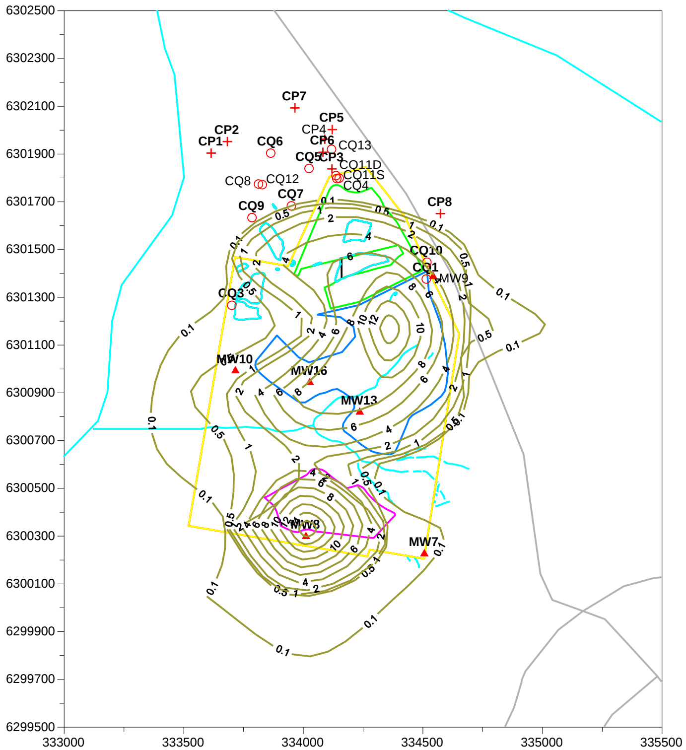
Figure 26. Predicted Watertable Drawdown (m) after 20 Years of Extraction
