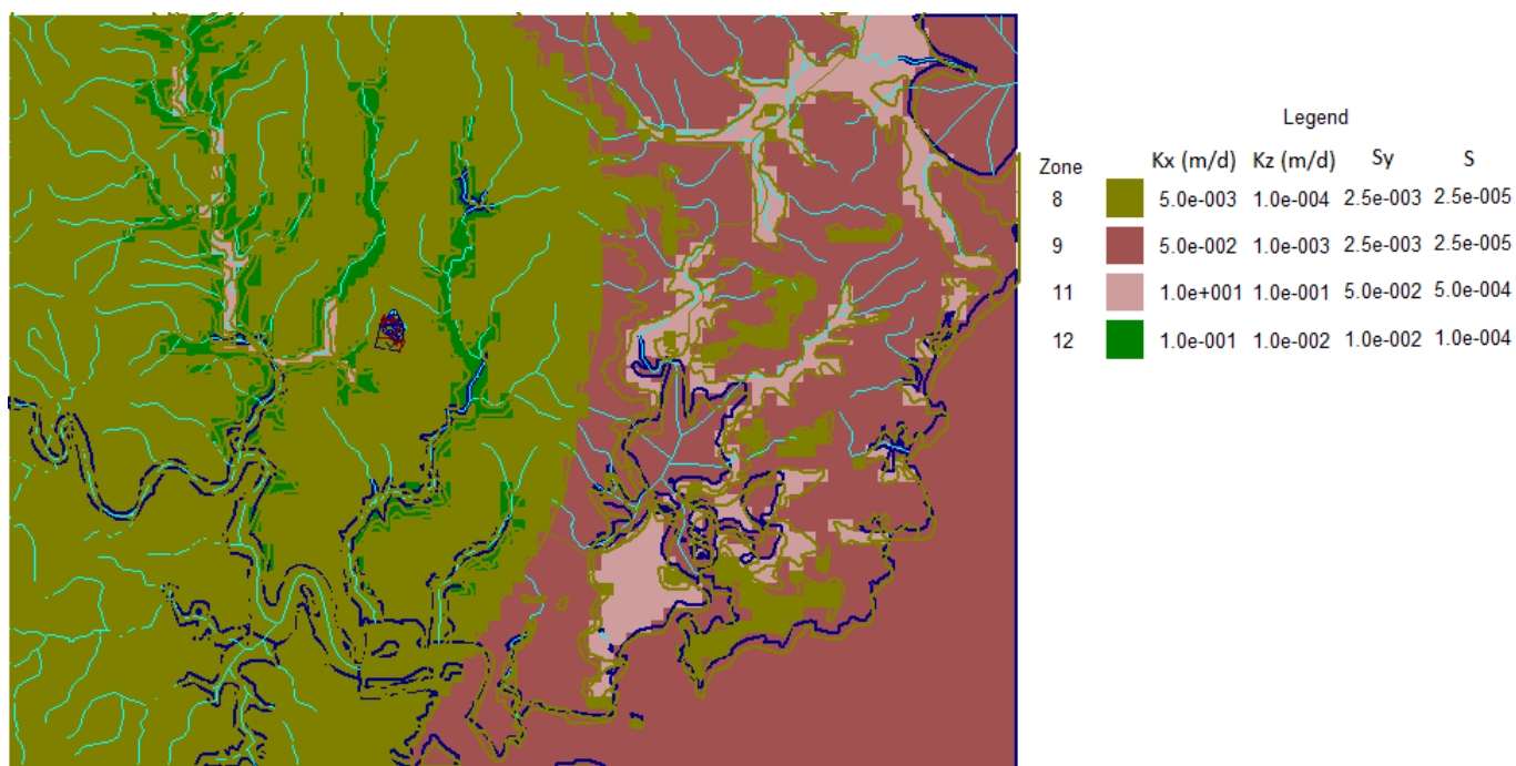
Figure AA-8. Hydraulic Property Zones for Layer 8
