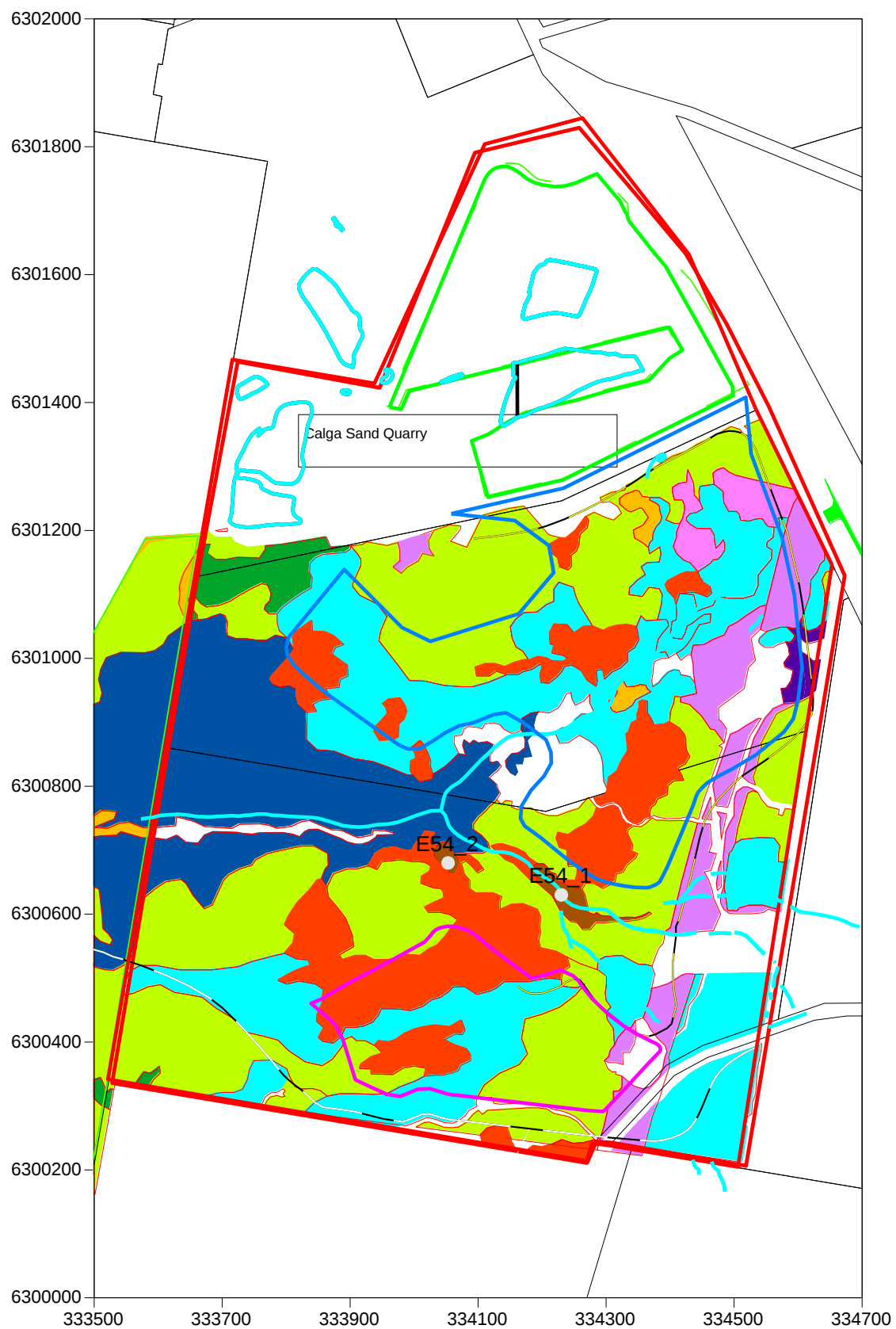
Figure 33. Hypothetical Bores (E54_1 and E54_2) Location Map on E54 areas
