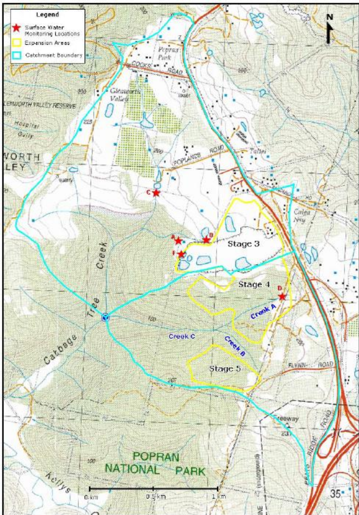
Figure 3. Catchments draining to Cabbage Tree Creek [after Evans & Peck, 2008]
