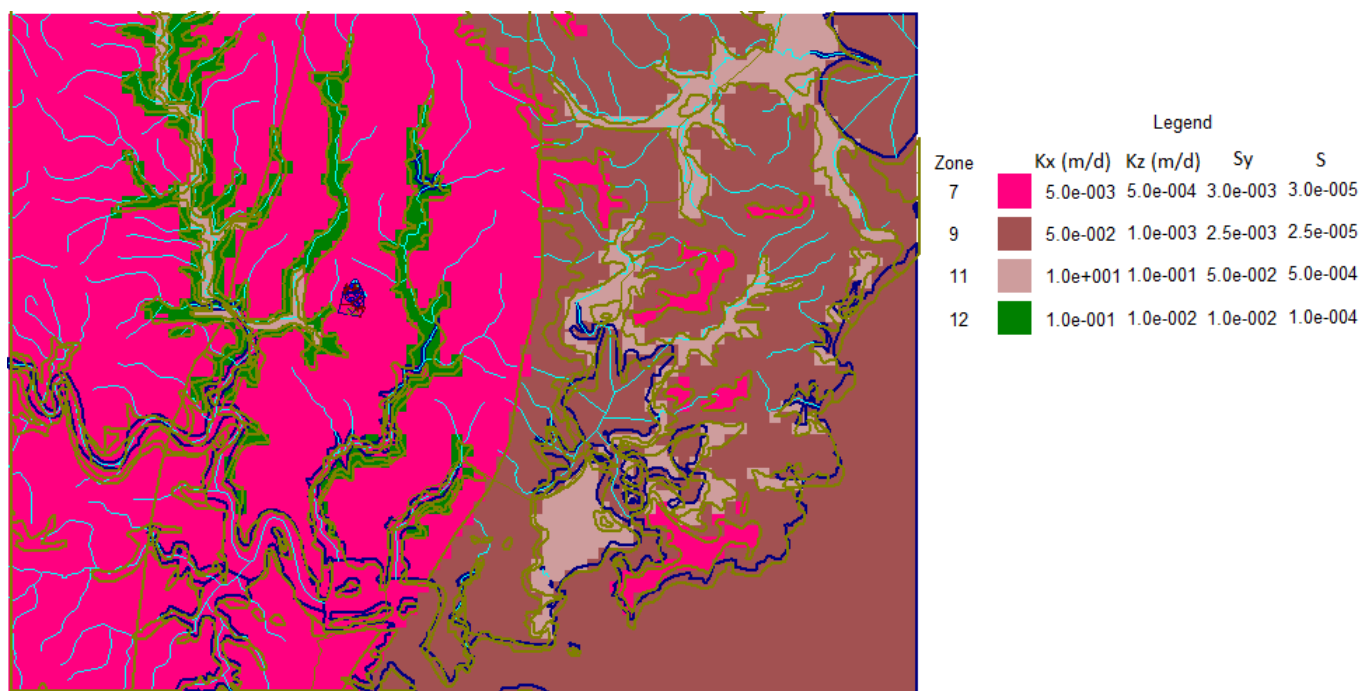
Figure AA-7. Hydraulic Property Zones for Layer 7
