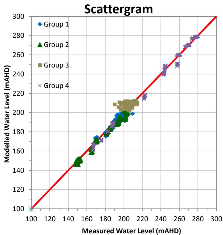
Figure 17. Scattergram of Simulated and Measured Heads for Transient Calibration
