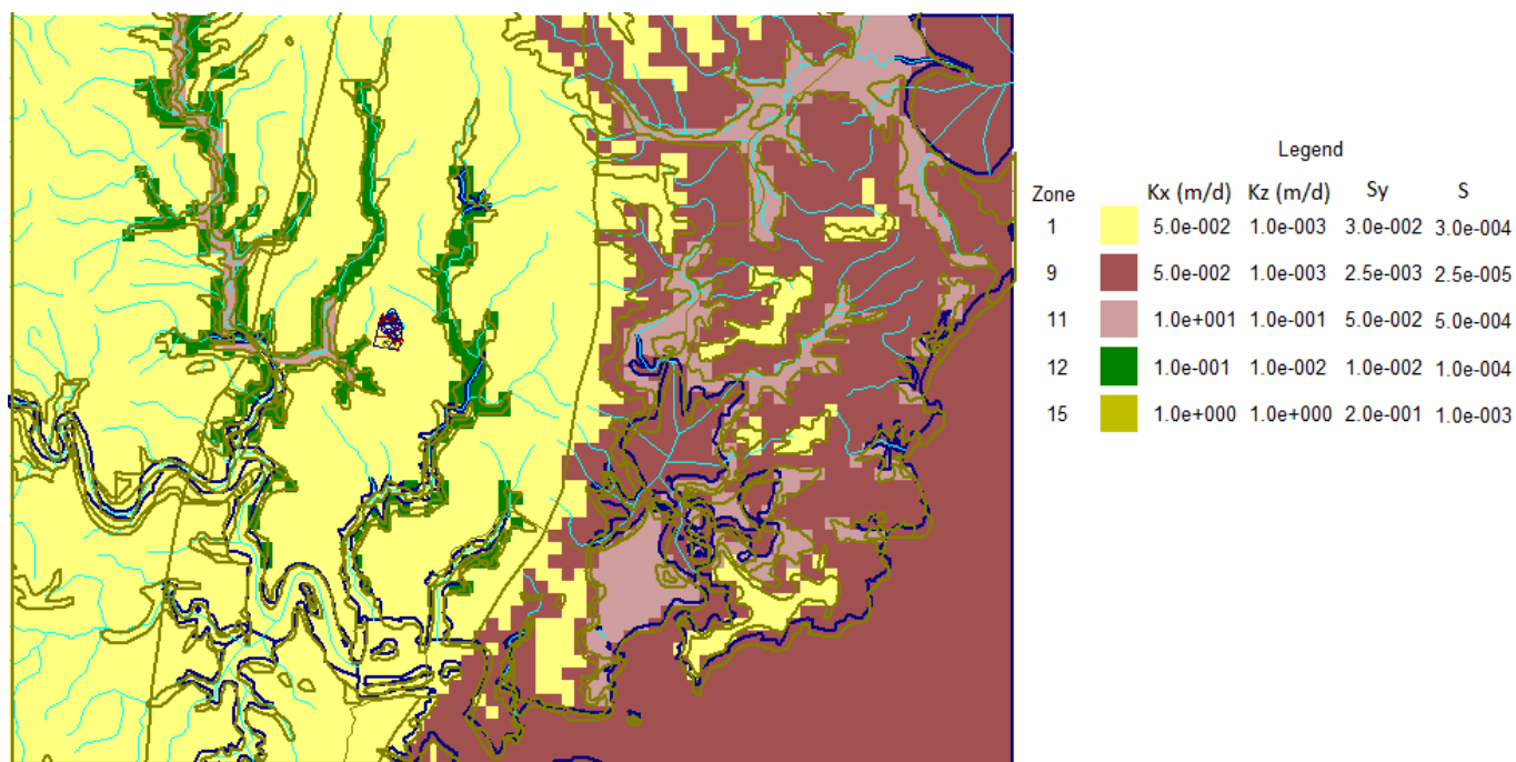
Figure AA-1. Hydraulic Property Zones for Layer 1
