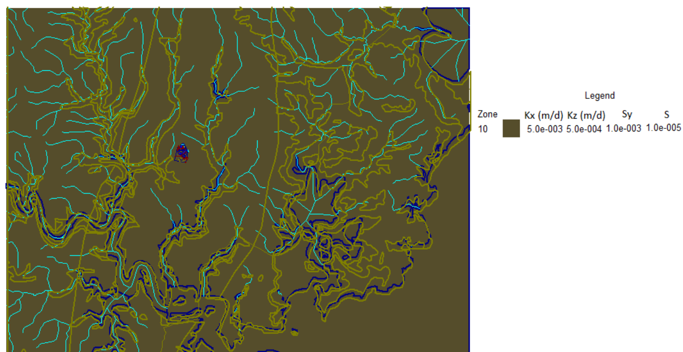
Figure AA-10. Hydraulic Property Zones for Layer 10
