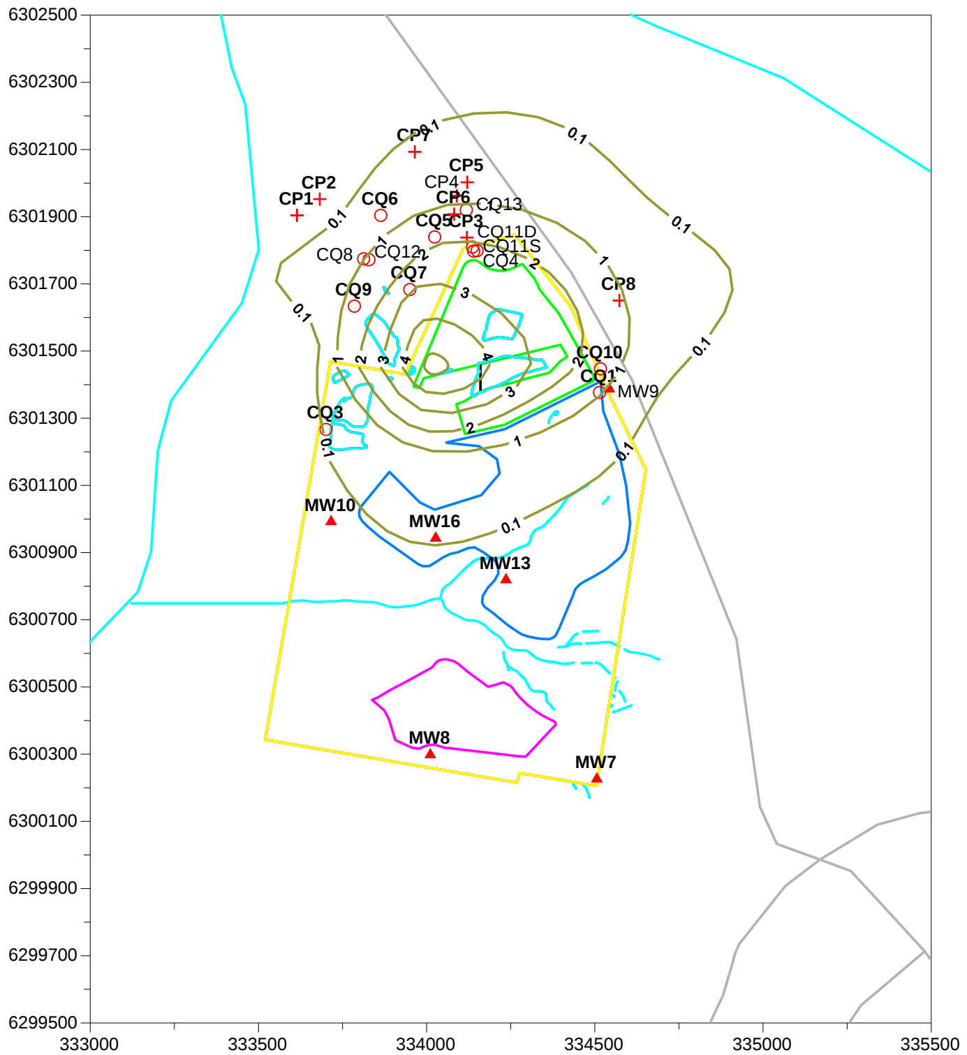
Figure 20. Simulated Watertable Drawdown at December 2012
