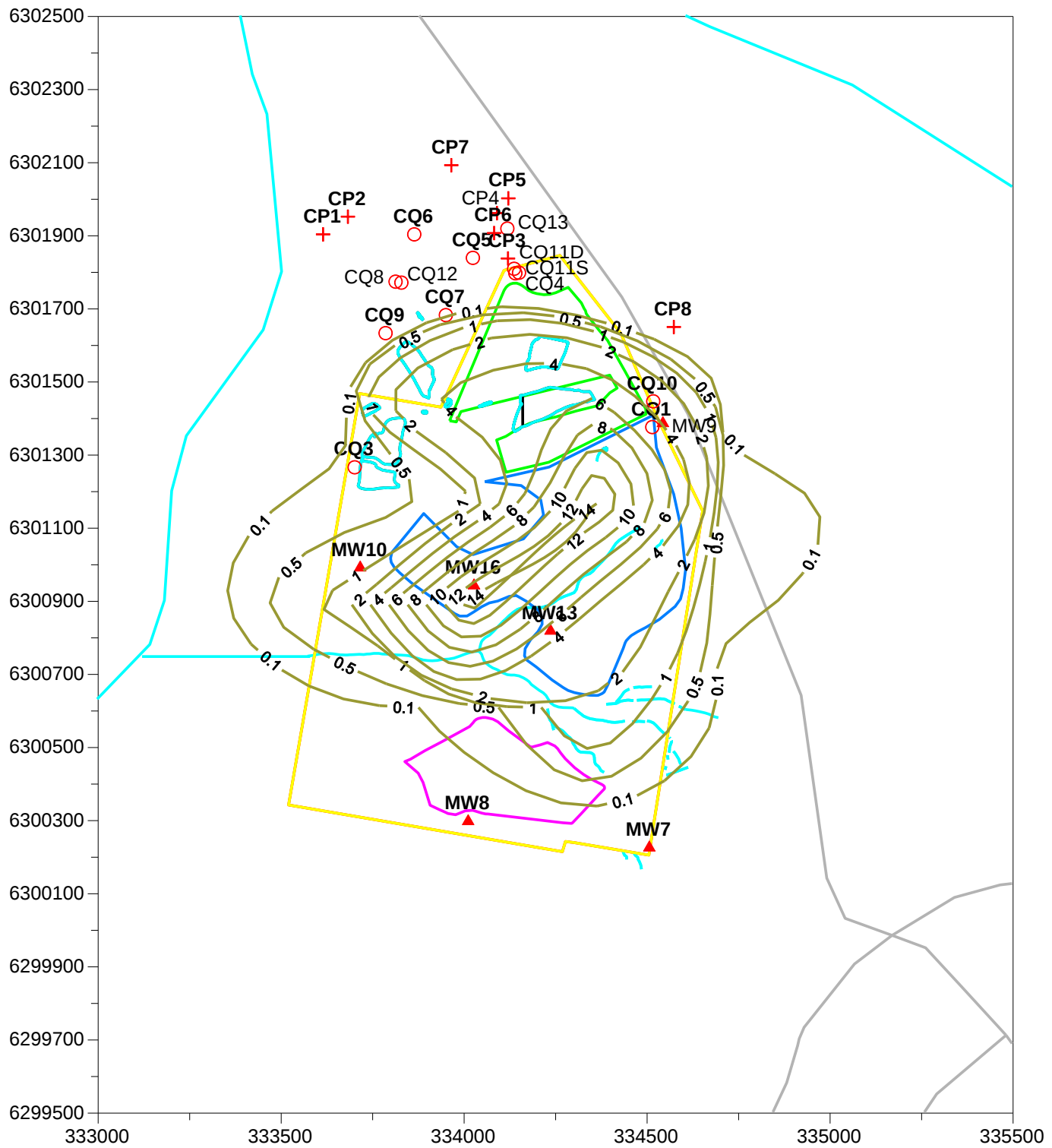
Figure 24. Predicted Watertable Drawdown (m) after 10 Years of Extraction
