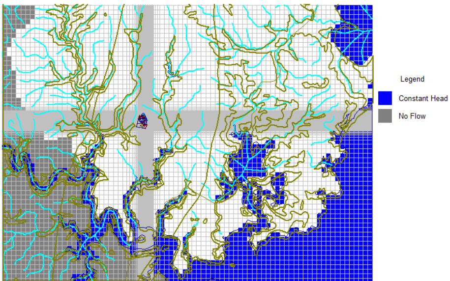
Figure 11. Model Boundary Conditions: [a] Layer 1; [b] Layer 9 and [c] Layer 10
