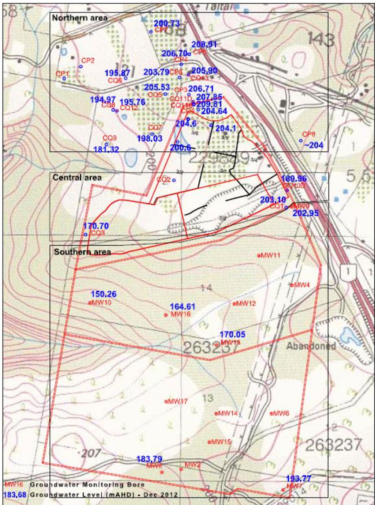
Figure 4. Groundwater Monitoring Bore Network [after Dundon, 2013]
