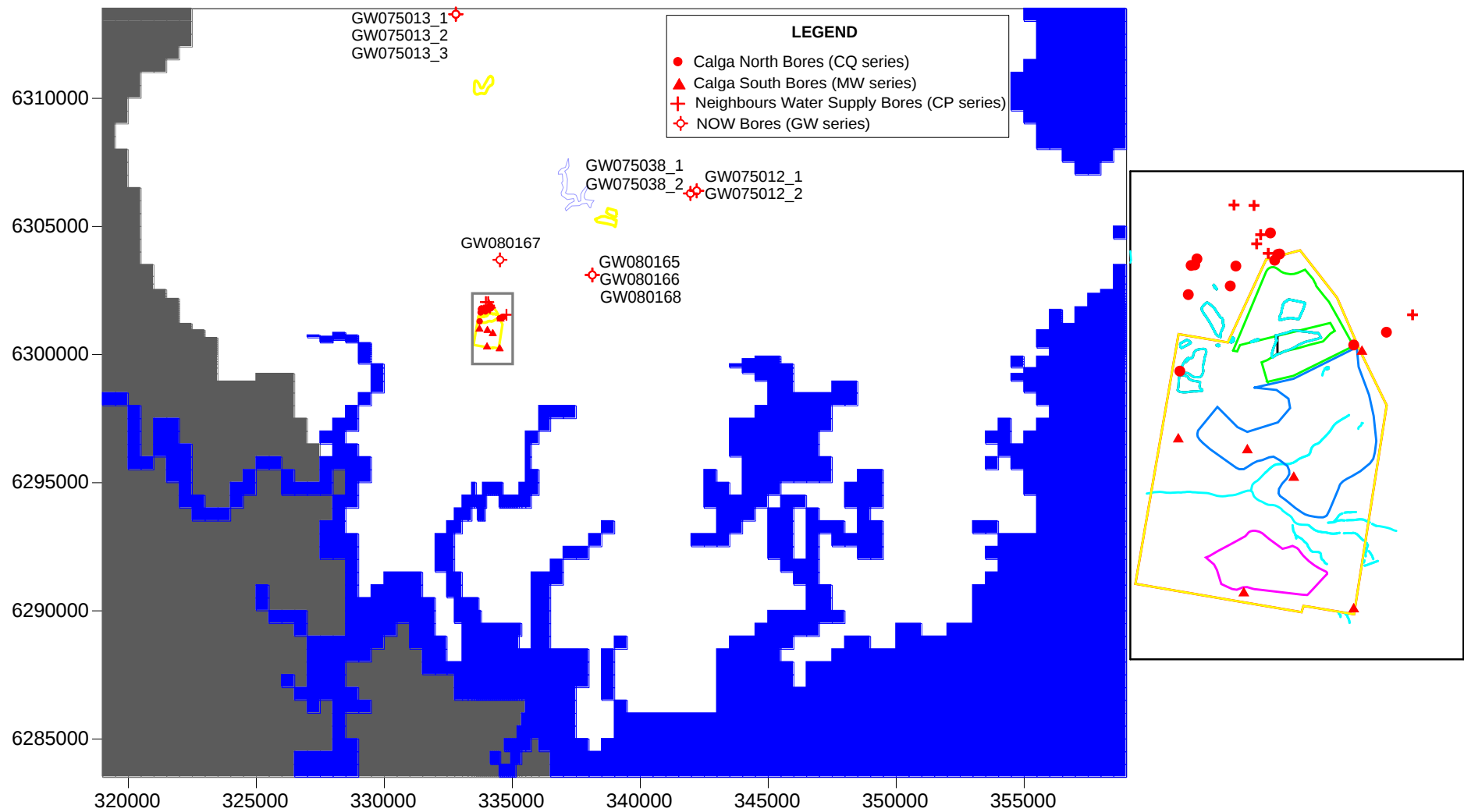
Figure 14 Locations of Monitoring Bore Calibration Sites
