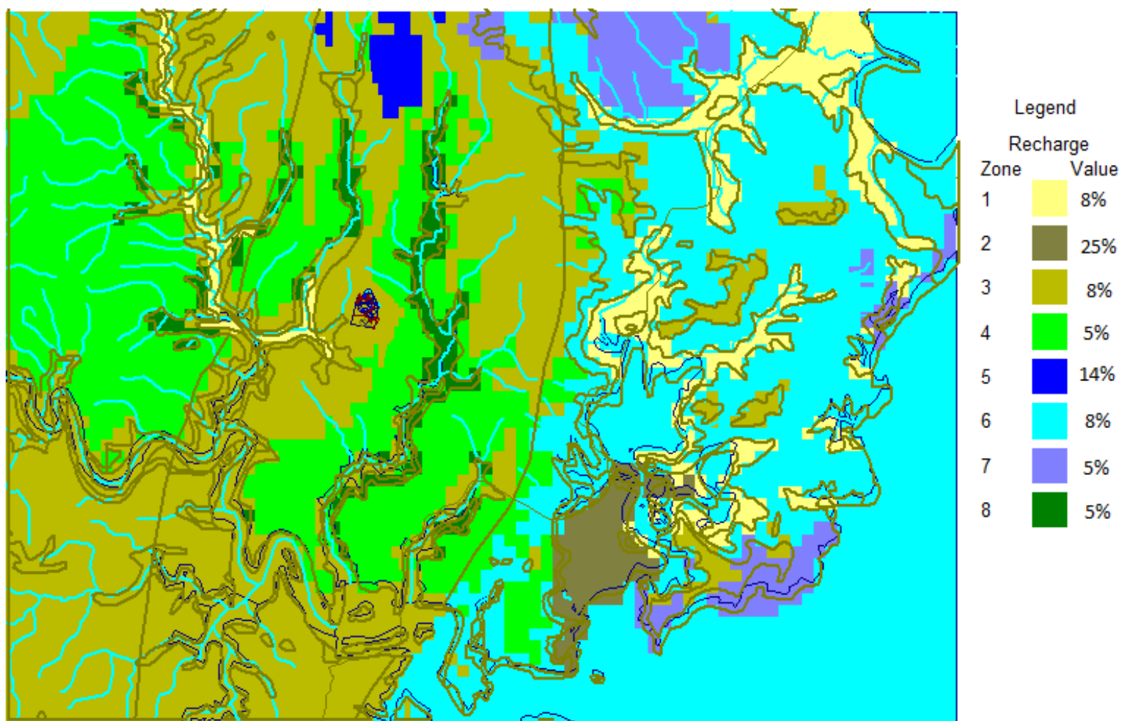
Figure 13. Rainfall Recharge Distribution as a Percentage of Rainfall
