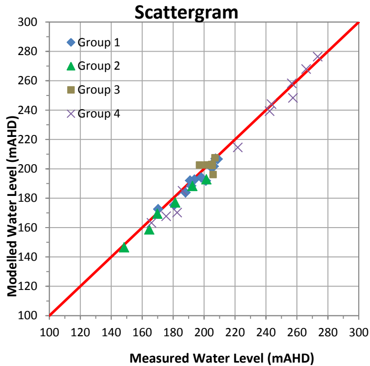
Figure 16. Scattergram of Simulated and Measured Heads for Steady State Calibration
