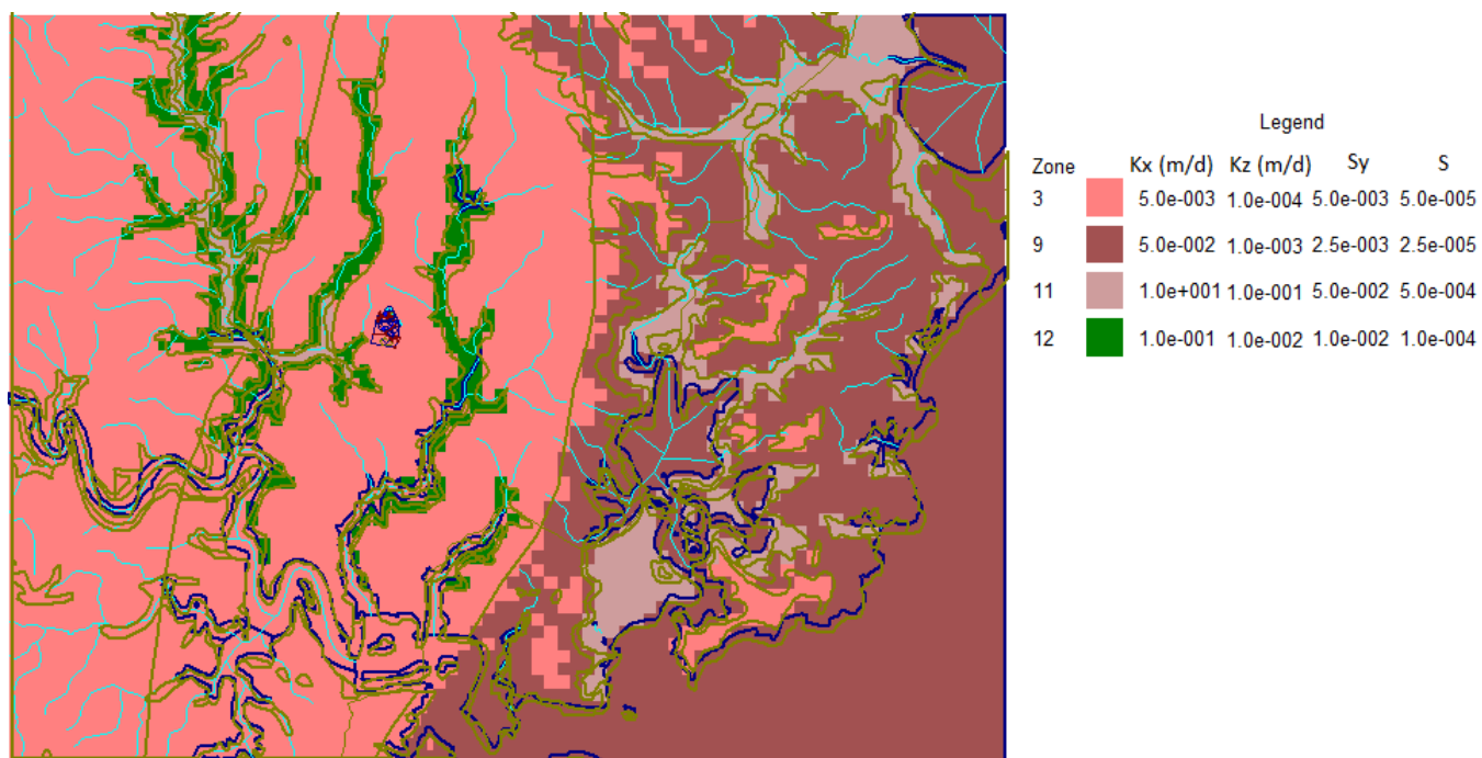
Figure AA-3. Hydraulic Property Zones for Layer 3
