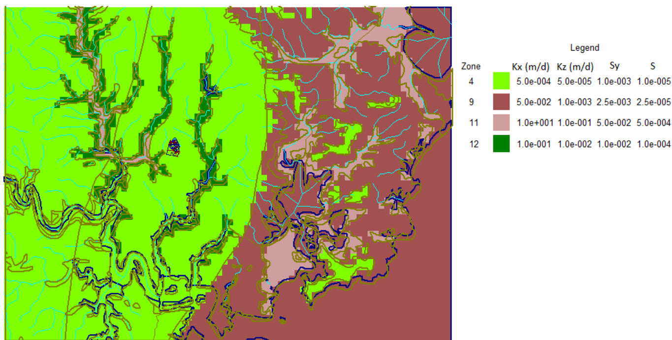
Figure AA-4. Hydraulic Property Zones for Layer 4
