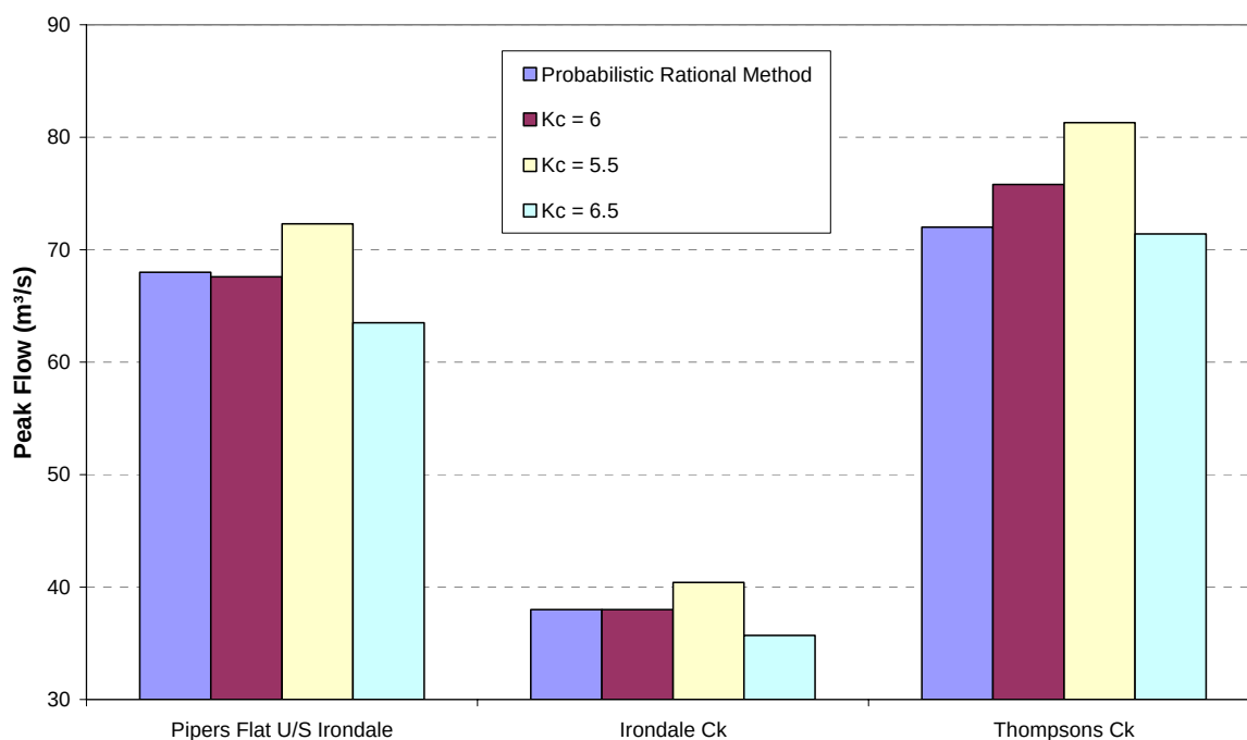
■ Figure 3-1: Test of sensitivity of peak flow estimates to k_c with IL=6.0 and CL=2.5.
