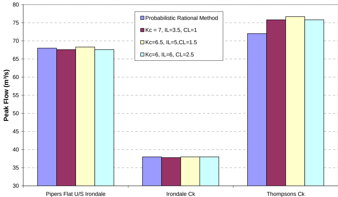
■ Figure 3-4: Comparison of RORB estimates with those from PRM for 100 year ARI storm event.
