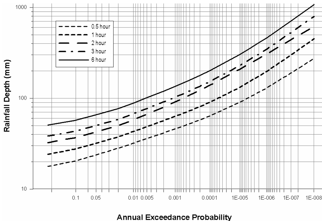
■ Figure 3-5: Design rainfall depths.
