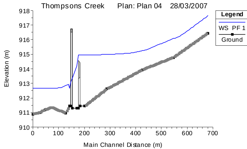
■ Figure 4-1: Thompsons Creek inlet for existing conditions.
