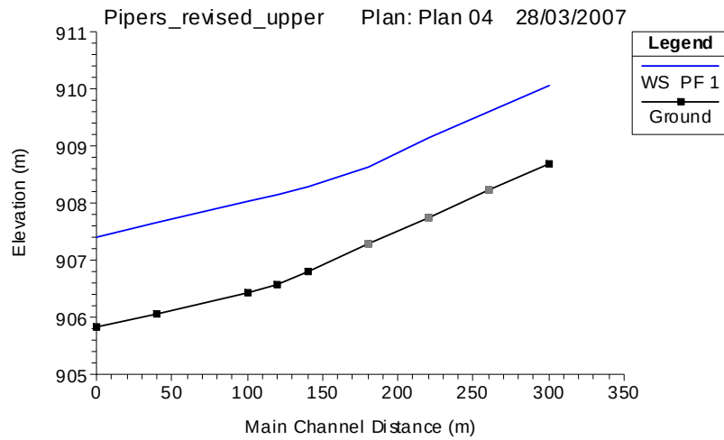
■ Figure 4-5: Pipers Creek inlet for existing conditions.
