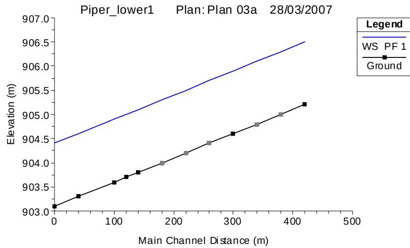
■ Figure 4-7: Pipers Creek outlet for existing conditions.
