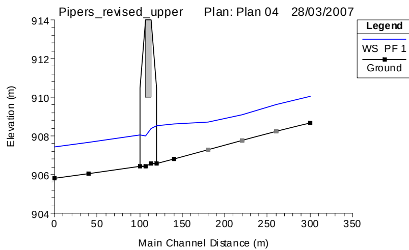
■ Figure 4-6: Pipers Creek outlet for proposed conditions.
