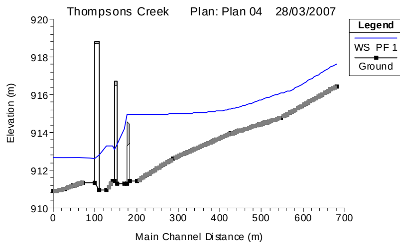
■ Figure 4-1: Thompsons Creek inlet for existing conditions.
