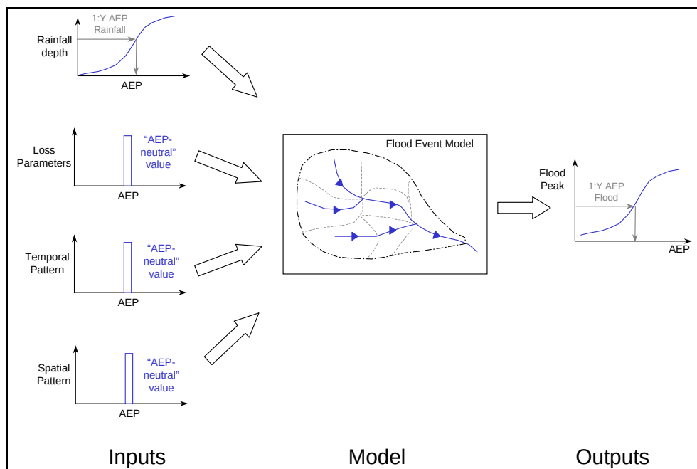
■ Figure 3-6 Schematic illustration of the design event approach
