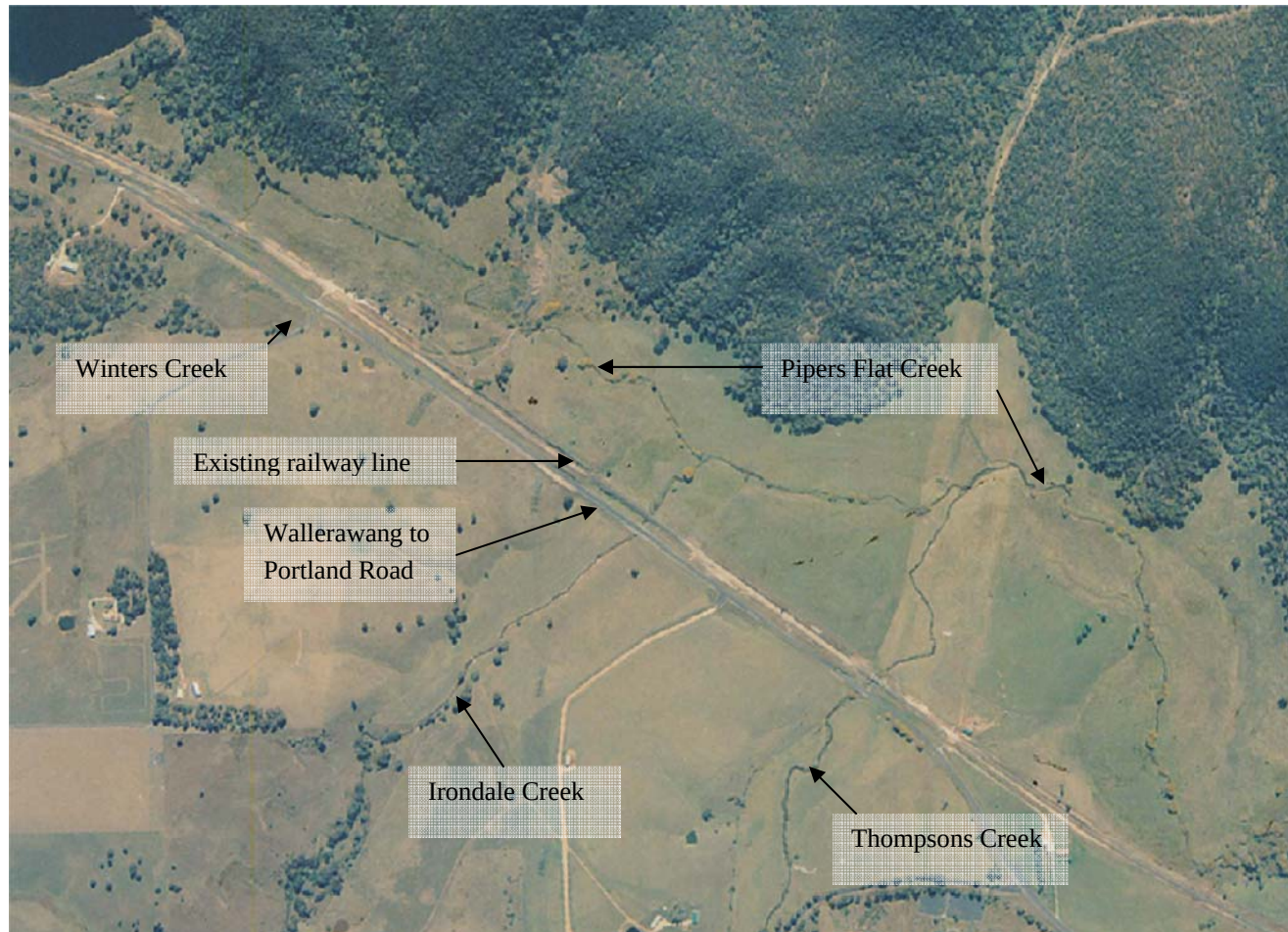
■ Figure 2-2: Existing Infrastructure and waterway crossings at Pipers Flat
