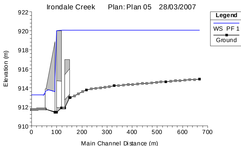
■ Figure 4-3: Irondale Creek inlet for existing conditions.
