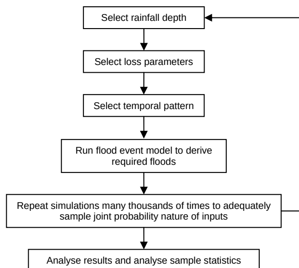
■ Figure 3-8: Overview of adopted joint probability framework
