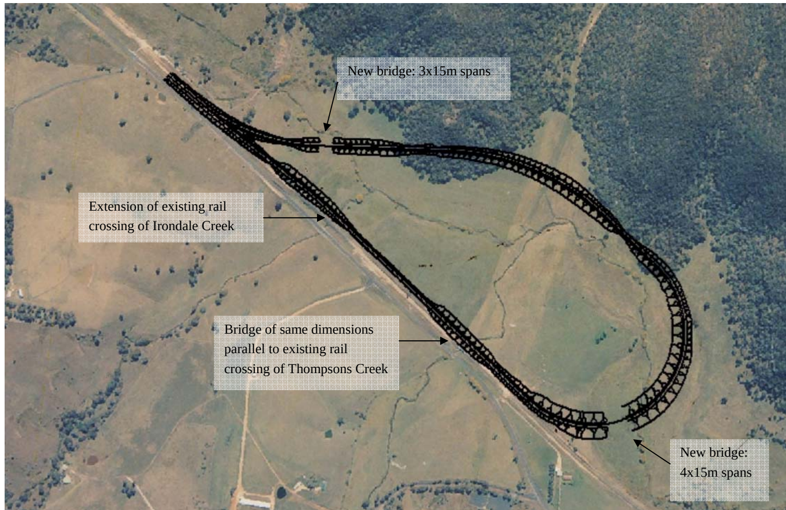
■ Figure 2-3: Proposed design of loop and additional waterway crossings at Pipers Flat
