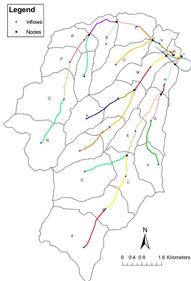
■ Figure 3-1: RORB model layout.
