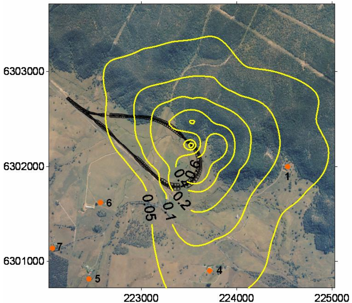
■ Figure 5-6 Monthly Dust Deposition Contours – Coal Transfer Operations ( \text{g}/\text{m}^2/\text{month} )
