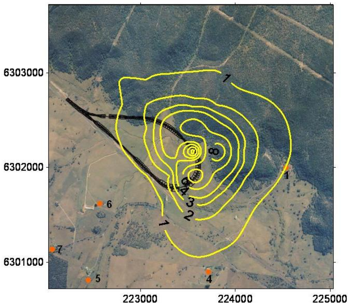
■ Figure 5-9 TSP Contours – Coal Transfer Operations ( \mu\text{g}/\text{m}^3 )
