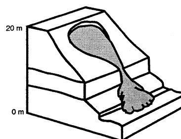
Figure B1 Types of movement: (a) fall, (b) topple, (c) slide, (d) spread, (e) flow. broken lines indicate original ground surfaces; arrows show portions of trajectories of individual particles of displaced mass; scales indicative for example chosen only (from “Landslides”, copyright Registration Number 427735 of Consumer and Corporate Affairs, Canada, by kind permission of the author D.M. Cruden).
