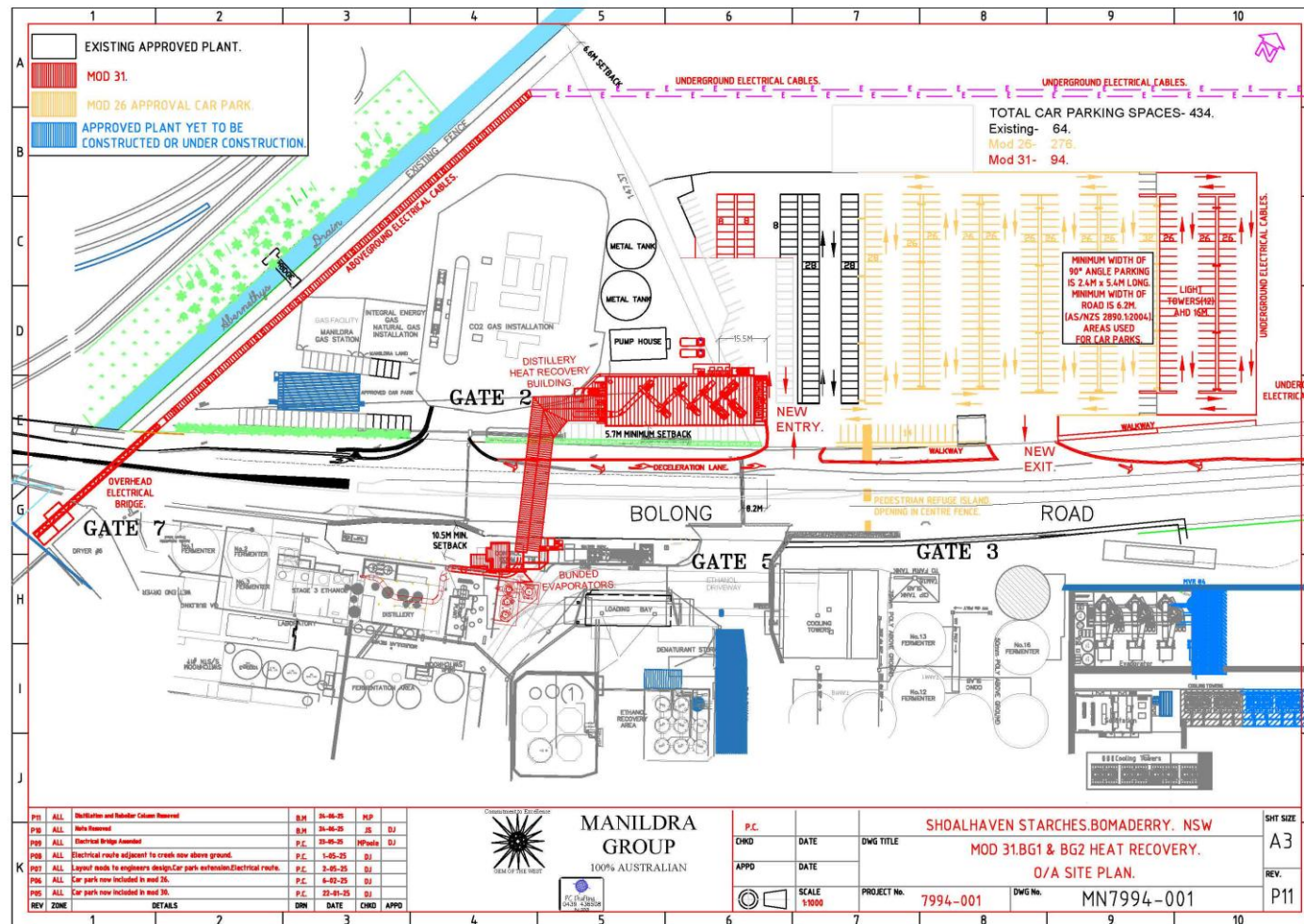
Figure 6 – Distillery Layout Showing Modifications
