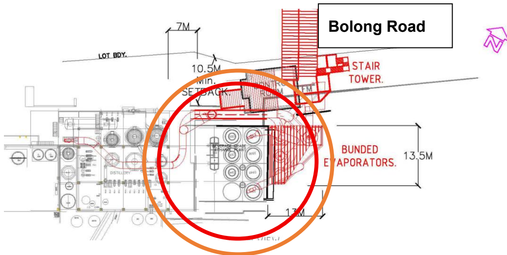
Figure 17 – Distillery Heat Recovery Bund Radiant Heat Contours
