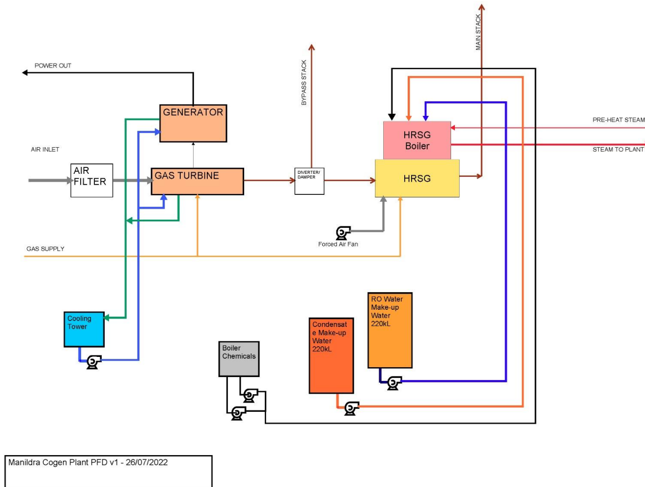
Figure 8 – Cogen Plant Process Flow Diagram
