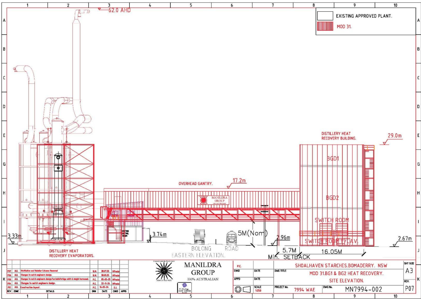
Figure 7 - Distillery Elevation Showing Modifications
