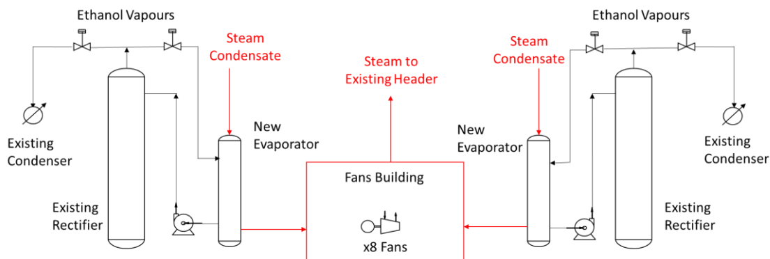
Figure 5 – Process Flow Diagram for One Beverage Grade Ethanol Plant
