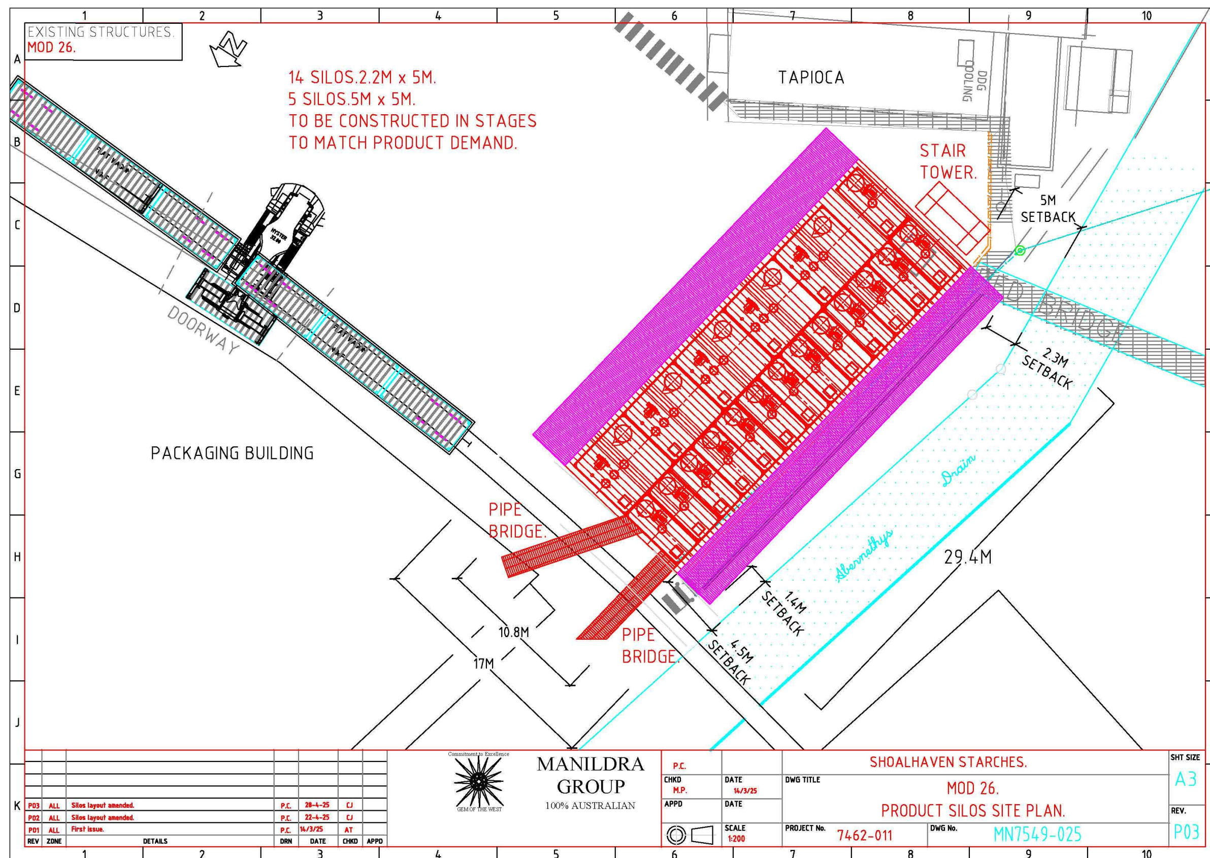
Figure 11 – Layout for the 19 Finished Product Silos
