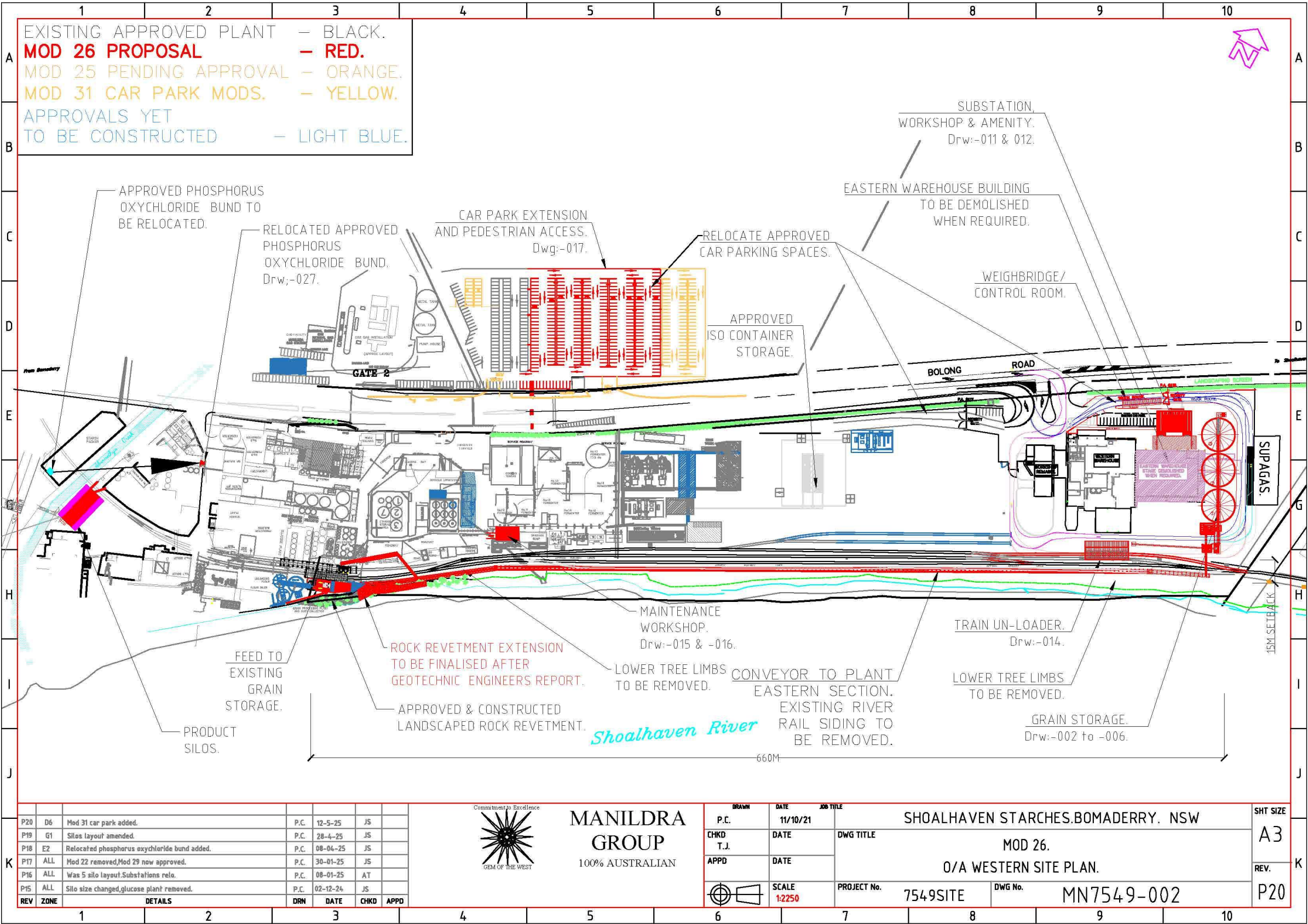
Figure 12 – Proposed Three Wheat Silos and Conveyor
