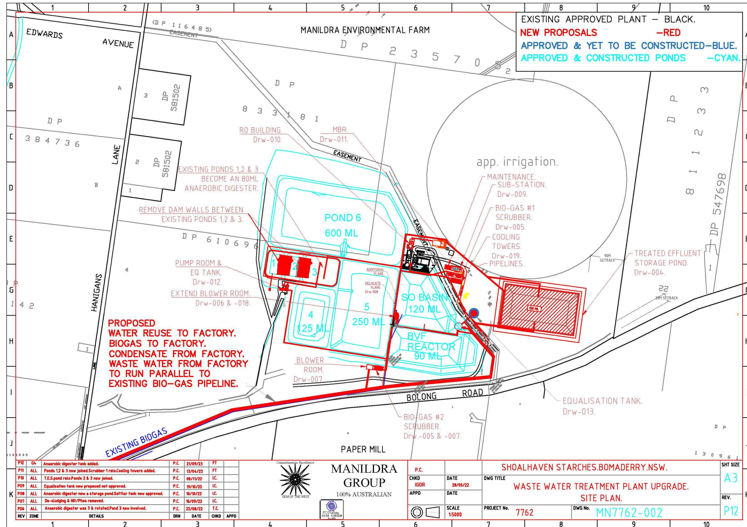
Figure 13 – WWTP Plan Showing Modifications
