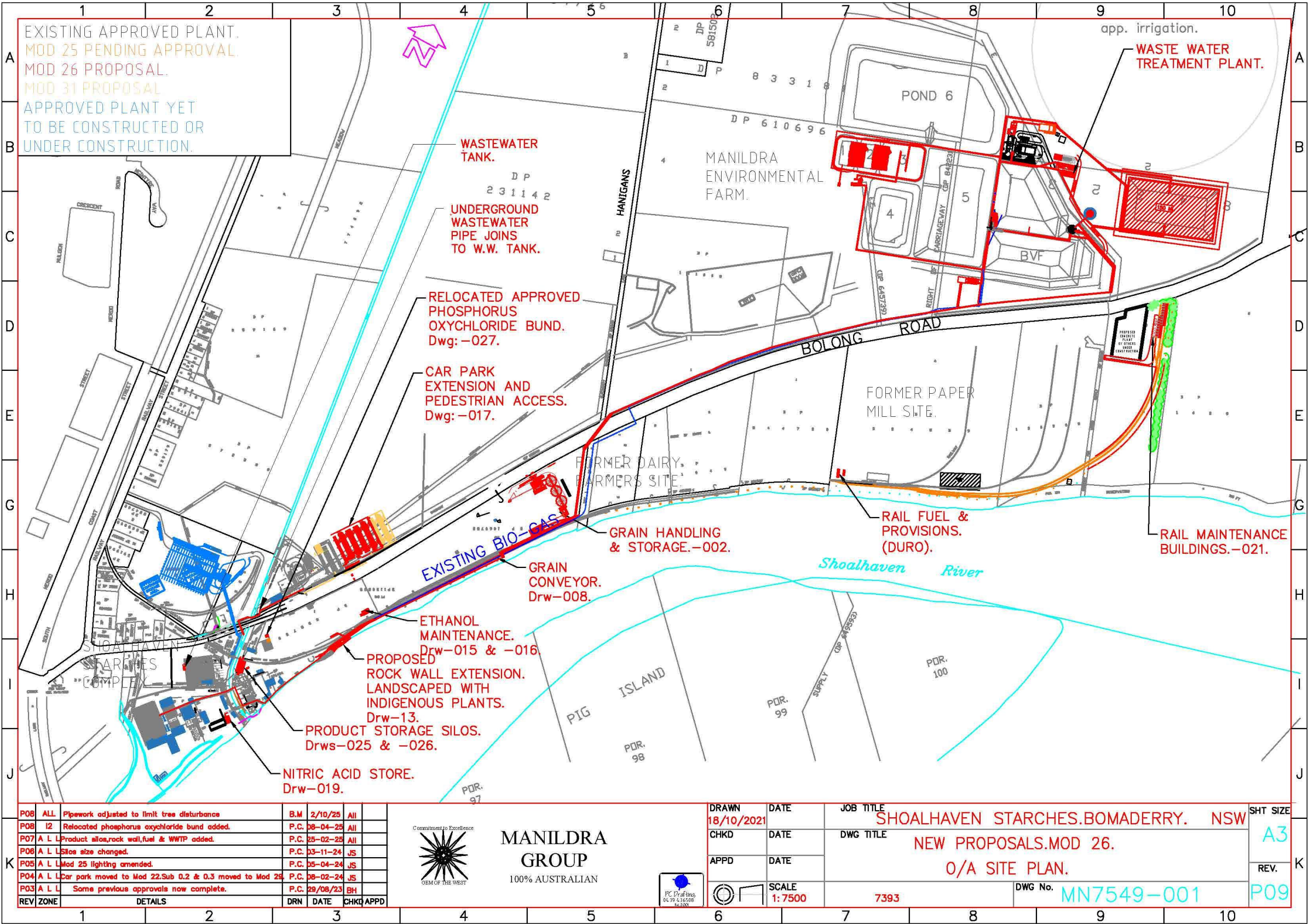
Figure 9 – Location of the Proposed Nitric Acid Tank (plus other MOD26 changes)
