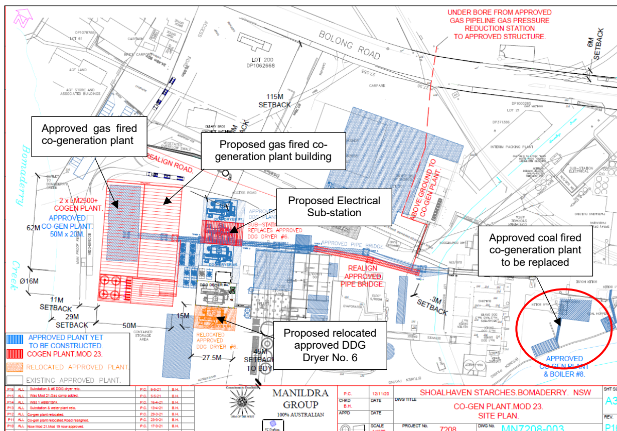
Figure 5: Site Plan showing location of approved and proposed gas fired co-generation plant and location of coal fired co-generation plan which is to be replaced
