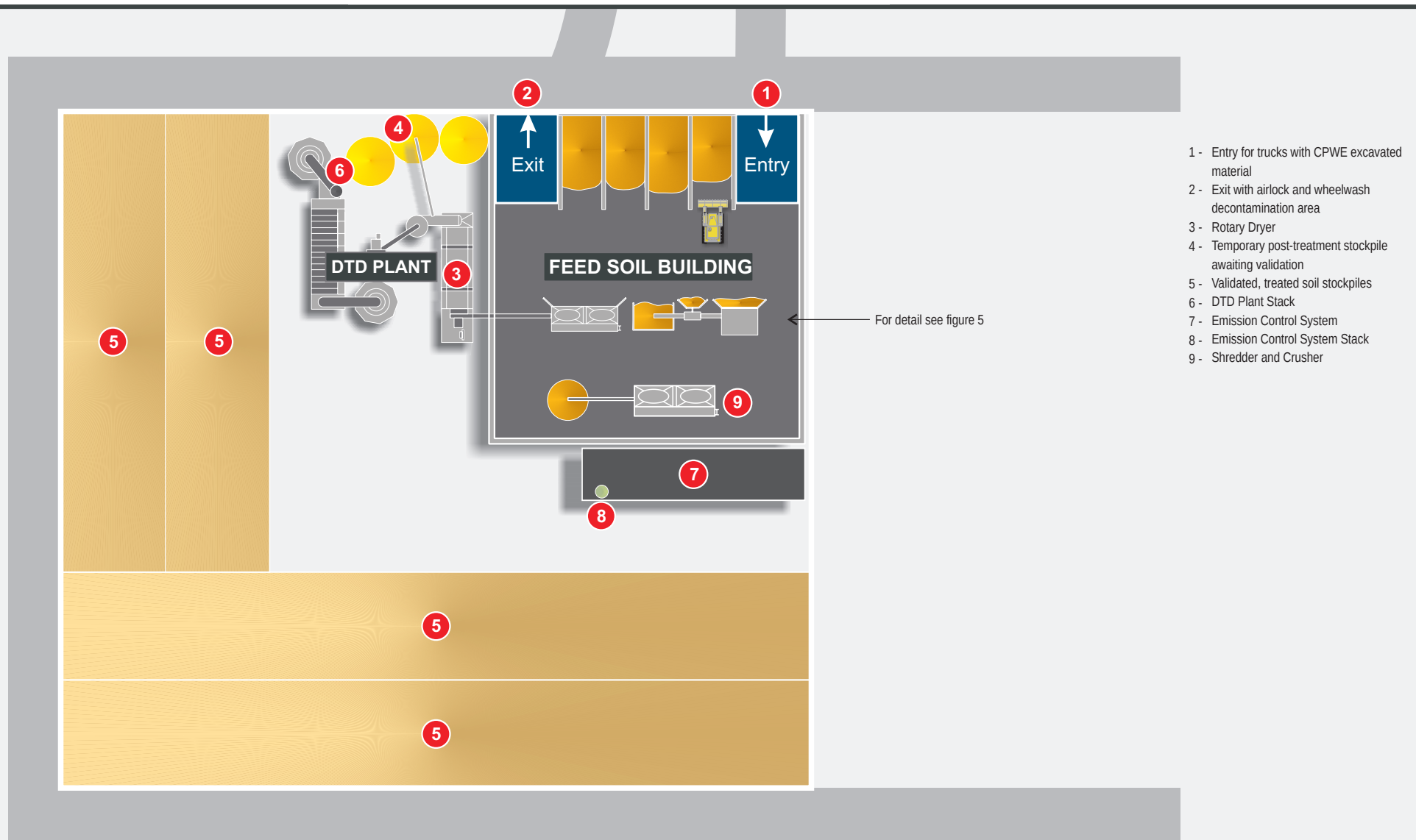
Figure 4 Conceptual Soil Treatment Area Layout Orica Australia Pty Ltd
