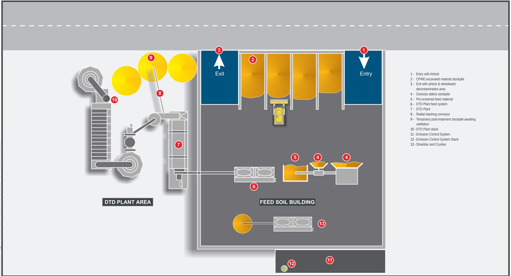
Figure 10 Conceptual Feed Soil Building Layout Orica Australia Pty Ltd Remediation of Car Park Waste Encapsulation Botany Industrial Park Environmental Assessment
