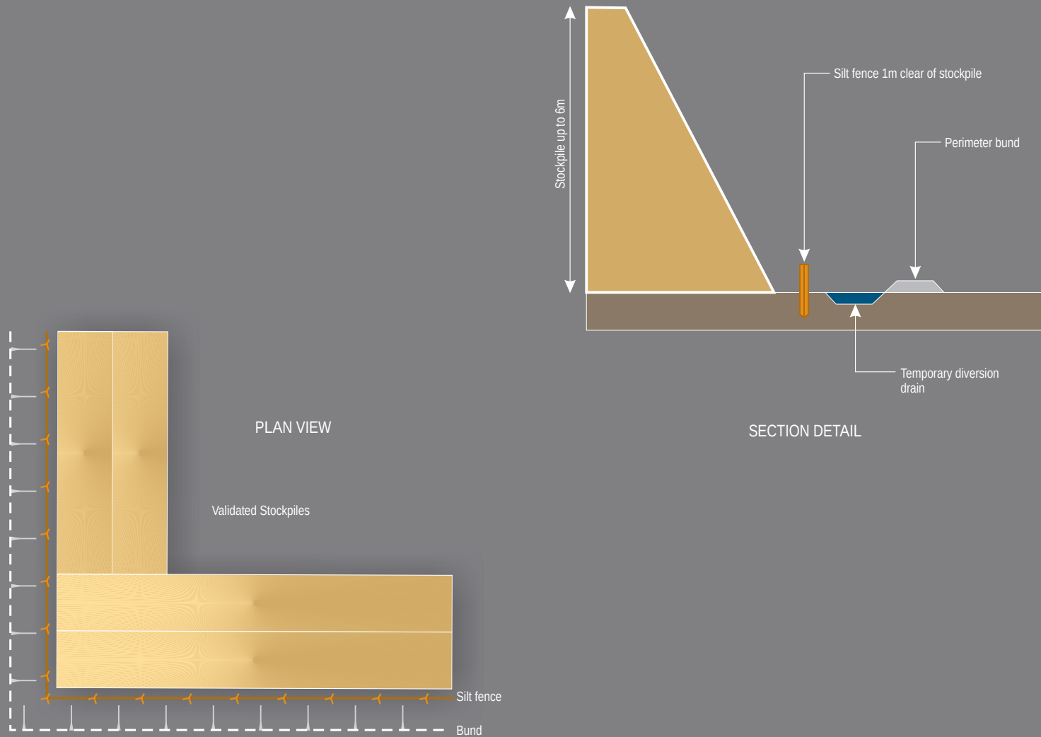
Figure 12 Conceptual Stockpile Management Orica Australia Pty Ltd Remediation of Car Park Waste Encapsulation Botany Industrial Park Environmental Assessment
