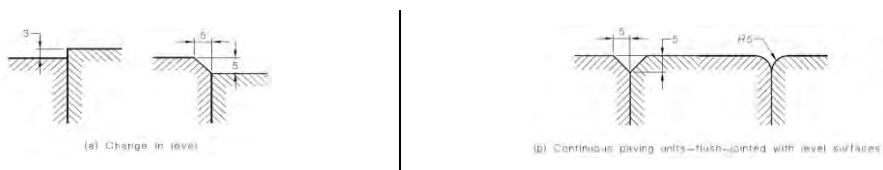
Figure 3: Trip Free Surfaces – Section 7.2 of AS1428.1-2009
