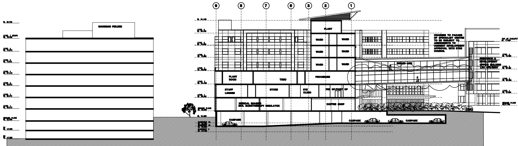
Section 3
