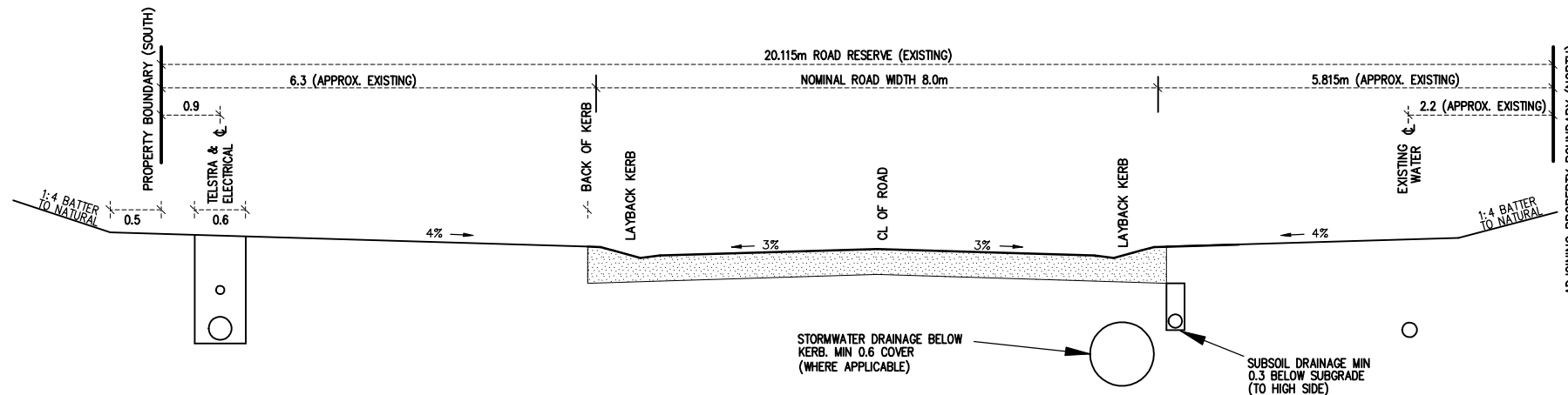
TYPICAL CROSS SECTION AND SERVICE LOCATION "THE BOUNTY" N.T.S.
