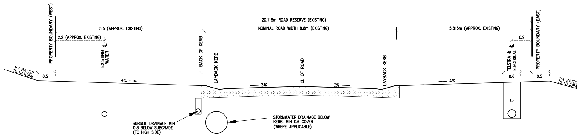
TYPICAL CROSS SECTION AND SERVICE LOCATION "MANYANA DRIVE" N.T.S.
