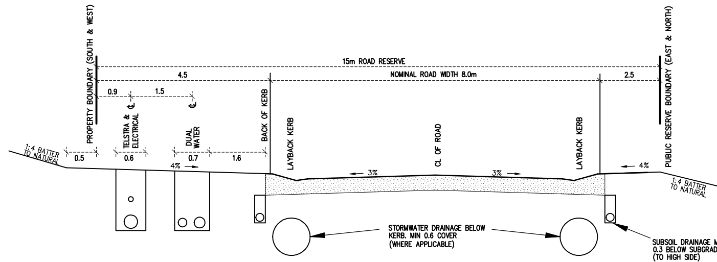
TYPICAL CROSS SECTION AND SERVICE LOCATION "ROAD 1" N.T.S.
