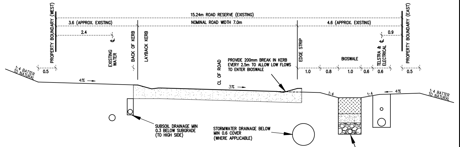
TYPICAL CROSS SECTION AND SERVICE LOCATION "THE BARRETTE" N.T.S.
