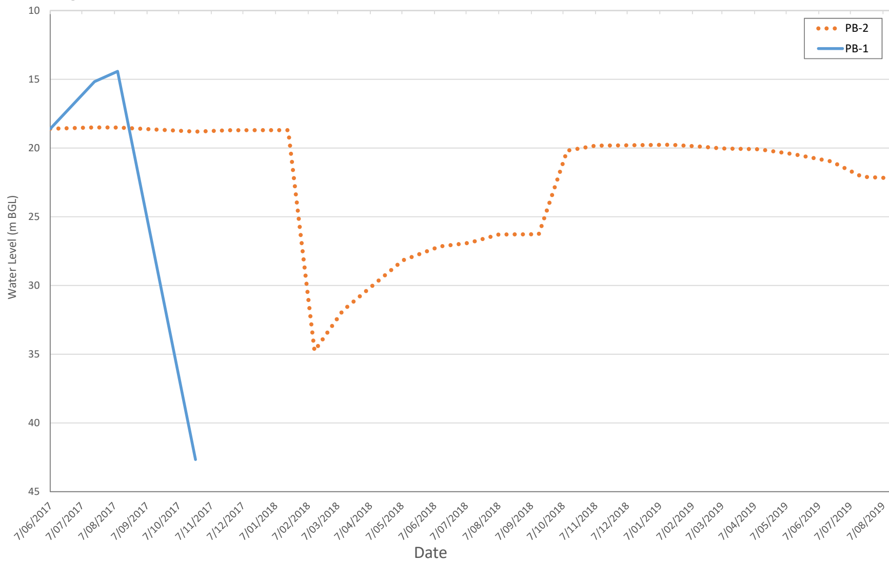
Figure HG-1: Lot 198 Wells (PB1 & PB-2): Groundwater Level Measurements (2017 to 2019)
