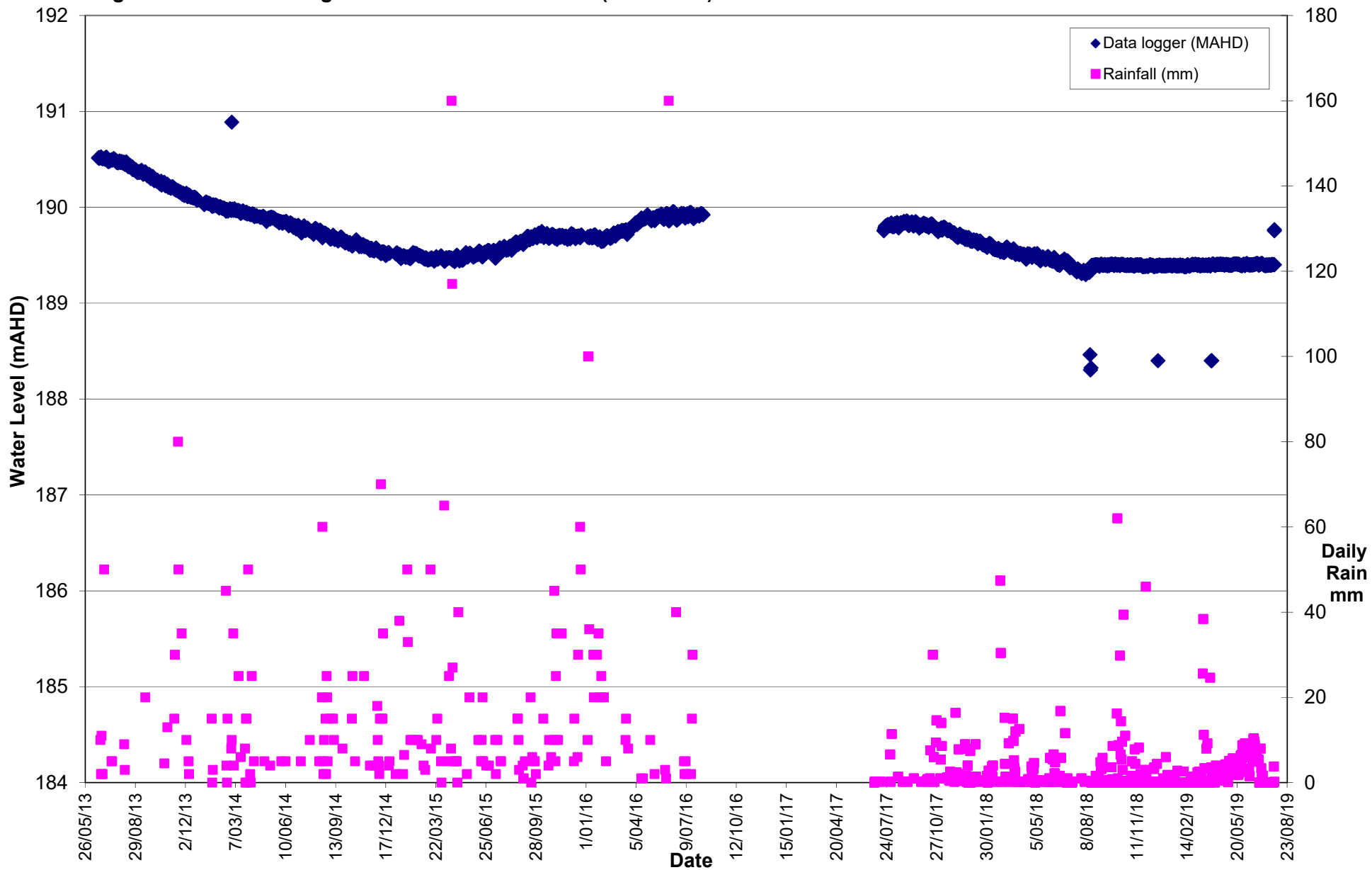
Figure HG-5: Monitoring Data Bore PFL2HitchMW1 (2013-2019)
