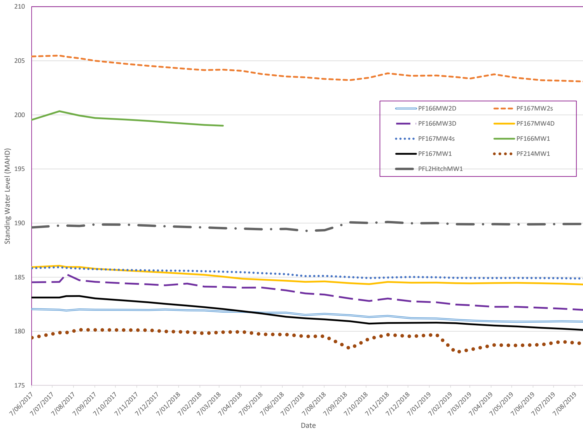
Figure HG-8: Hitchcock Road, Monthly Groundwater Levels (2017-2019)
