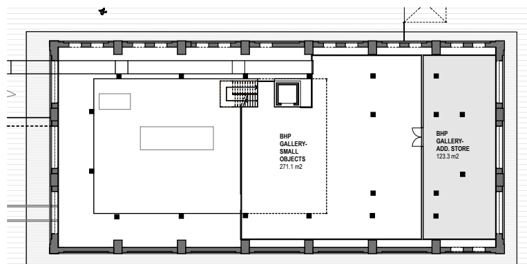
2 Lower Mezzanine Level 1:500
