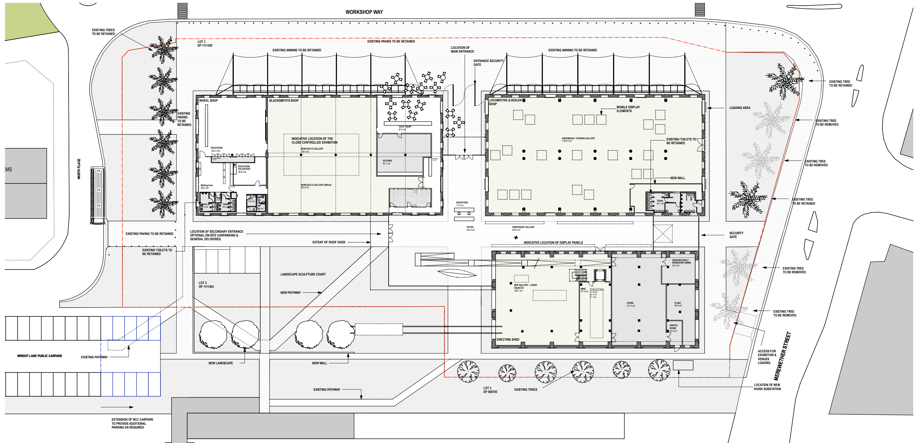
1 Ground Level 1:500
