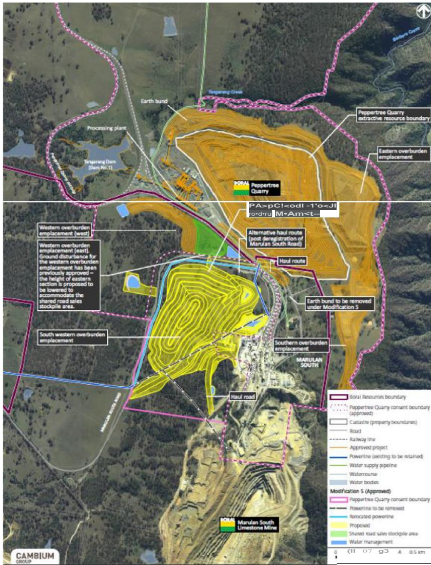
Figure 1.1: Site Layout
