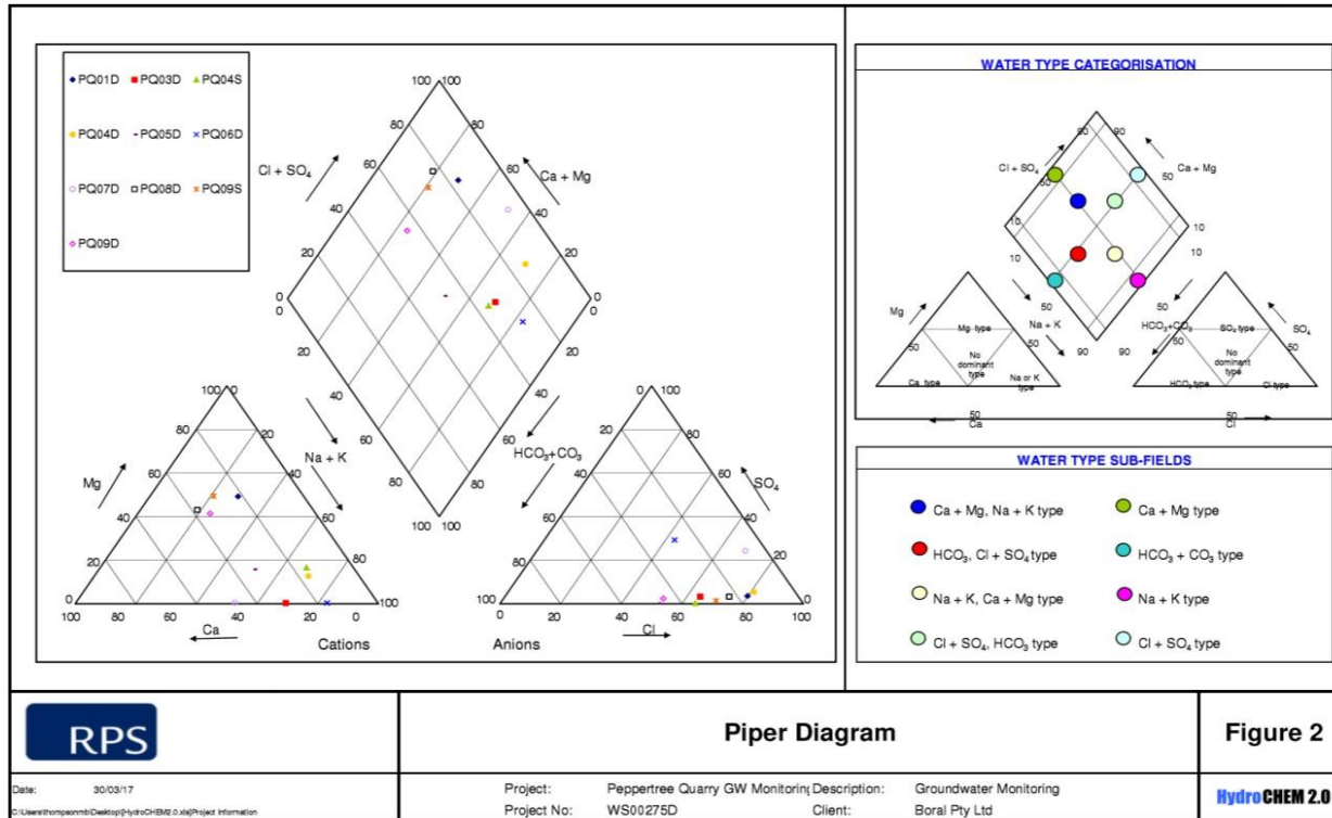
Figure 4.5 Piper Diagram of Results
