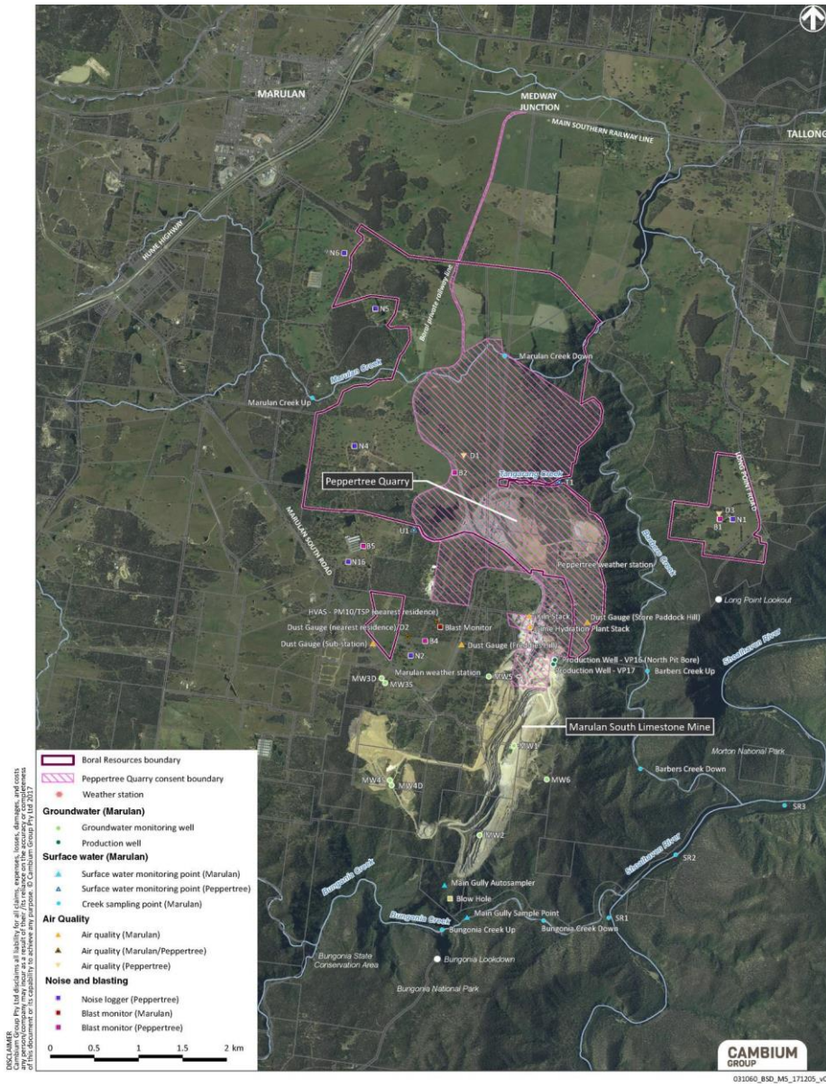
Figure 4.1: Surface Water and Groundwater Monitoring Sites
