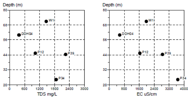
Figure 4.2: TDS and EC vs Depth
