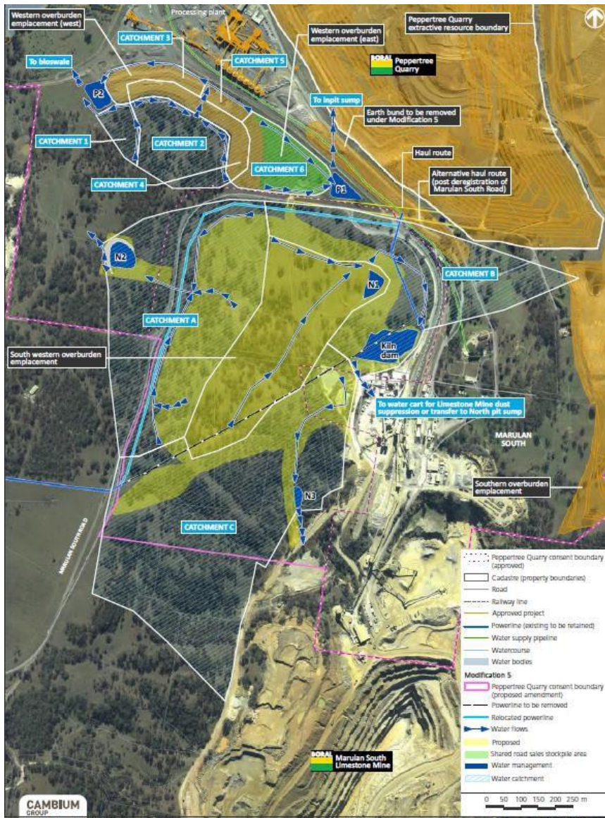
Figure 5.4: South Western Overburden Emplacement Surface Water Management
