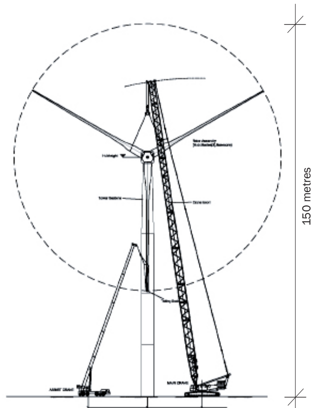
Section showing typical erection of Rotor assembly
