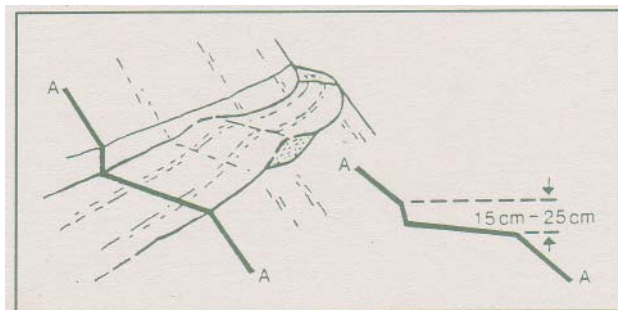
Figure 1: Outfall surfacing of the road should be used instead of infalling.
