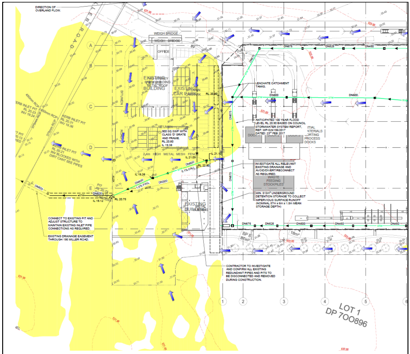
Figure 2 – Stormwater Drainage Plan (Drawing DA-STW-101 of Appendix N of EA)
