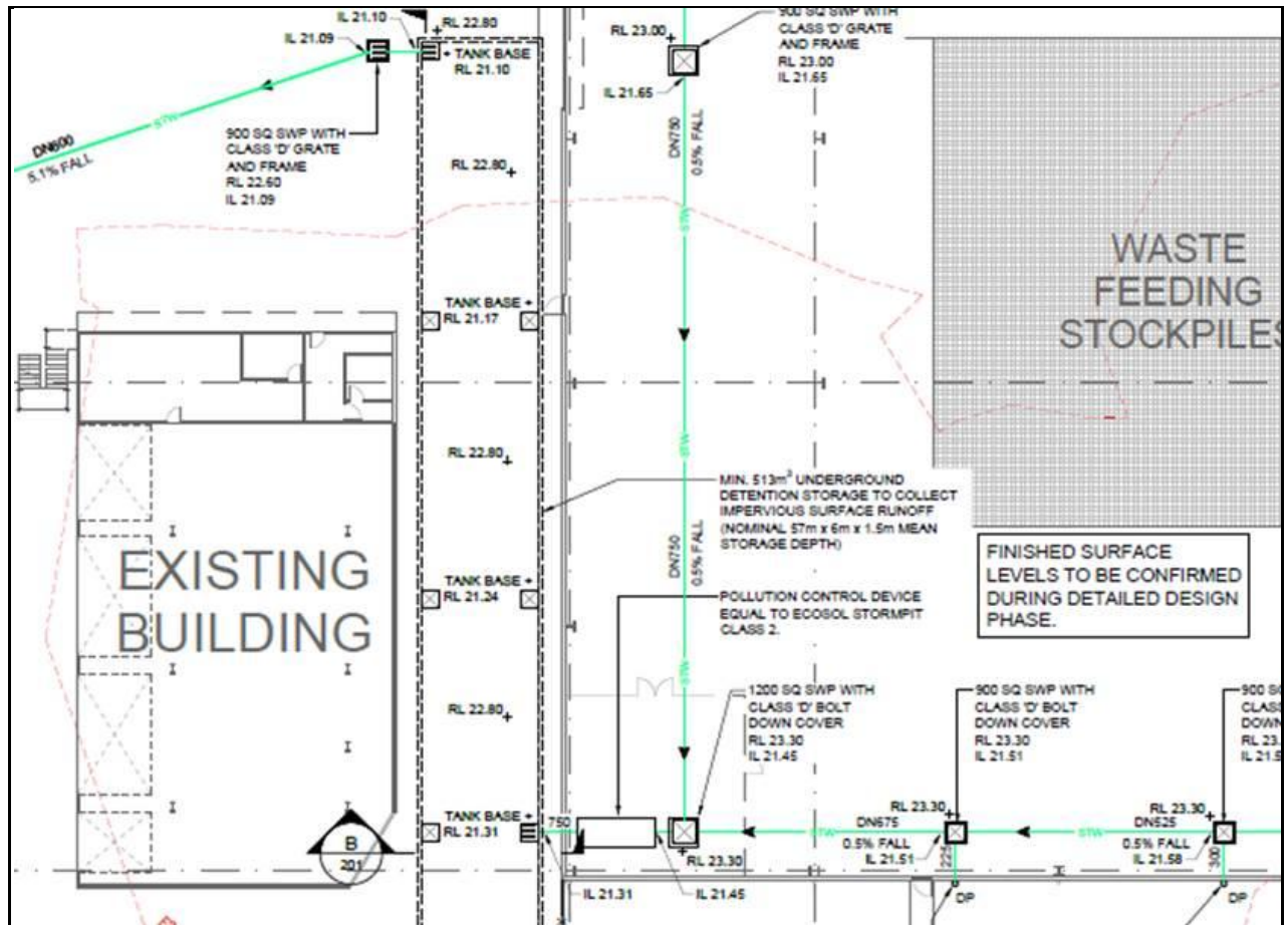
Figure 1 – Pollution control device upstream of the On Site Detention (OSD) tank as per drawing DA-STW-104 of Appendix J of EA.
