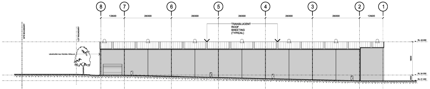
Figure 3.1.10-Northern Elevation
