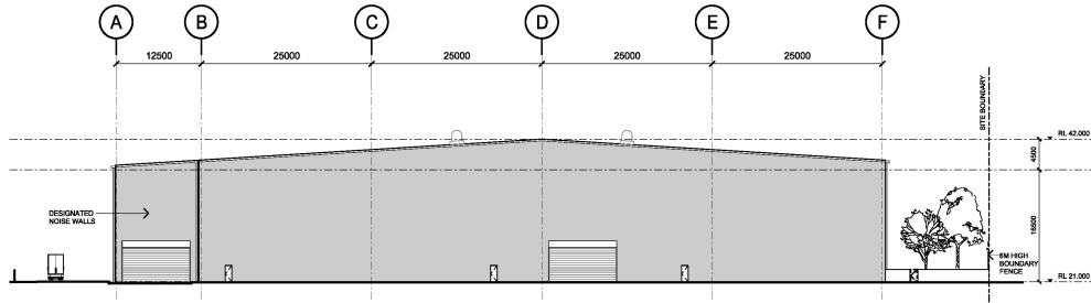
Figure 3.1.8 - Western Elevation
