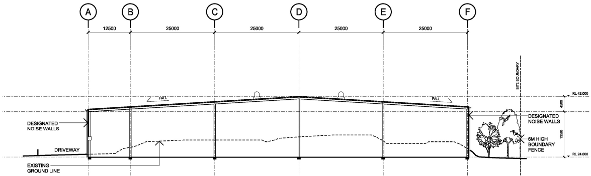
Figure 3.1.5 – Section through new building
