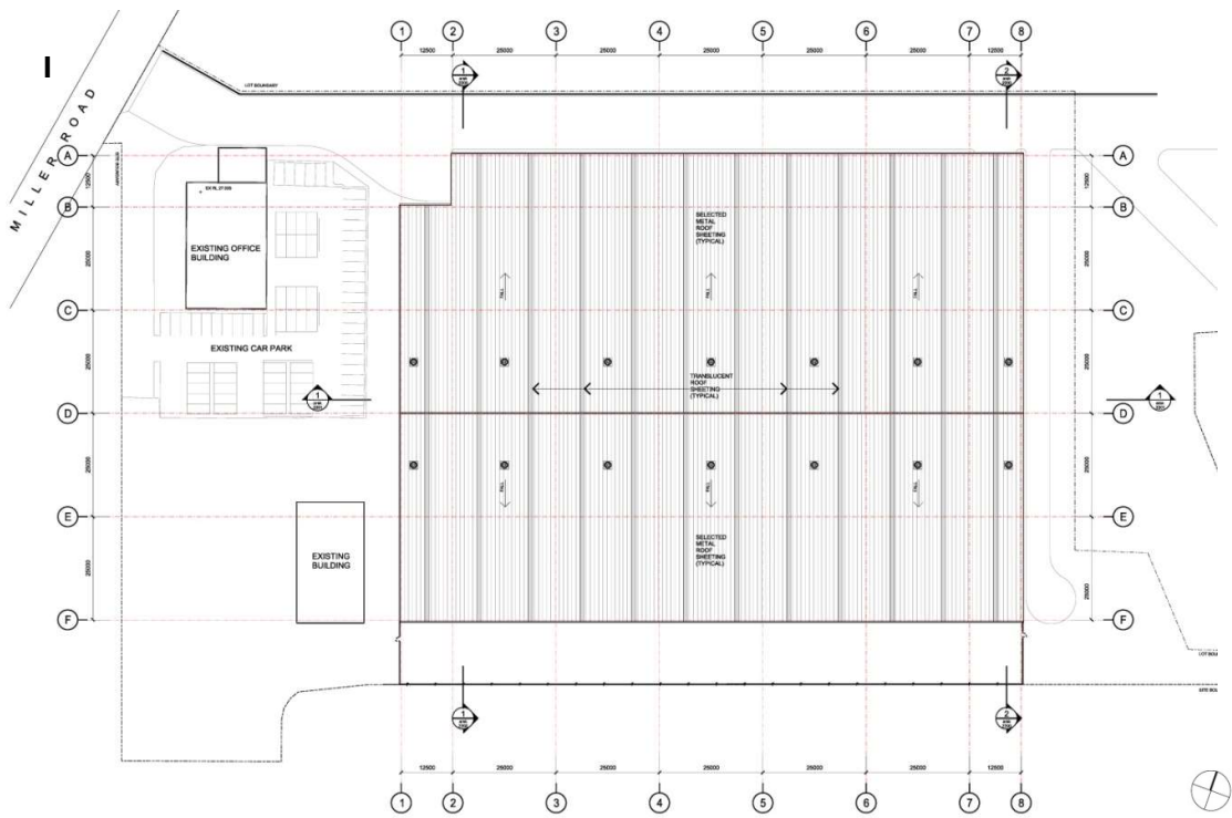
Fig 3.1.2- Roof Plan
