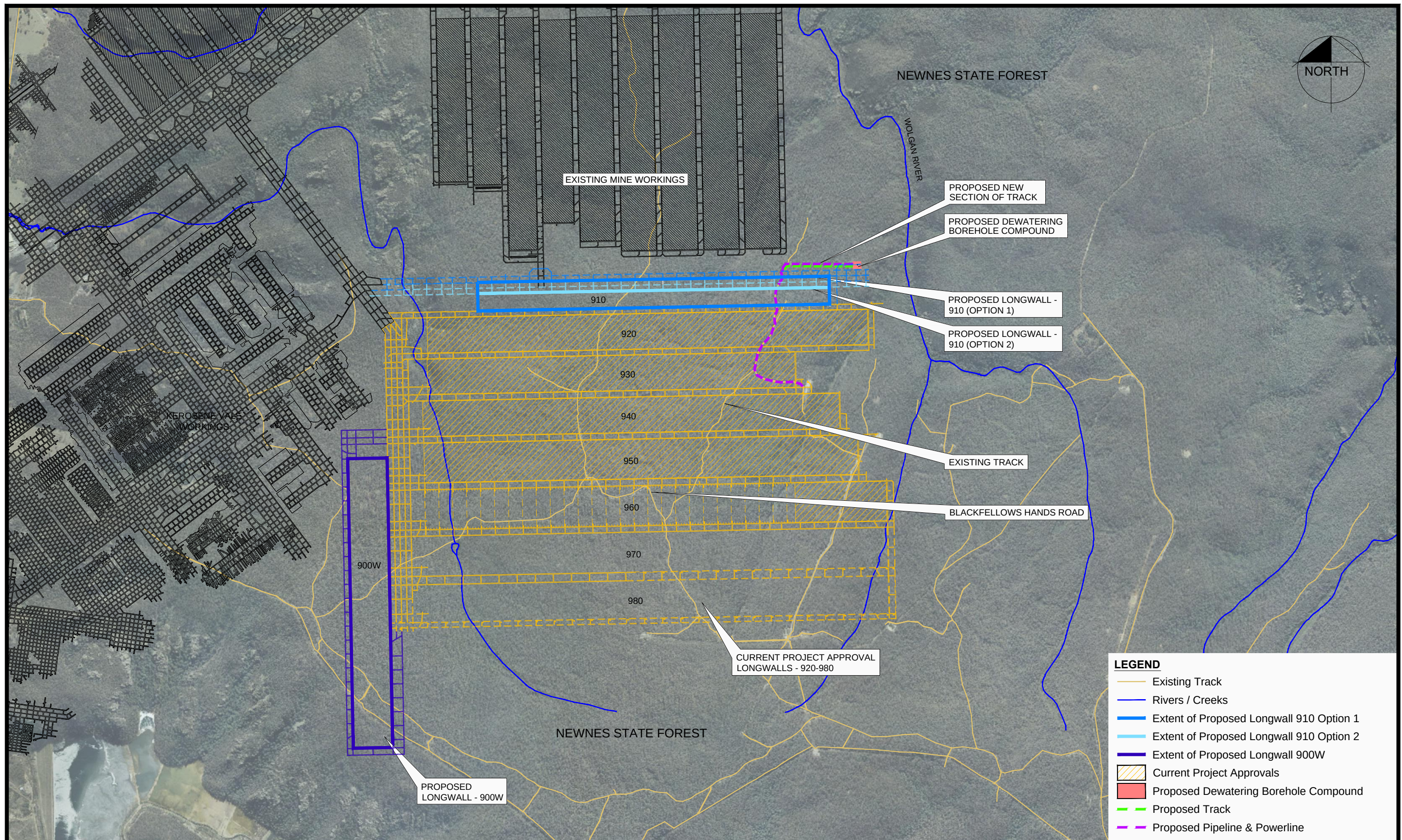
PROPOSED LONGWALLS, DEWATERING BORE & ASSOCIATED INFRASTRUCTURE FIGURE 3.2
