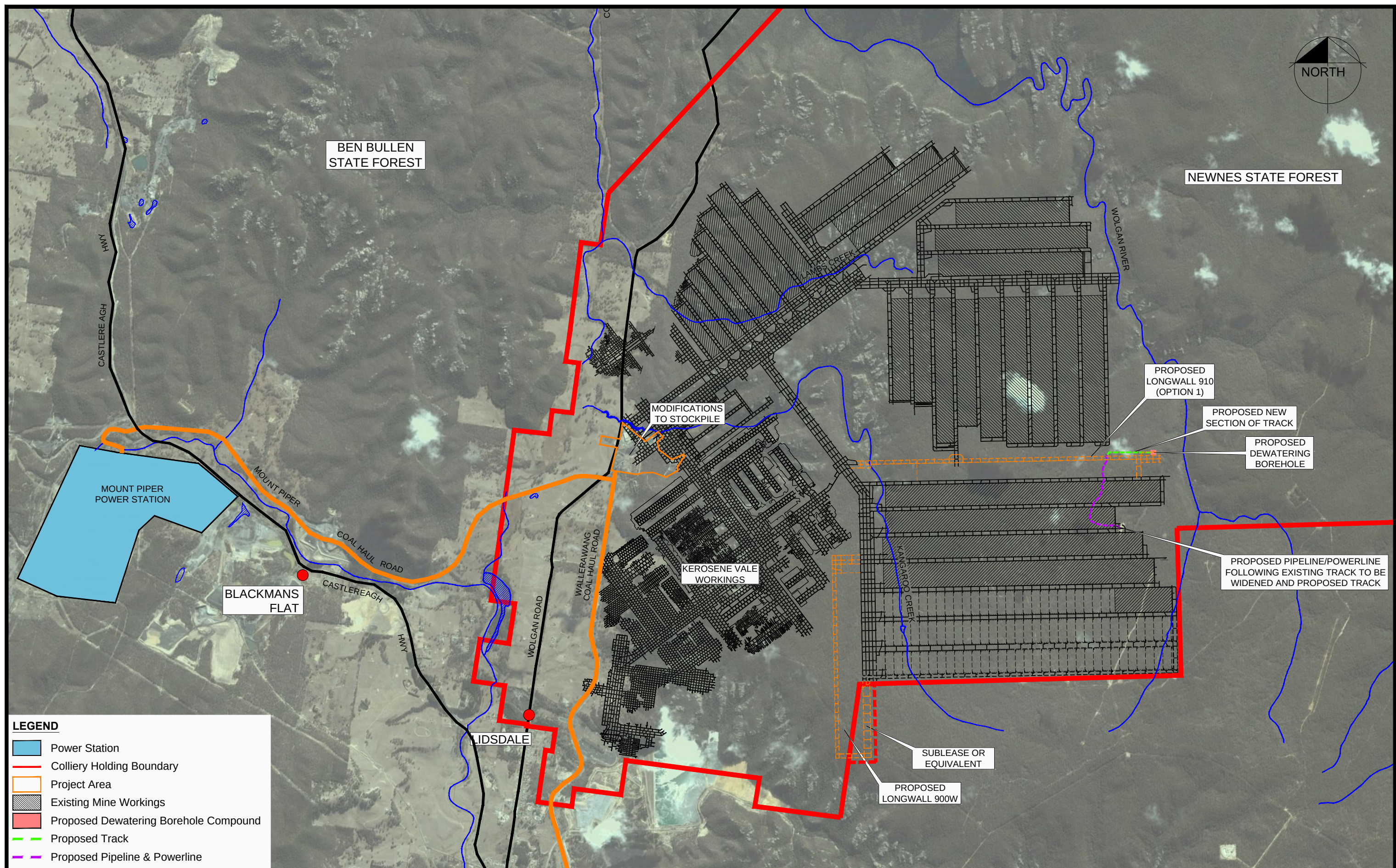
EXISTING MINE WITH PROPOSED MODIFICATIONS FIGURE 3.1
