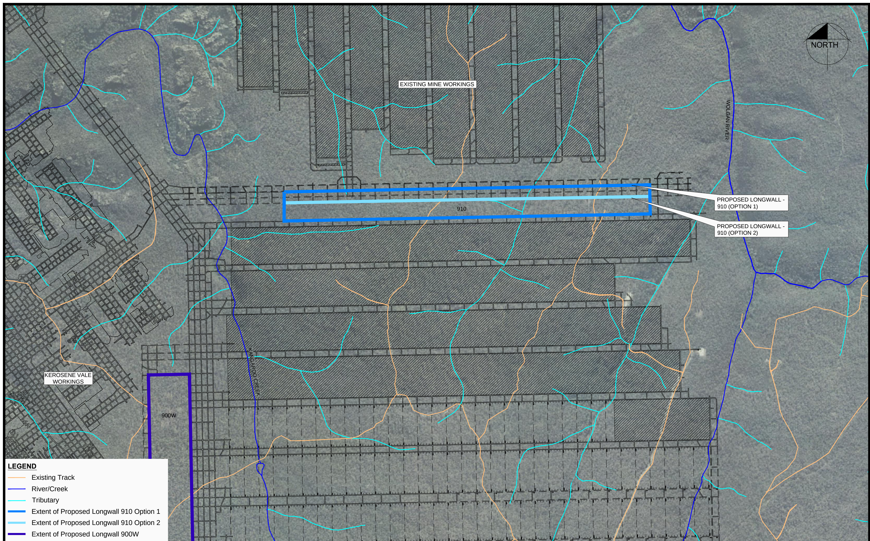
PROPOSED LONGWALL 910 FIGURE 3.3
