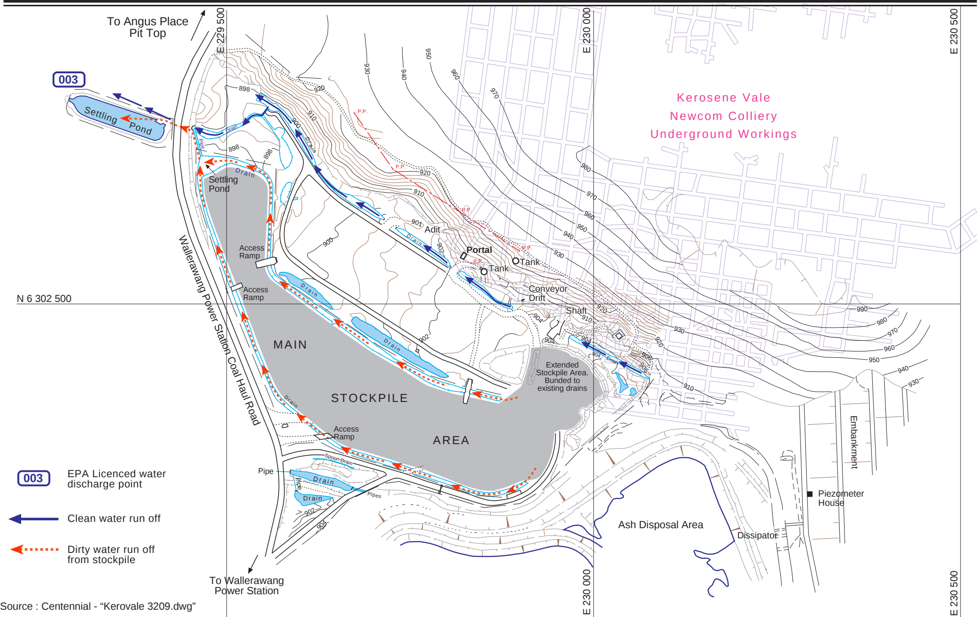
FIGURE 4 Kerosene Vale Colliery - Site Plan
