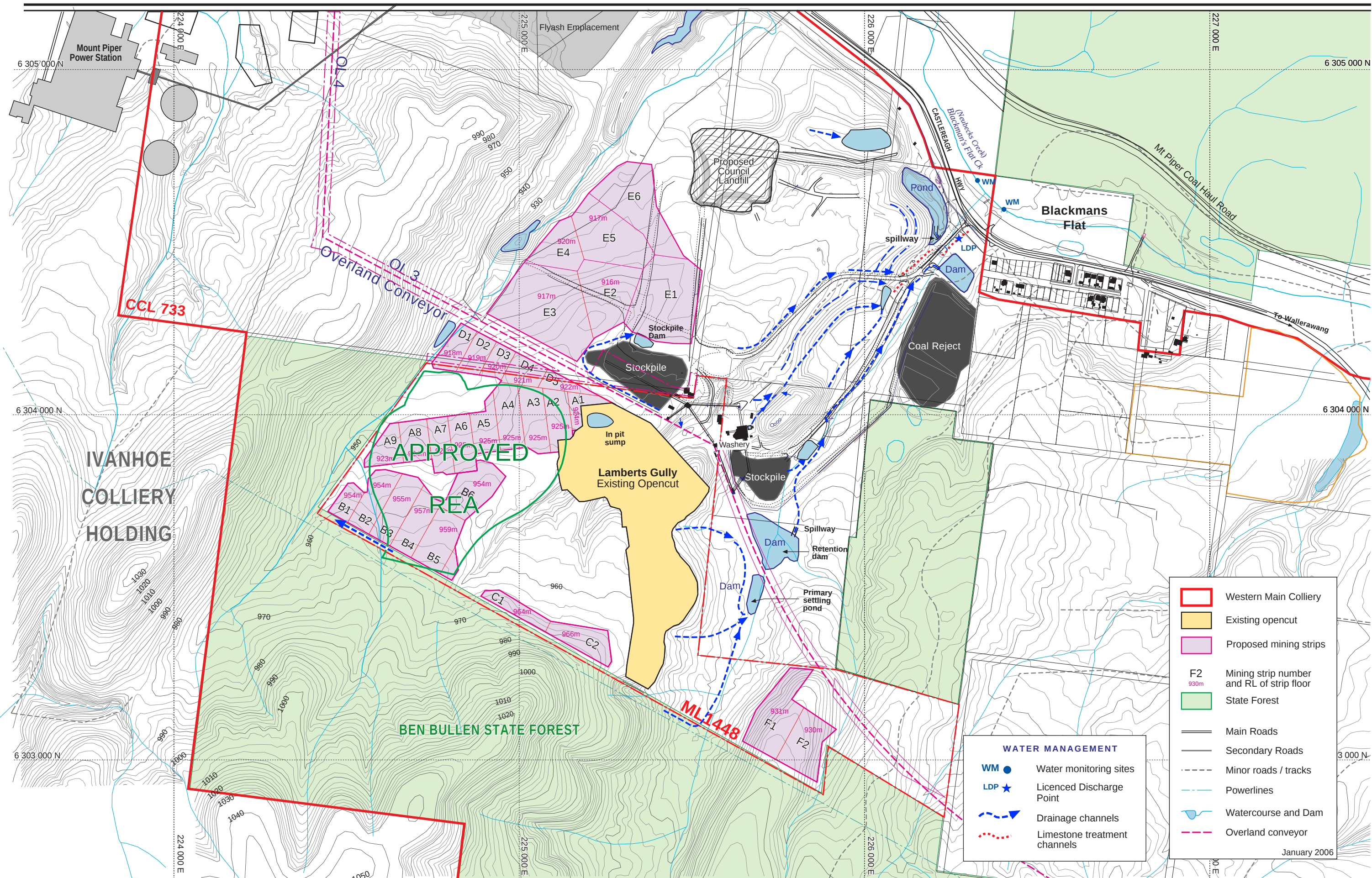
FIGURE 5 Lamberts Gully - Water Management Plan
