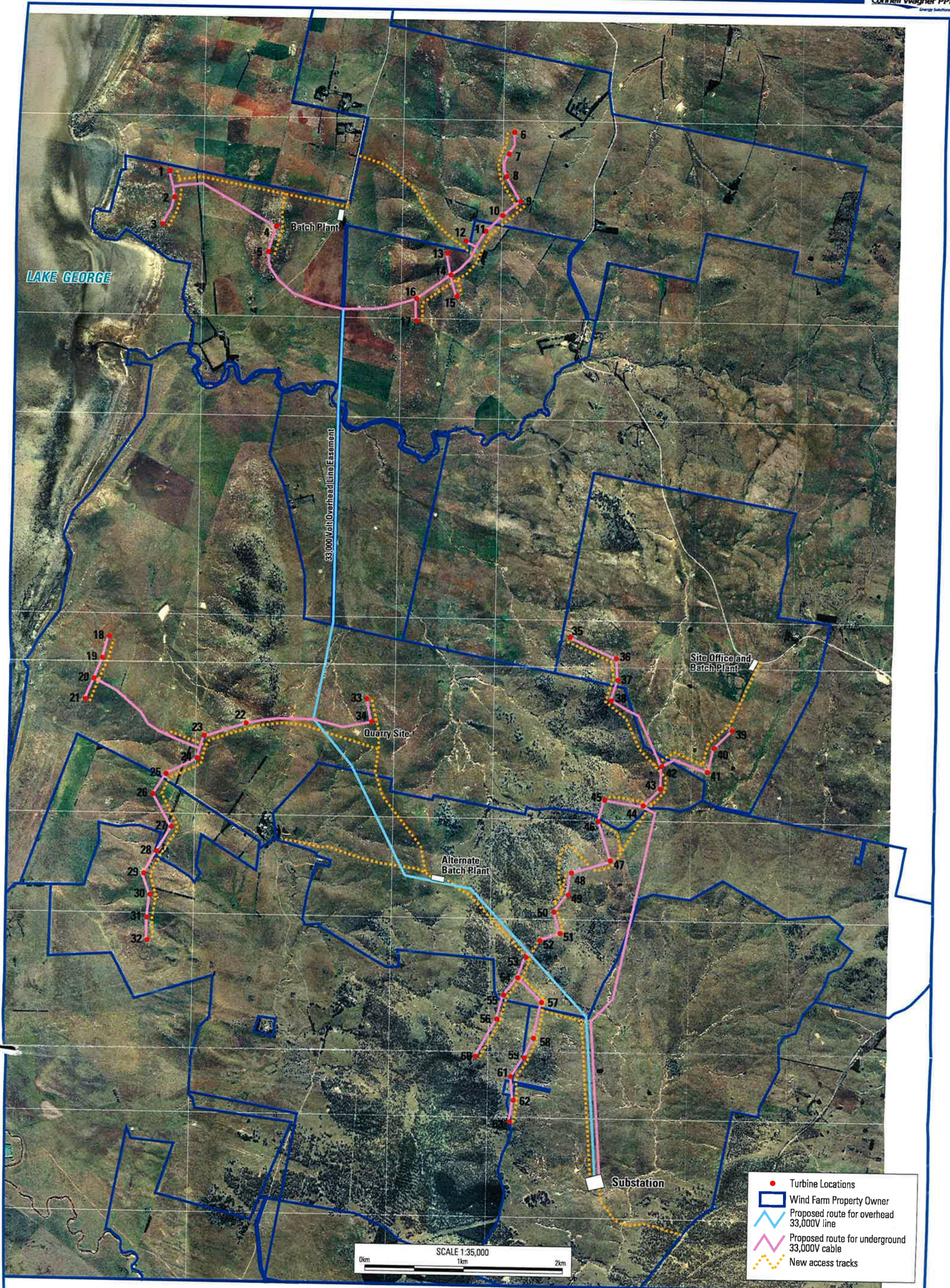
FIGURE 1.6 AERIAL PHOTO WITH WIND FARM LAYOUT
