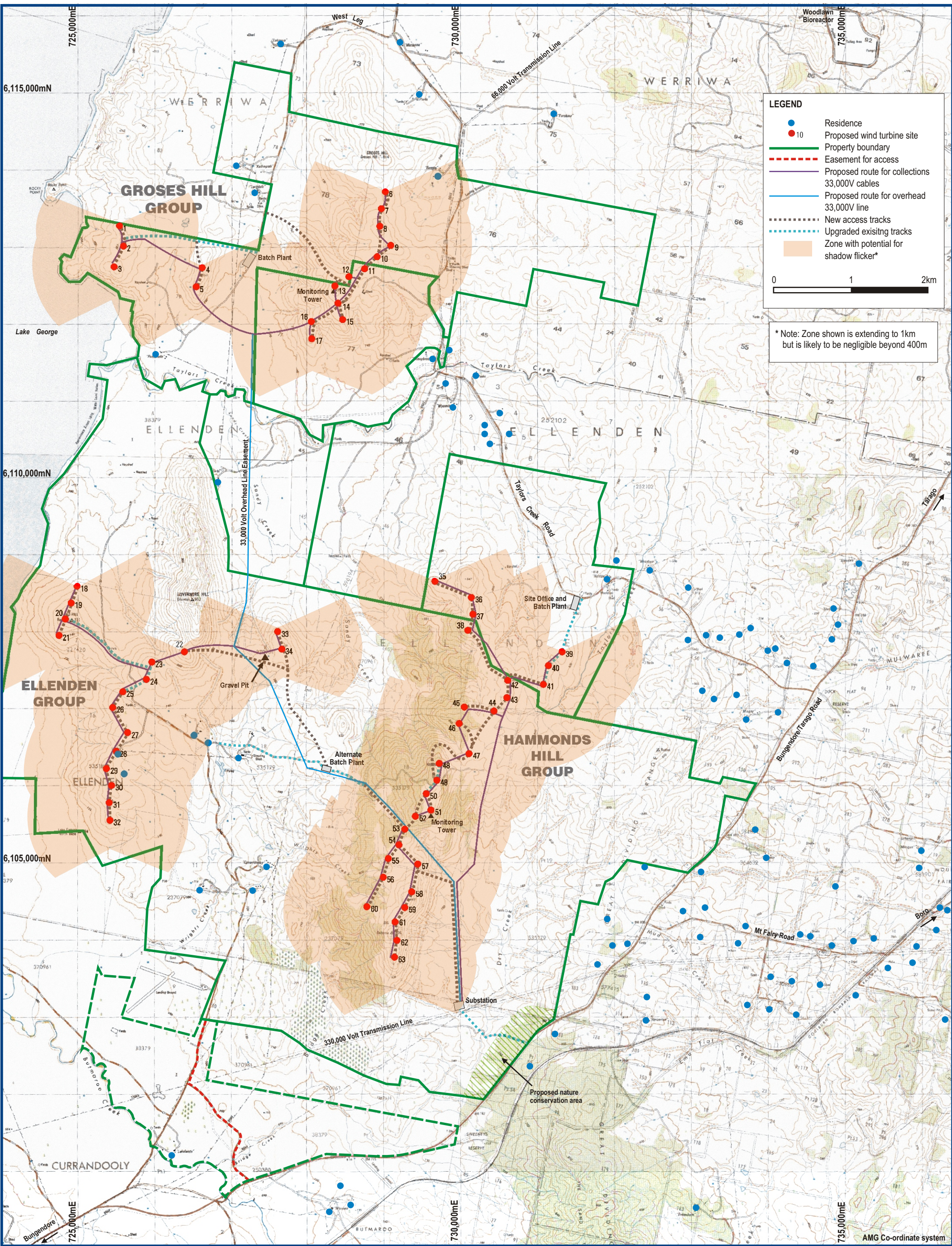
FIGURE 6 POTENTIAL SHADOW FLICKER ZONE
