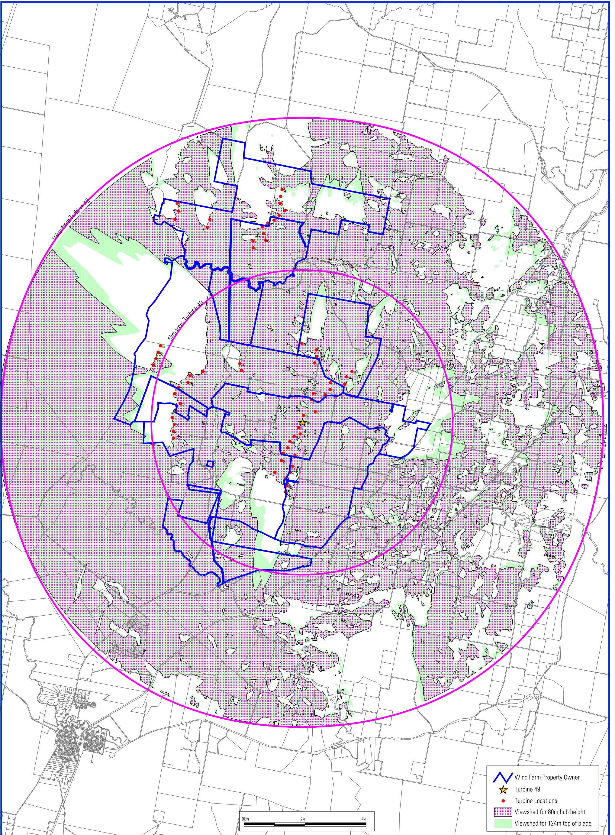
FIGURE 9 TURBINE 49 COMPARISON OF VIEWSHED FOR 80M AND 124M HEIGHTS
