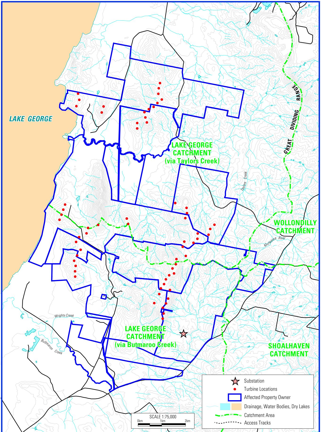
FIGURE 5.7 SITE DRAINAGE MAP, CREEKS AND CATCHMENTS
