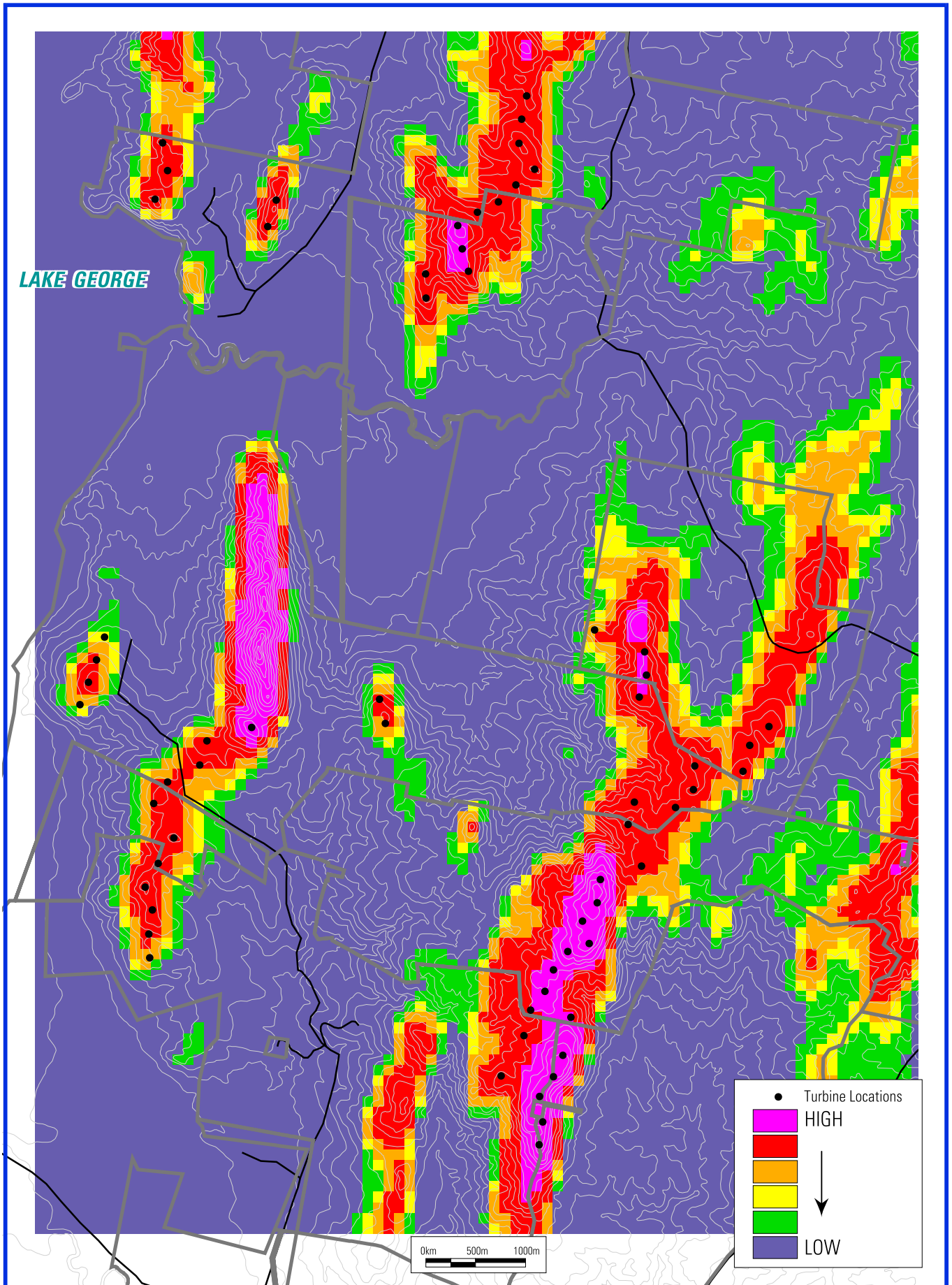
FIGURE 5.3 WIND ENERGY
