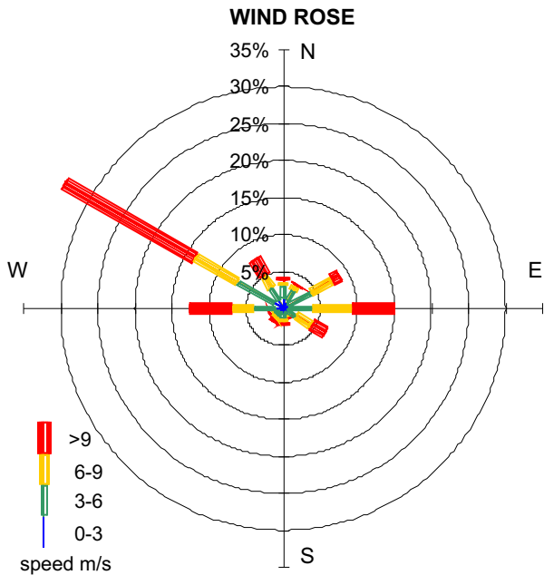
Wind Rose Data for 65m Level
