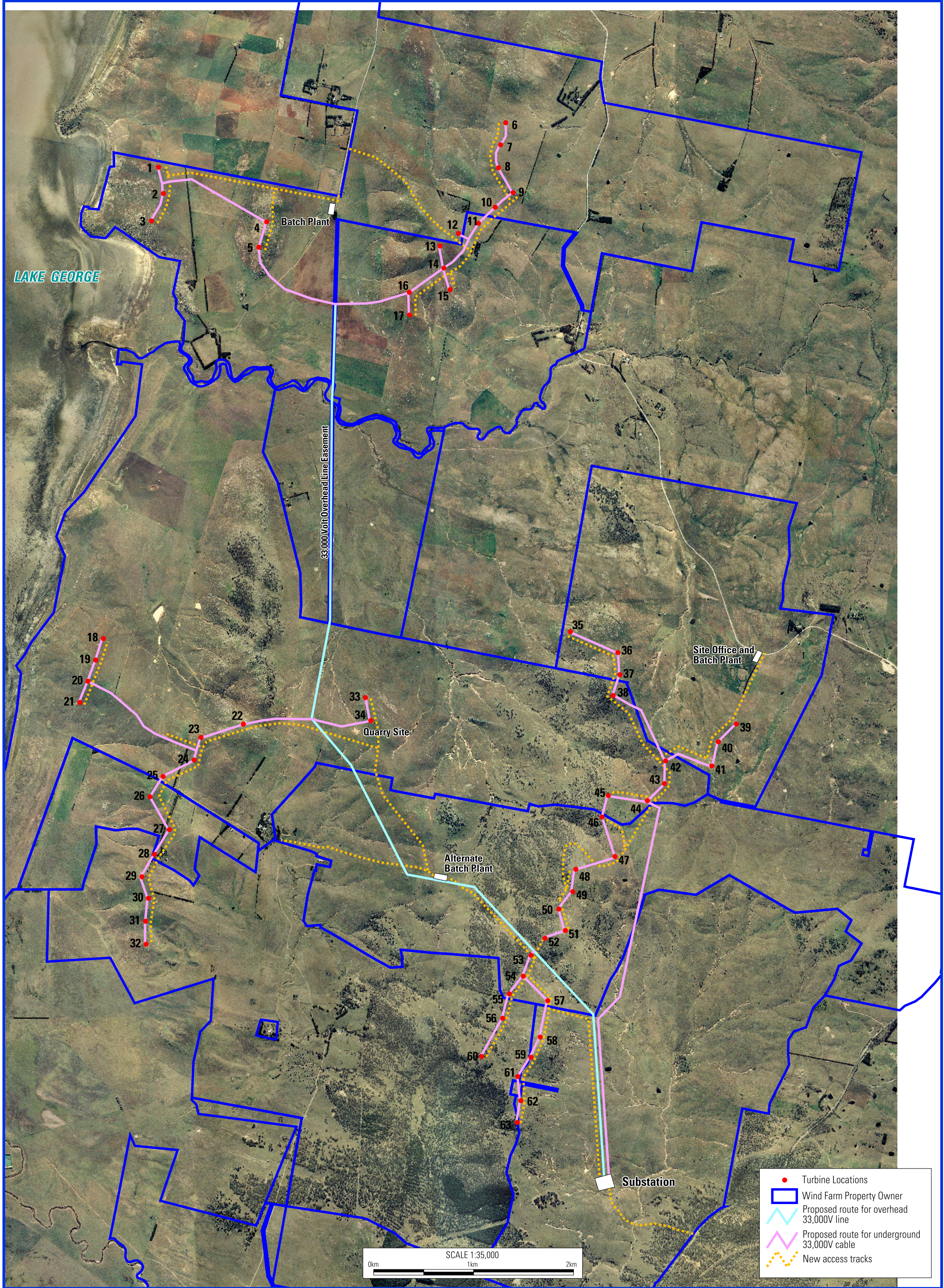
FIGURE ES-2 AERIAL PHOTO WITH WIND FARM LAYOUT
