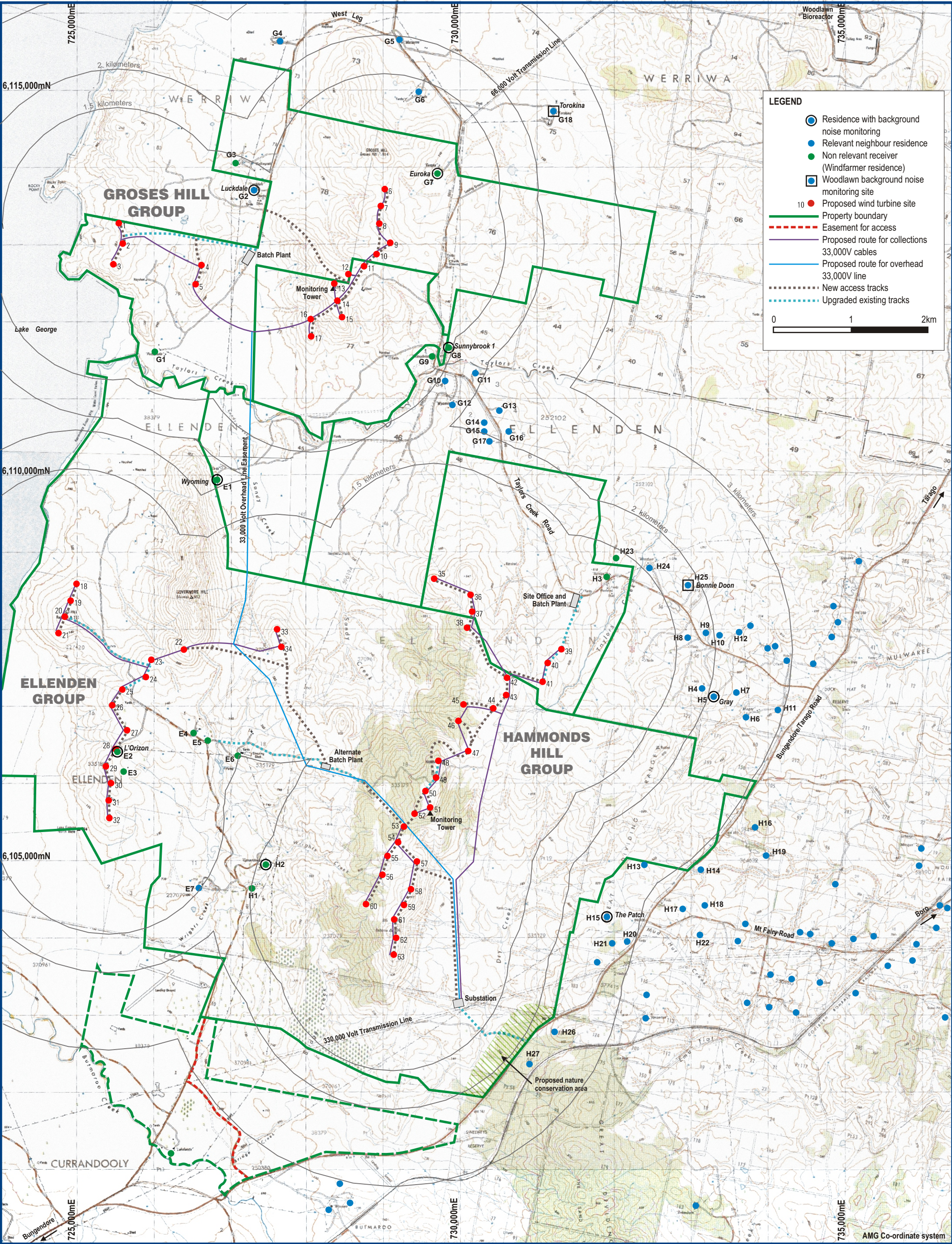
FIGURE 10.1 LOCATION OF RESIDENCES AND BACKGROUND NOISE MONITORING SITES
