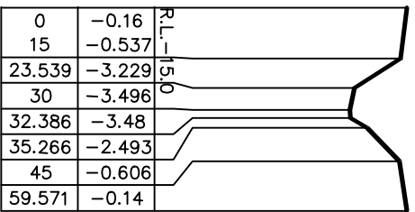
Cross Section.No.7 LOOKING DOWNSTREAM
