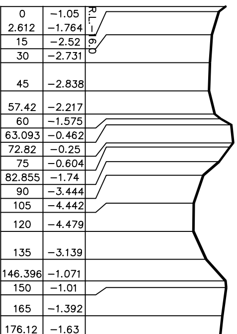
Cross Section.No.10 STONECUT CHANNEL
