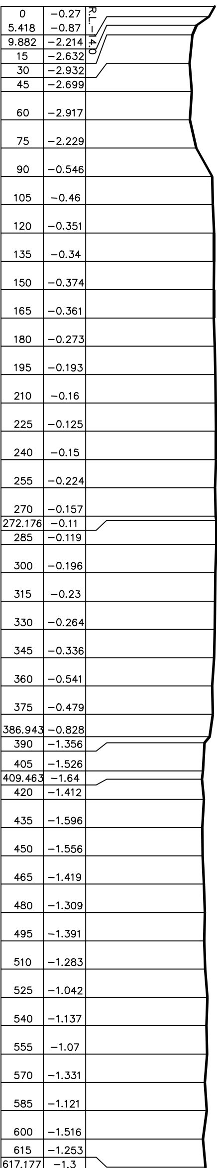
Cross Section.No.20 LOOKING DOWNSTREAM
