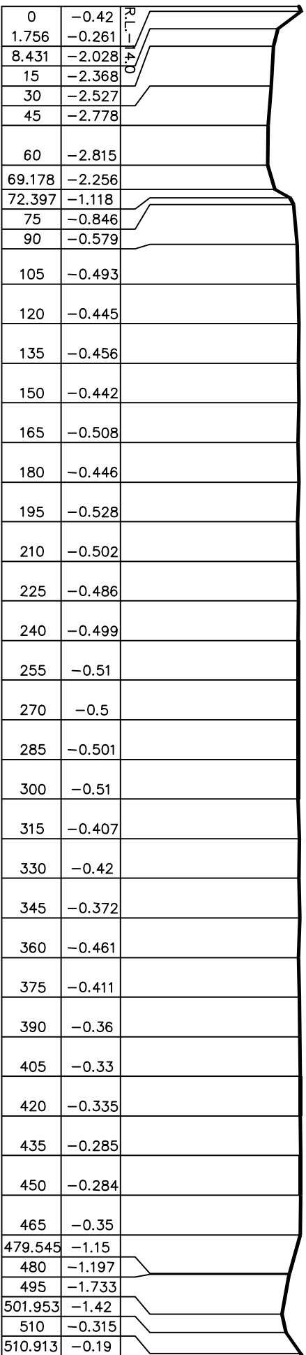
Cross Section.No.17 LOOKING DOWNSTREAM
