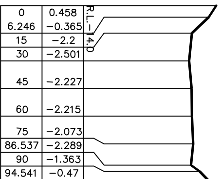
Cross Section.No.26 LOOKING DOWNSTREAM
