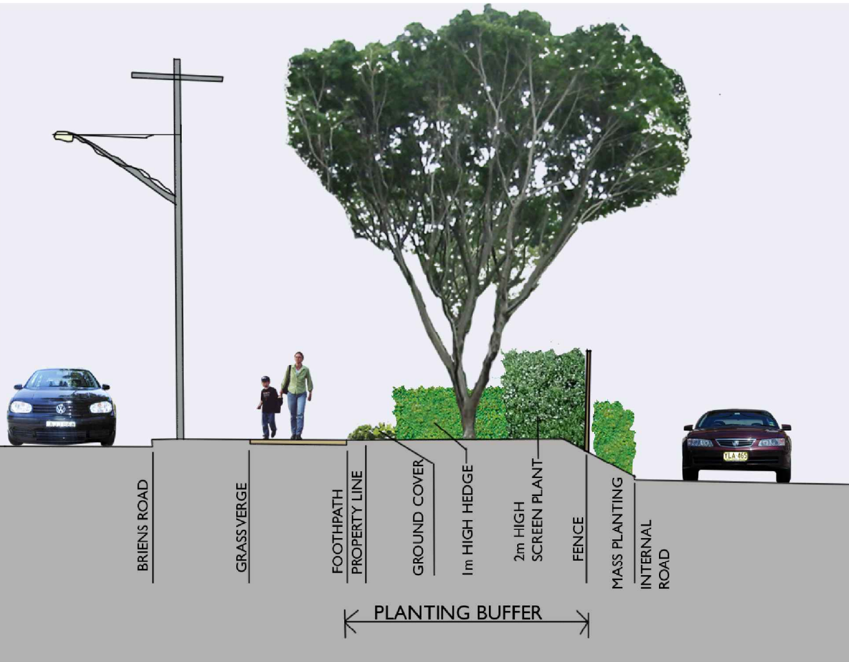
Typical Section
