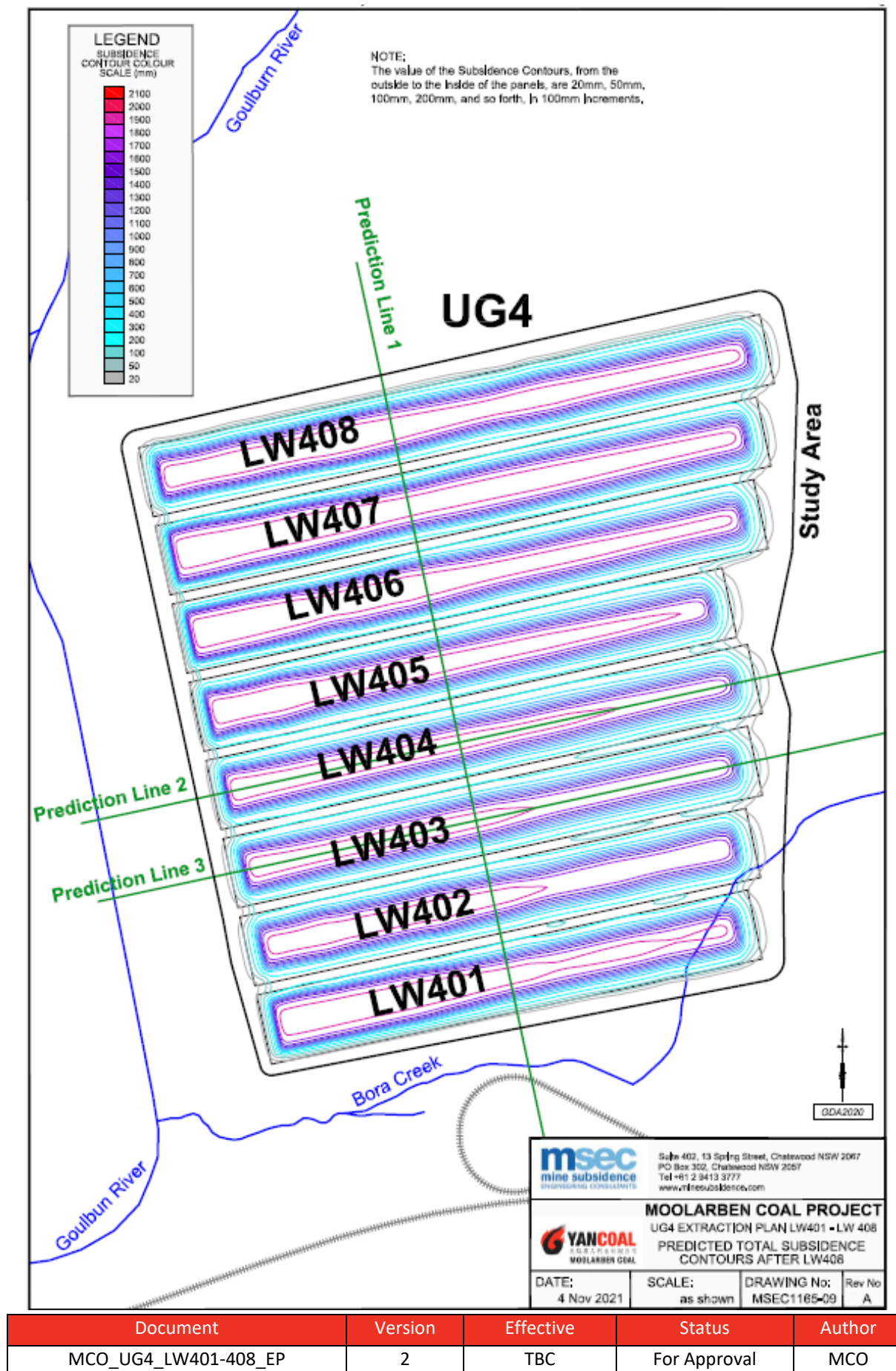
Figure 7: Predicted Subsidence after Longwalls LW401 - 408
