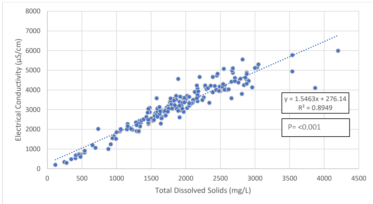
Chart 6. Electrical conductivity (µS/cm) and total dissolved solids (mg/L) correlation in Goulburn River surface water monitoring site SW08.
