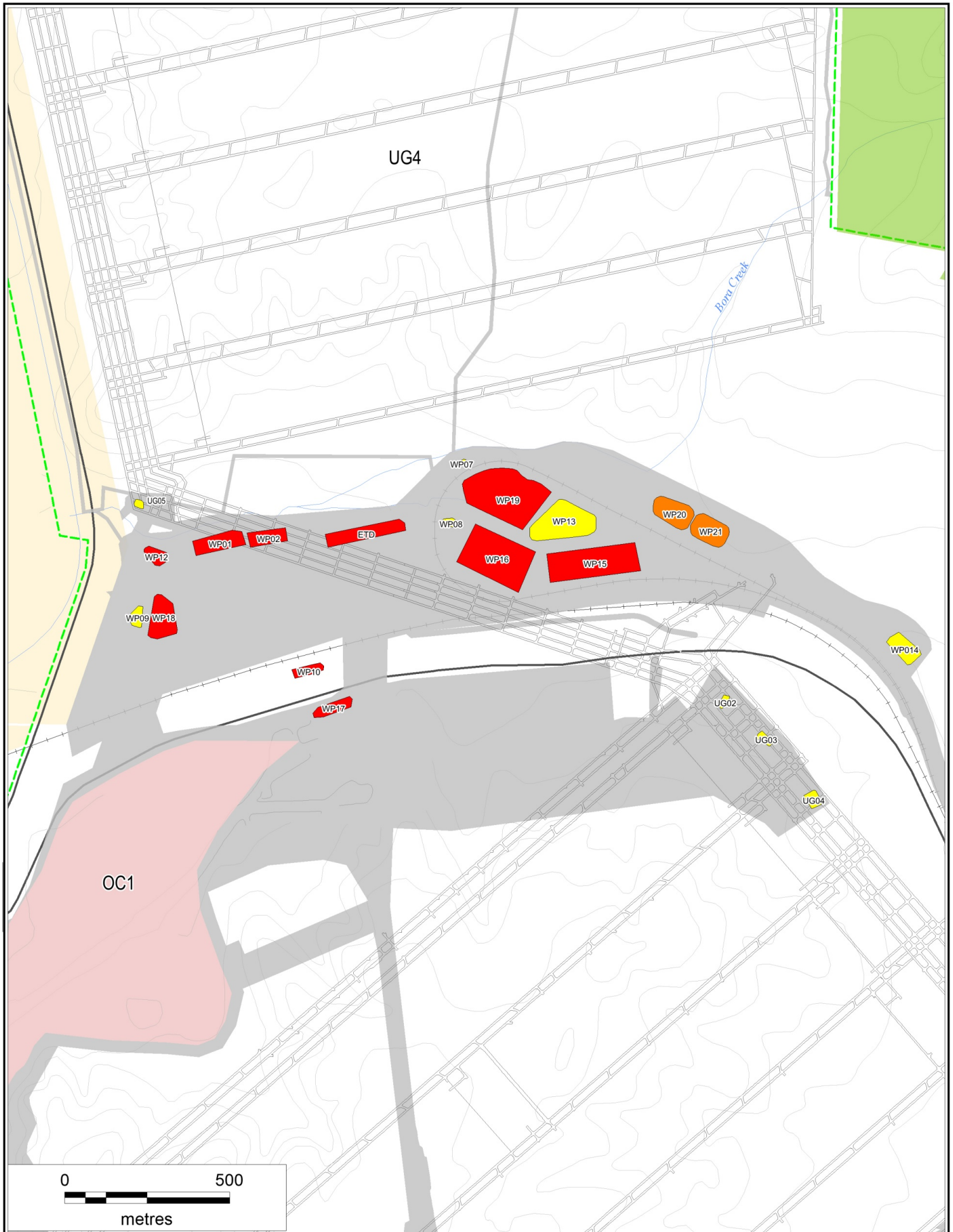
Figure 6 Location of Water Storage and Sediment Dams in CHPP Area
