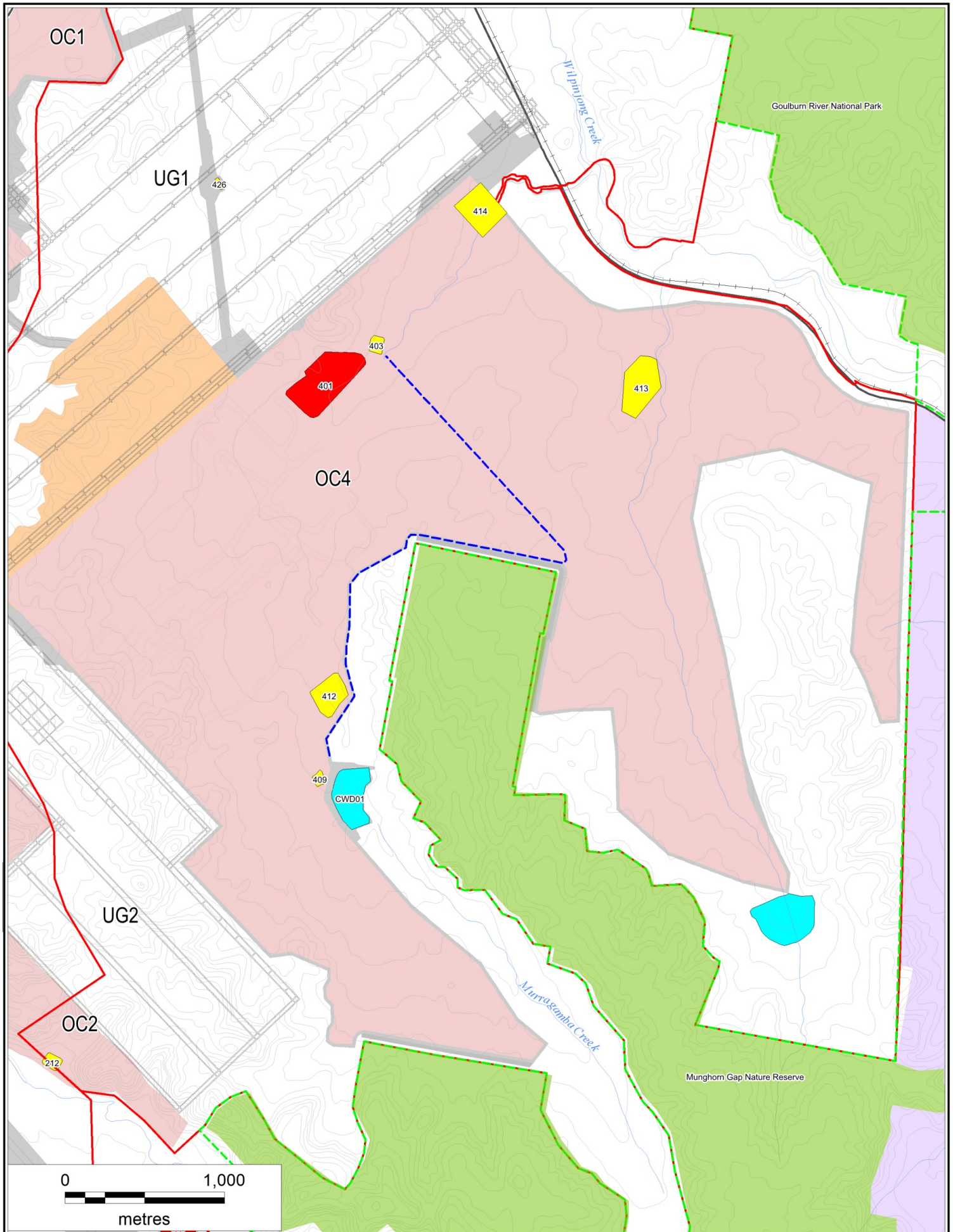
Figure 10 Location of Water Storage and Sediment Dams in OC4
