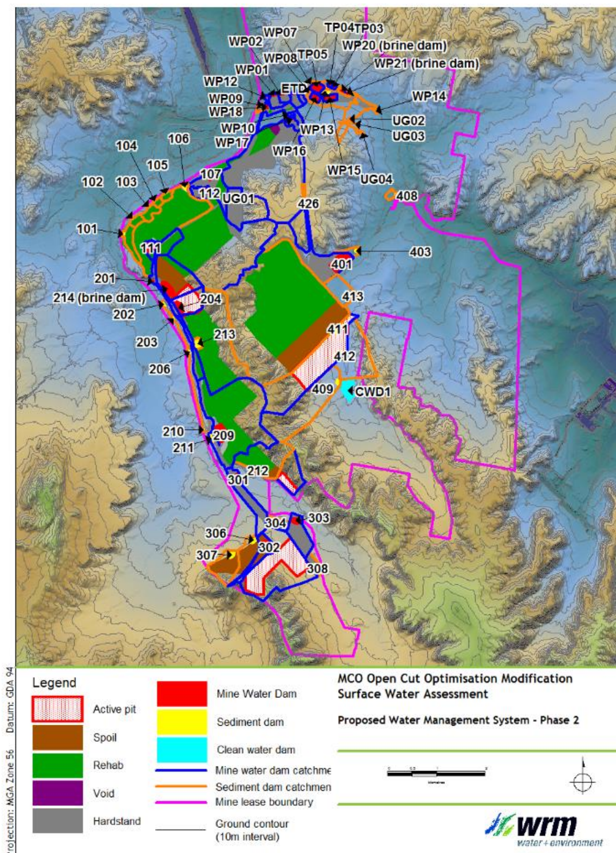
Moolarben Coal Complex Stage Plans – Phase 2 (indicatively 2020 to 2021)
