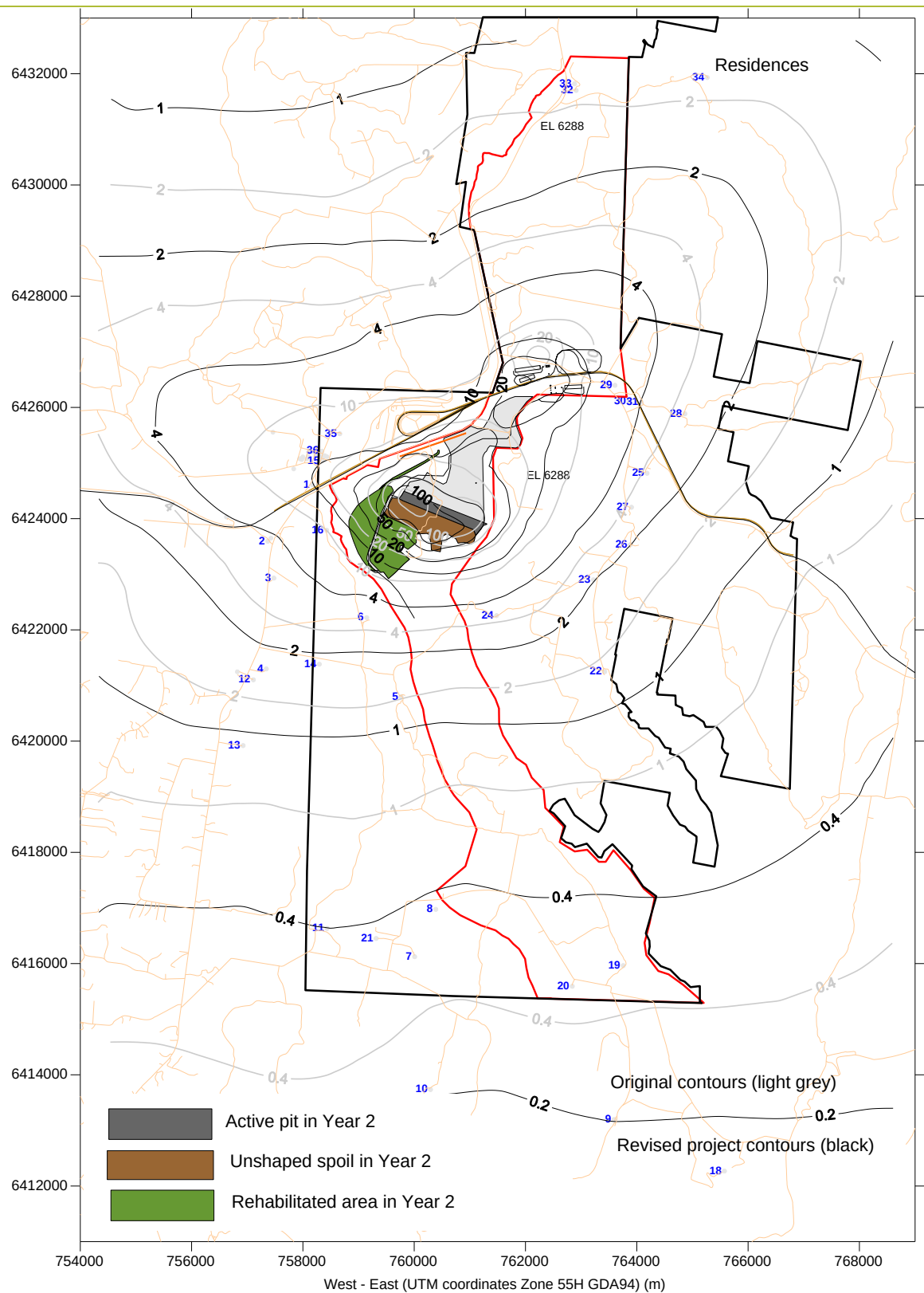
Comparison of predicted annual average PM_{10} concentrations due to emissions from original (grey) and revised (black) Moolarben mine in Year 2 - \mu g/m^3
