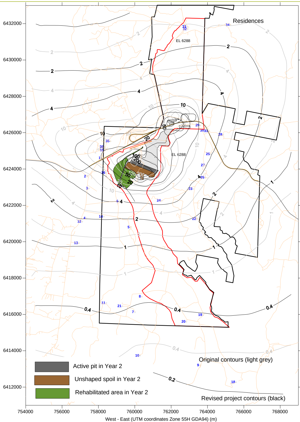
Comparison of predicted annual average TSP concentrations due to emissions from original (grey) and revised (black) Moolarben mine in Year 2 - \mu\text{g}/\text{m}^3
