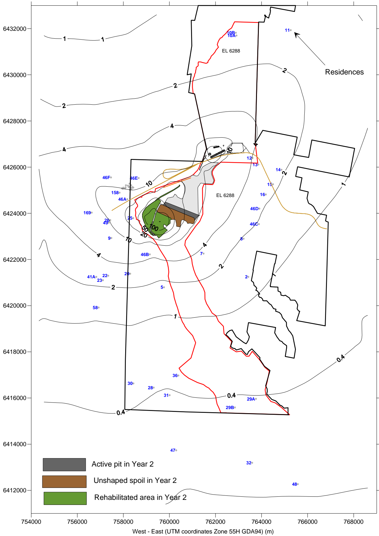
Predicted annual average PM 10 concentrations due to emissions from Moolarben in Year 2 - µg/m 3
