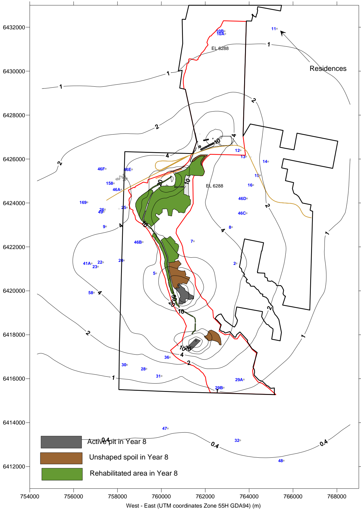
Predicted annual average PM_{10} concentrations due to emissions from Moolarben in Year 8 - \mu g/m^3
