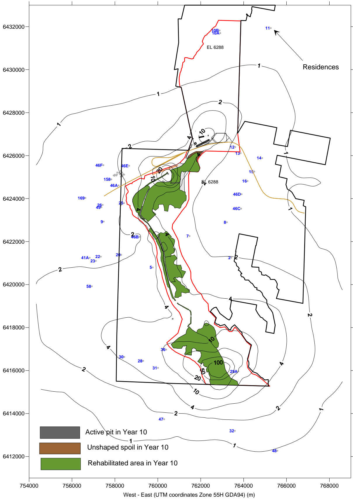
Predicted annual average PM_{10} concentrations due to emissions from Moolarben in Year 10 - \mu g/m^3
