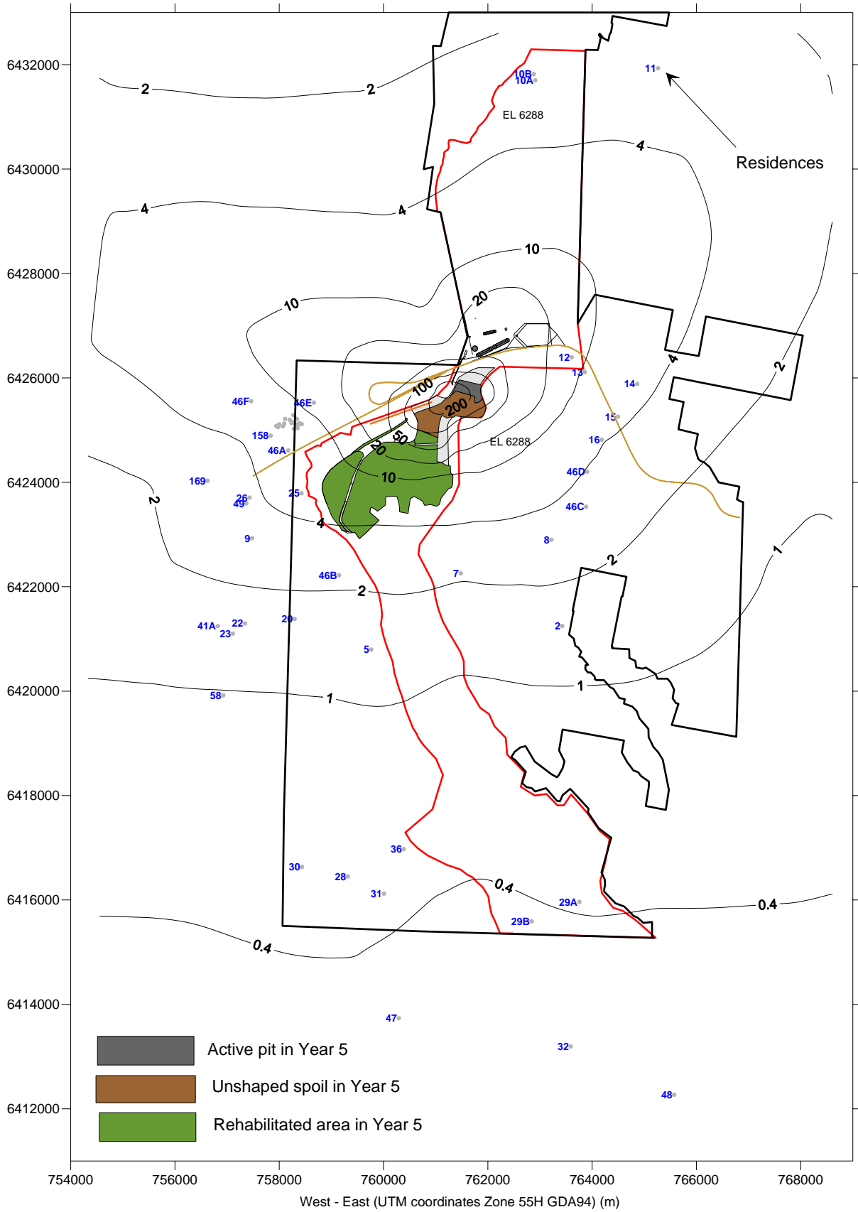
Predicted annual average PM 10 concentrations due to emissions from Moolarben in Year 5 - \mu\text{g}/\text{m}^3
