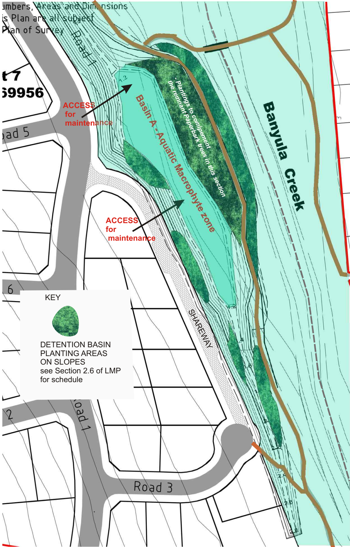
Plan 3a -BASIN A Conceptual Layout of plantings
