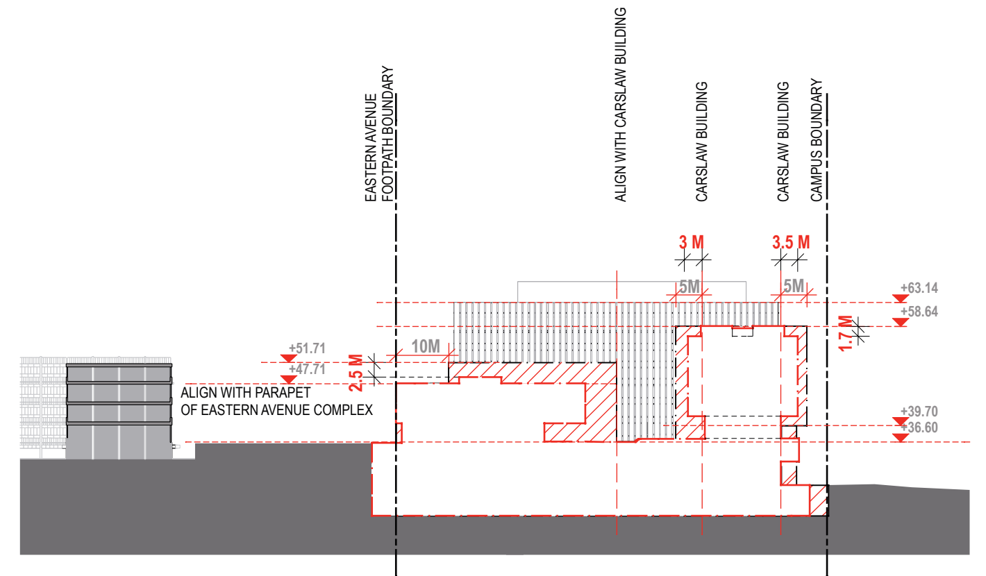
SECTION B
