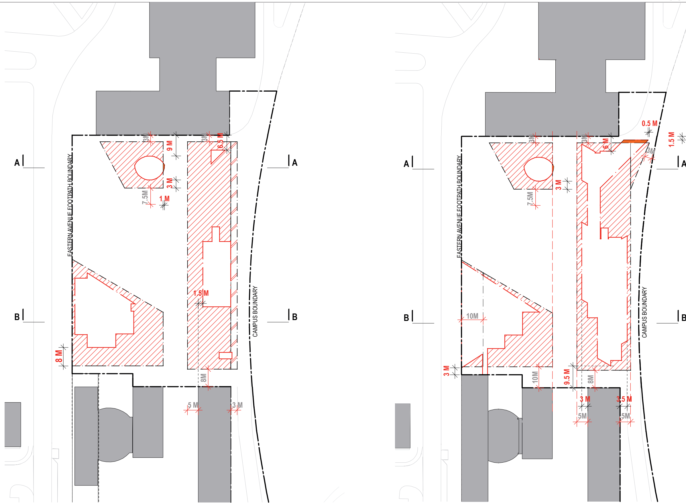
LEVEL 3 (EASTERN AVENUE LEVEL)
