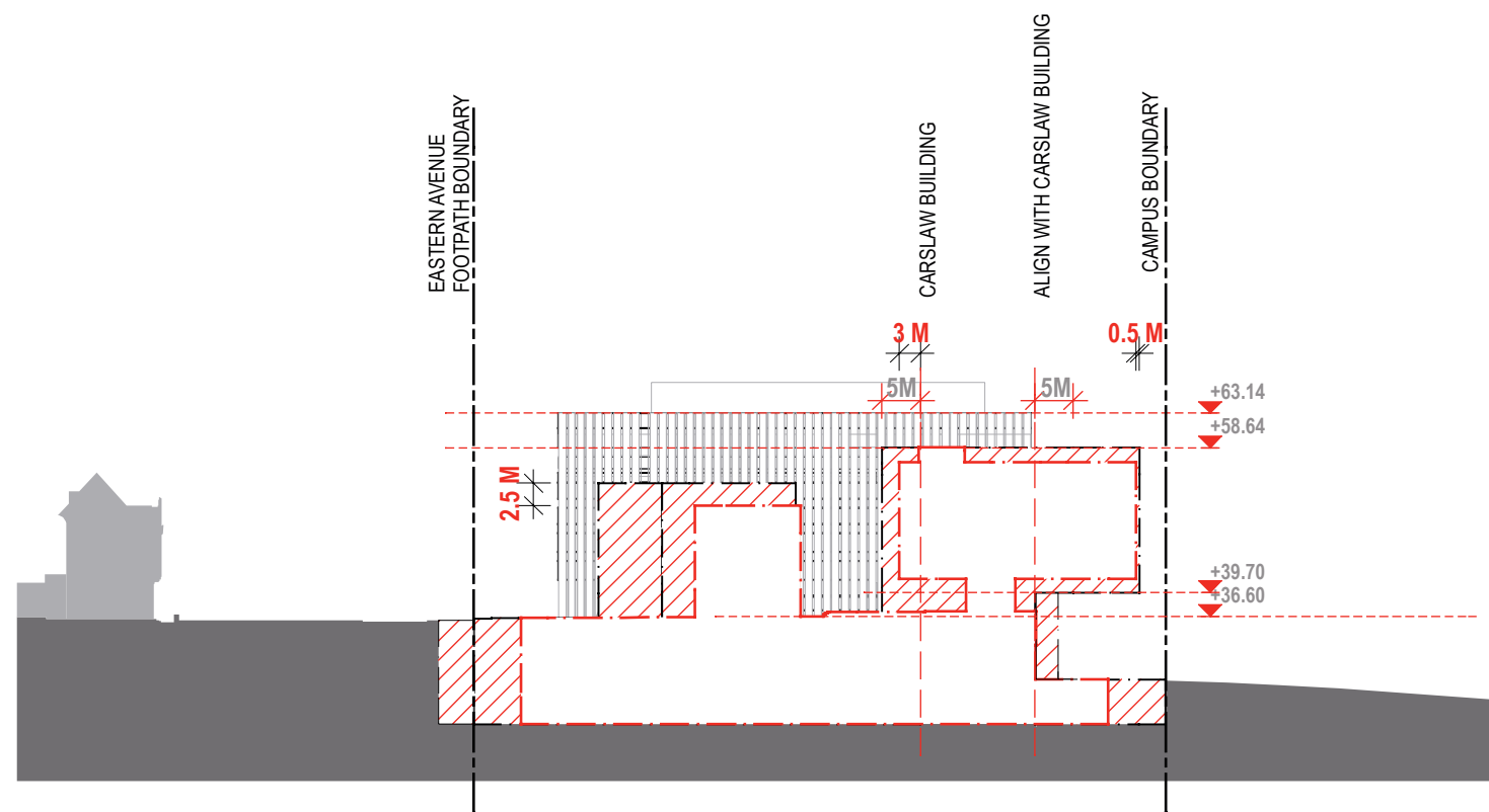
SECTION A
