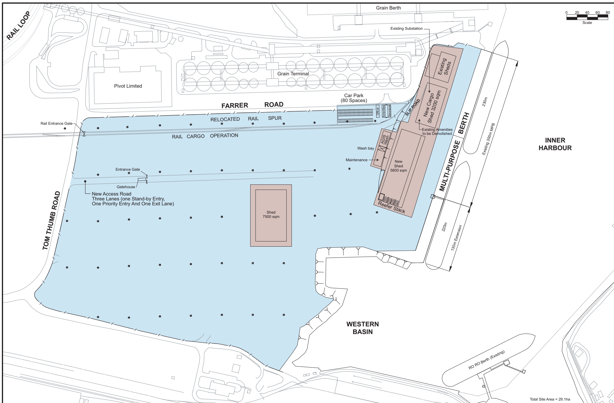
Figure 2.1 APPROVED DEVELOPMENT PROPOSAL
