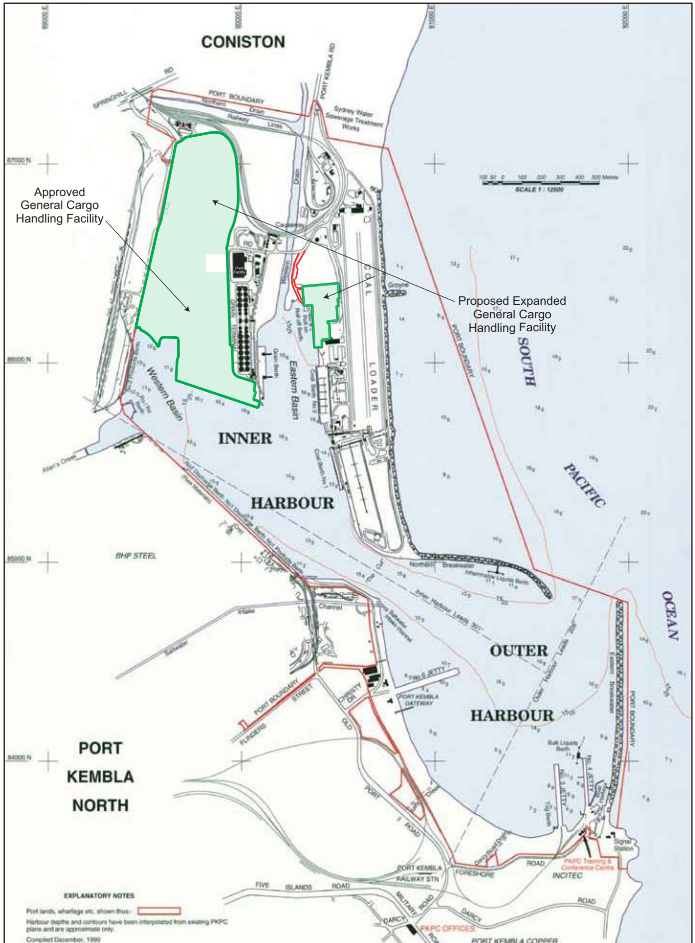
Figure 1.1 LOCALITY PLAN
