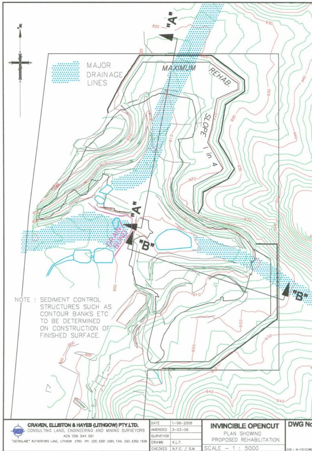
Figure 11 Proposed Rehabilitation Landform.
