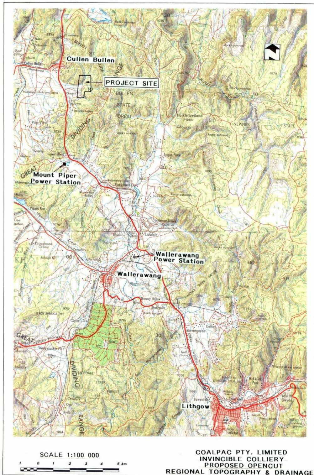
Figure 12 Regional Topography and Drainage.
