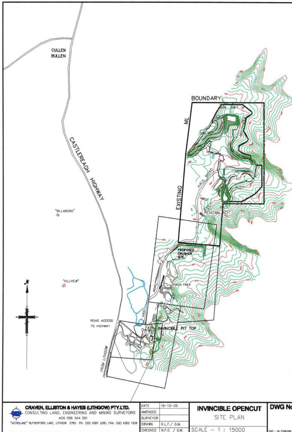
Figure 8 Invincible Open Cut Site Plan
