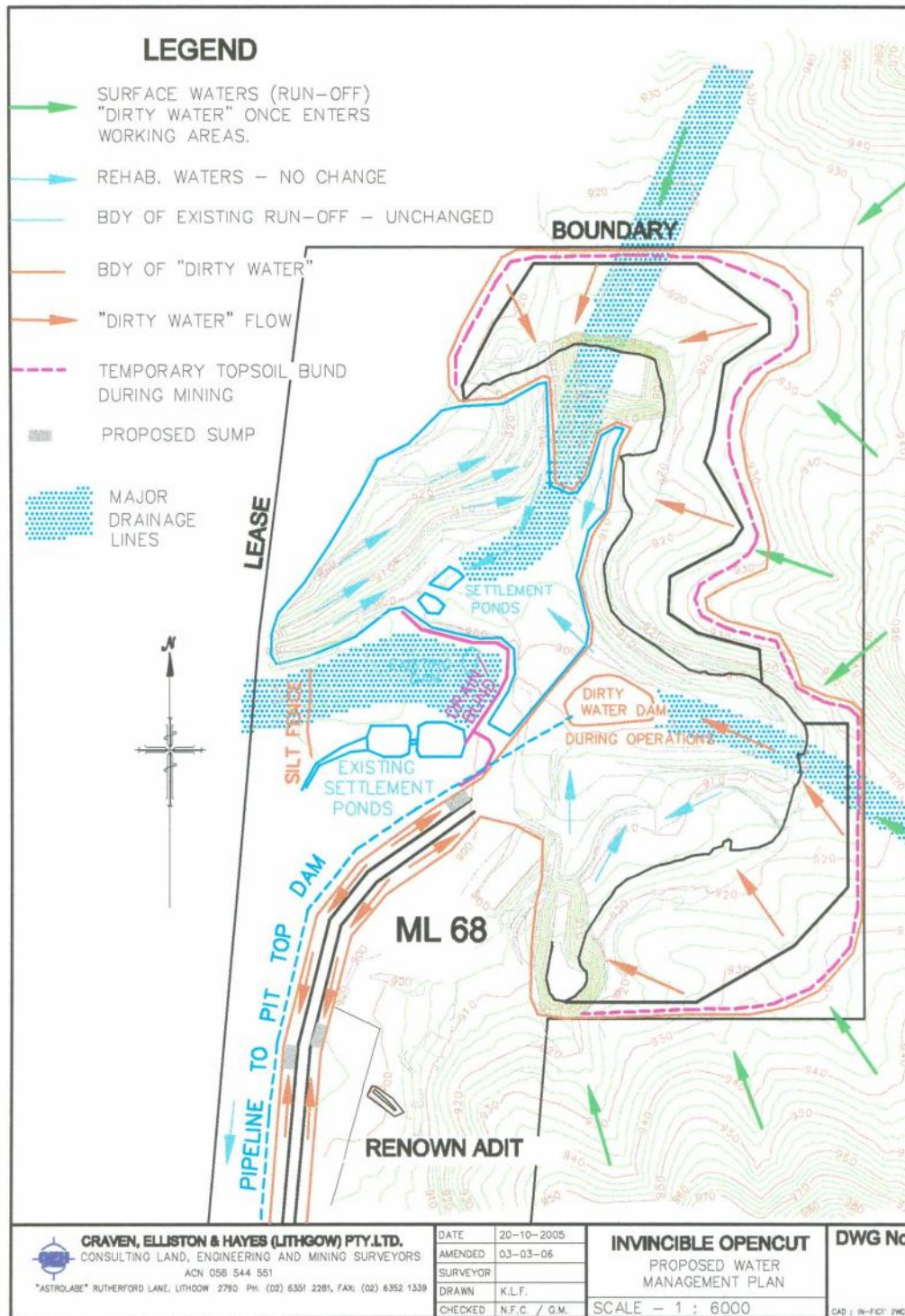
Figure 9 Open Cut Proposed Water Management Plan.
