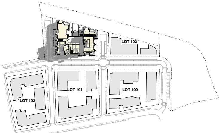
June 21 12.00
