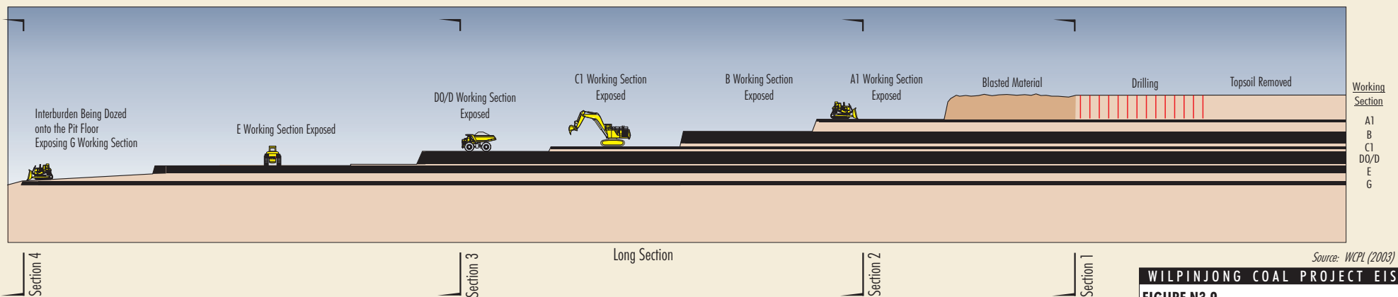
FIGURE N3.9 Conceptual Mining Method (Section View)
