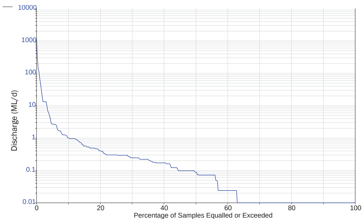
Figure 3.4 Derived Flow-Duration Relationship for Saddlers Creek at Bowfield (1956-1981)
