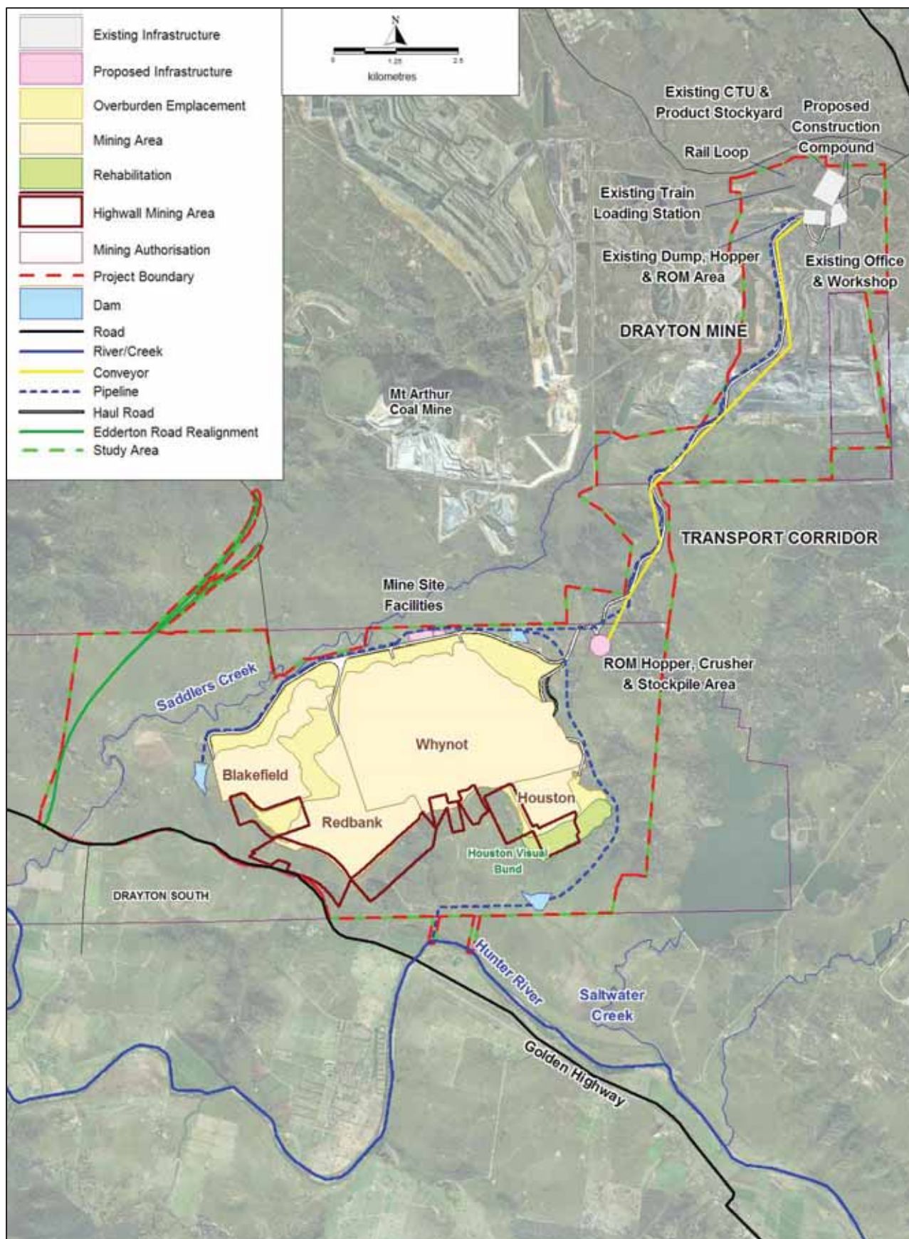
Figure 1.2 Conceptual Project Layout
