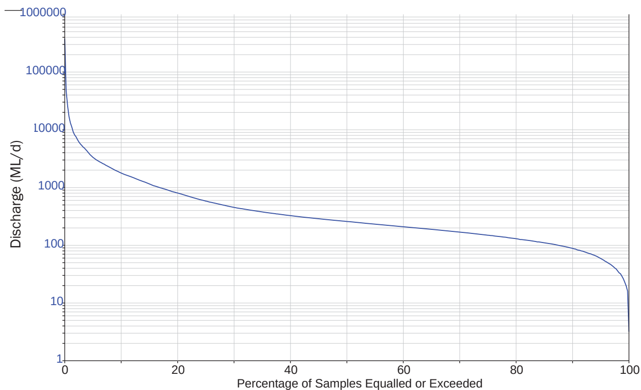
Figure 3.3 Recorded Flow-Duration Relationship for the Hunter River at Liddell (1969-2009)
