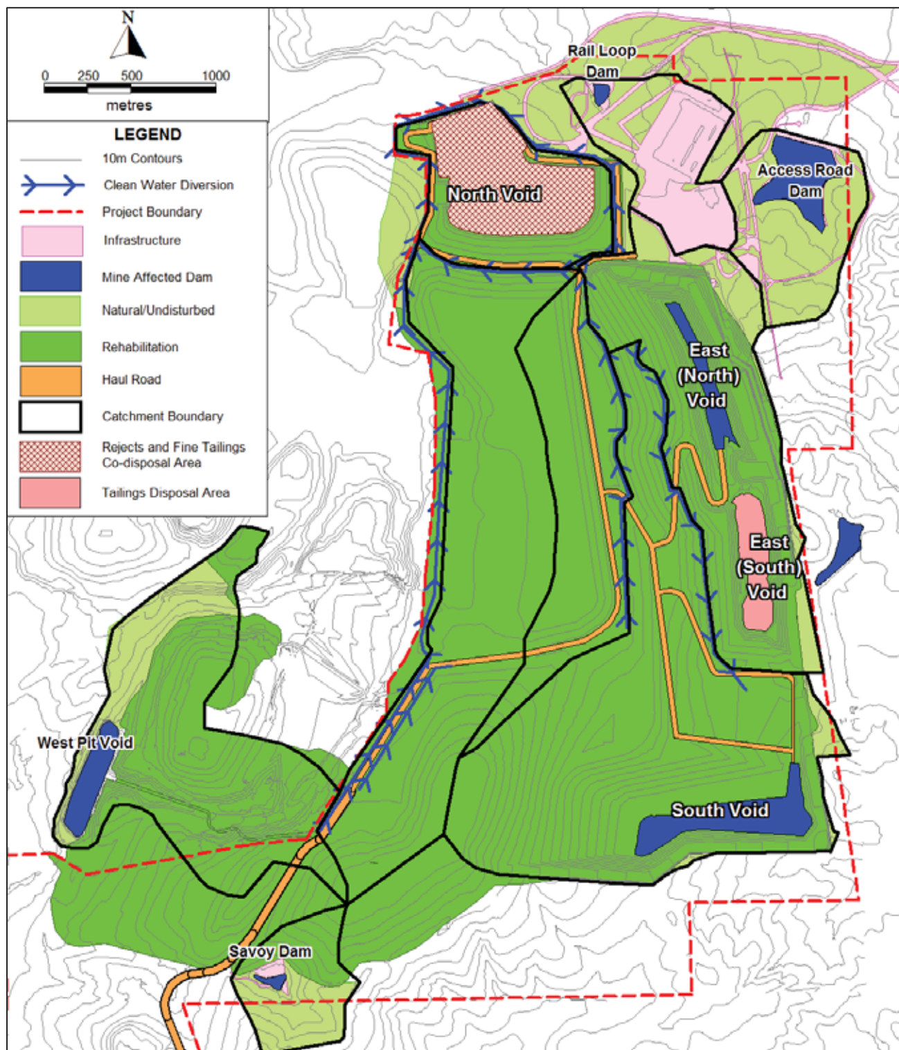
Figure 4.9 Drayton Mine Conceptual Landform Year 3-27 (Scenario 3)
