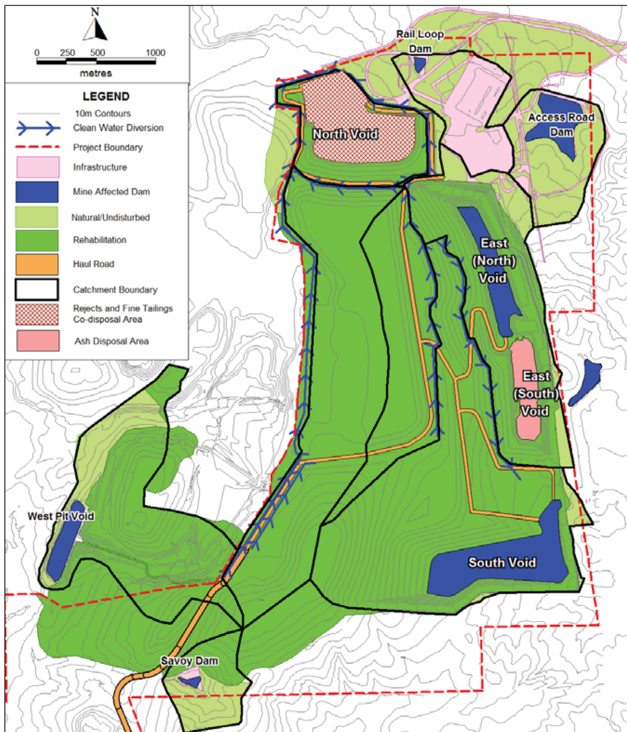
Figure 4.7 Drayton Mine Conceptual Landform Year 3-27 (Scenario 1)
