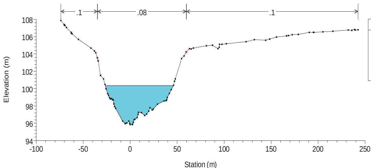
Figure 3.6 Saddlers Creek HEC-RAS Model (XS70) 100 Year ARI Flood Level
