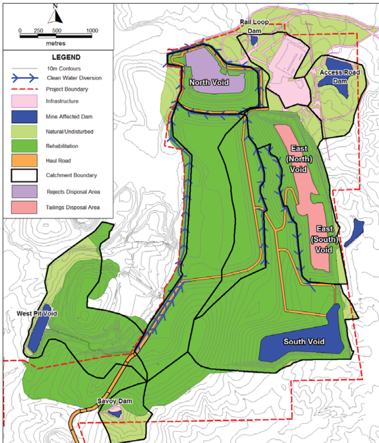
Figure 4.8 Drayton Mine Conceptual Landform Year 3-27 (Scenario 2)
