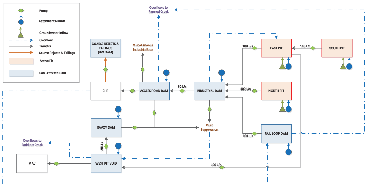
Figure 3.8 Drayton Mine Water Management System Schematic
