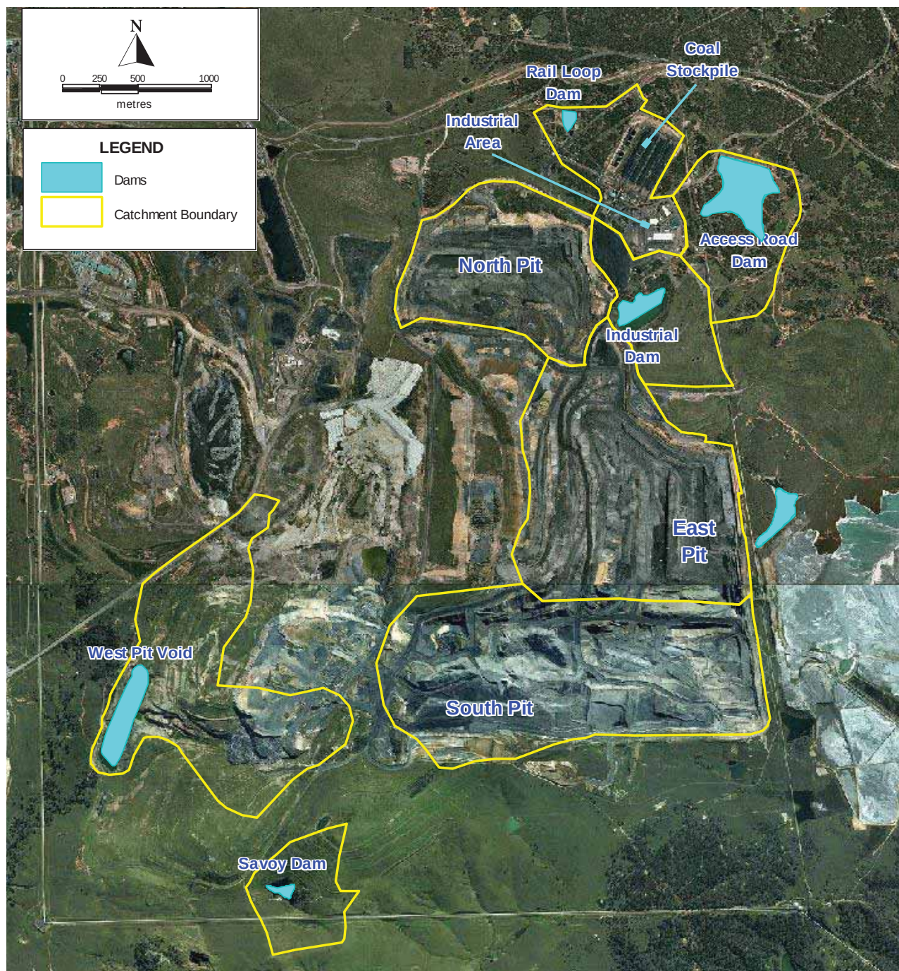
Figure A 3 Existing Drayton Mine Catchment and Operational Areas
