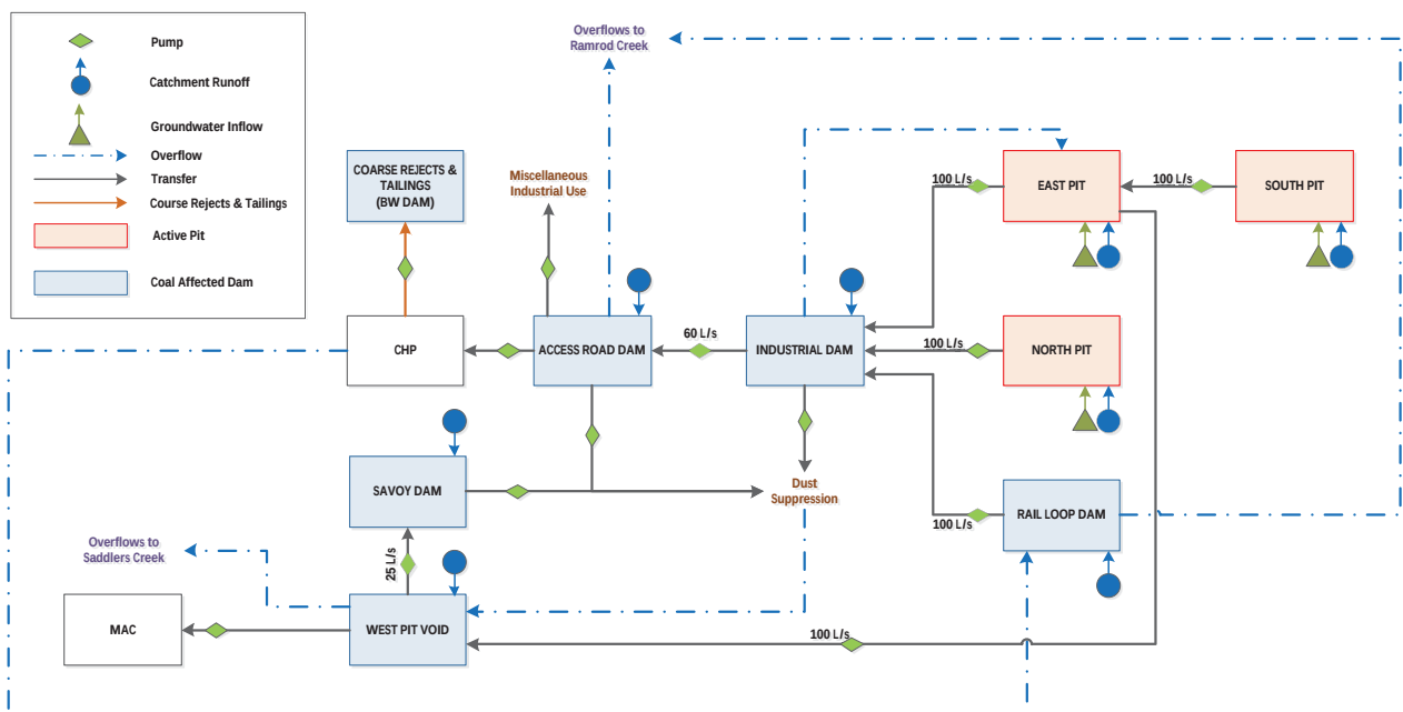
Figure A 2 OPSIM Model Schematic of Drayton Mine Water Management System for the Calibration Period, January 2007 to May 2011
