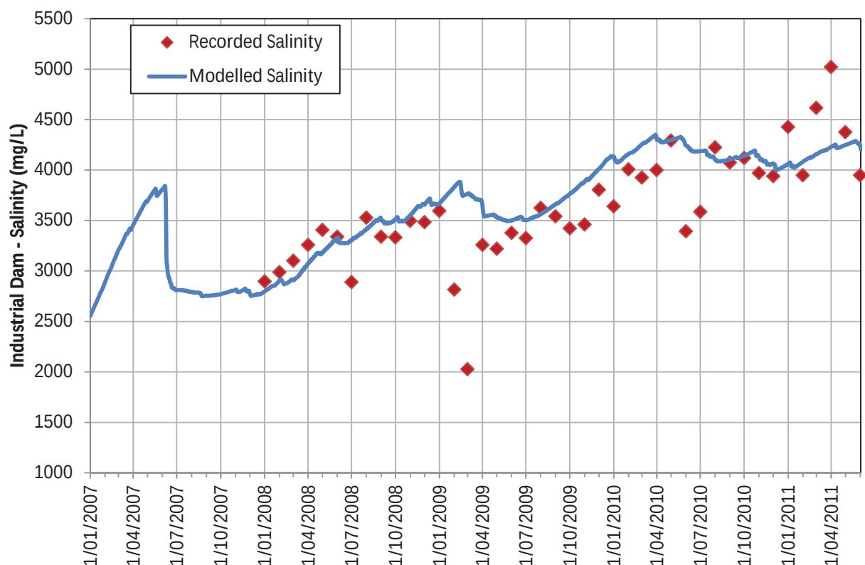
Figure A 6 Modelled and Recorded Industrial Dam Total Dissolved Solids, Jan 2007 to May 2011
