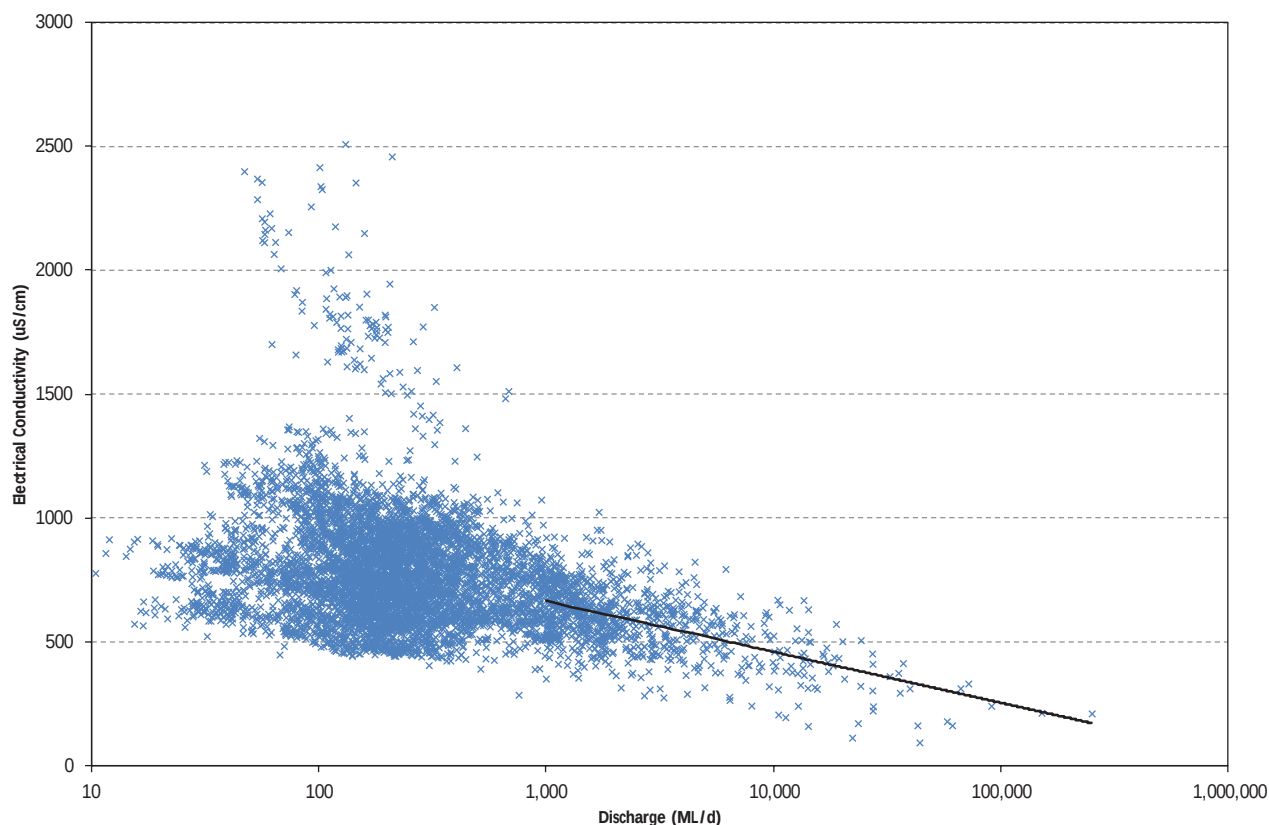
Figure 3.7 Stream Flow and Electrical Conductivity Relationship for the Hunter River at Glennies Creek
