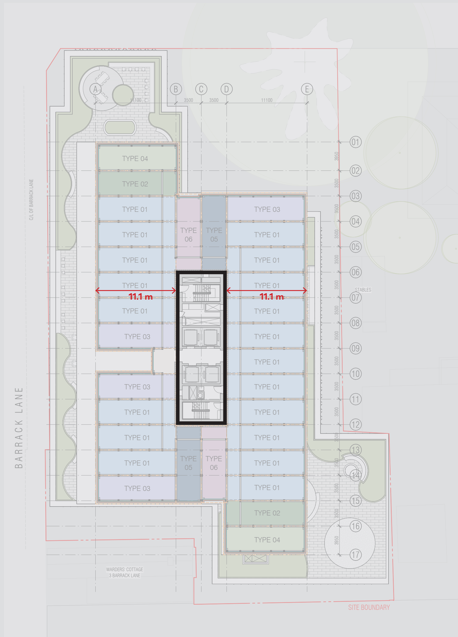
VMC MODULE CONFIGURATION
