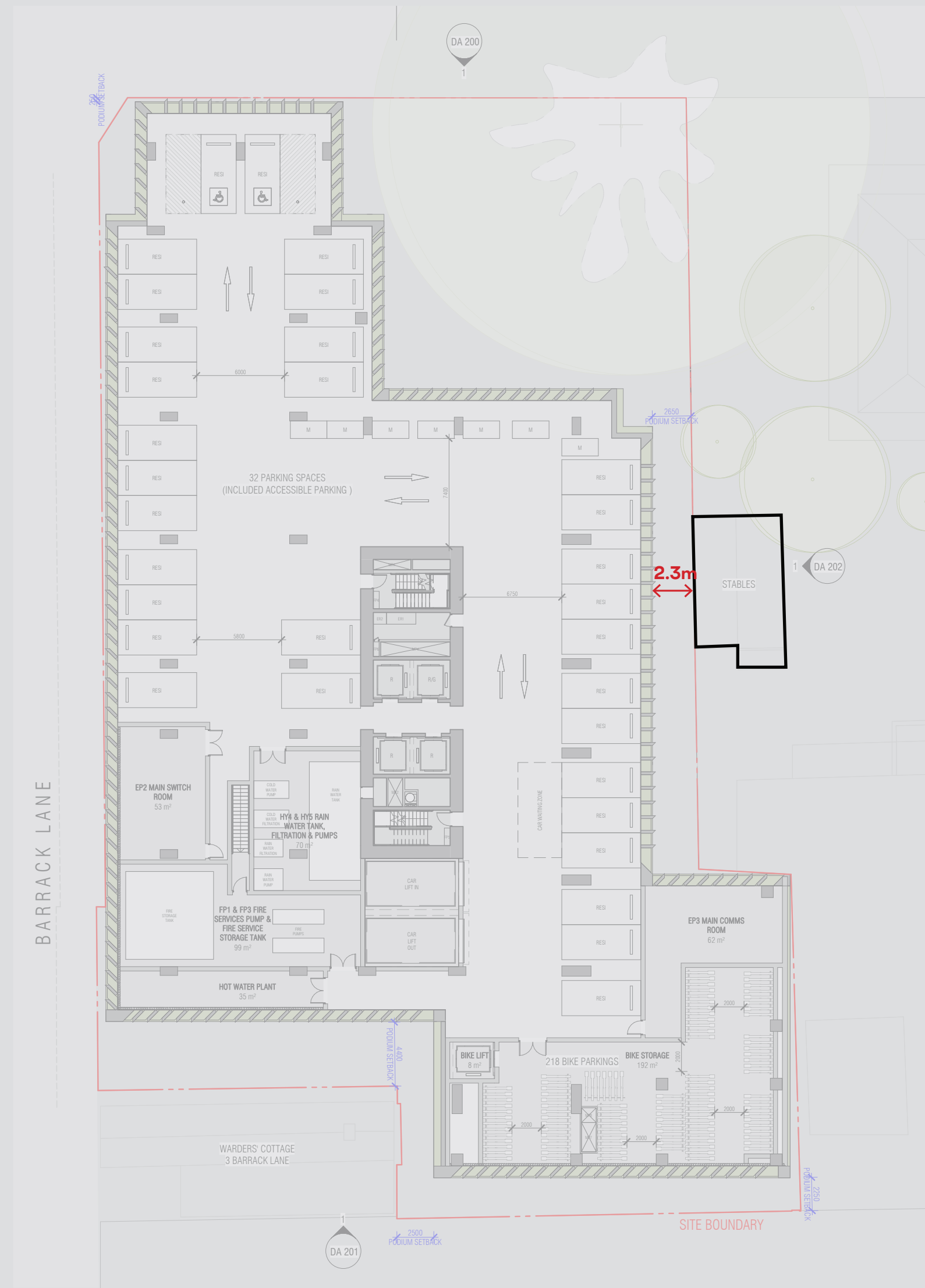
UPPER LEVEL PODIUM CONNECTION TO THE STABLES
