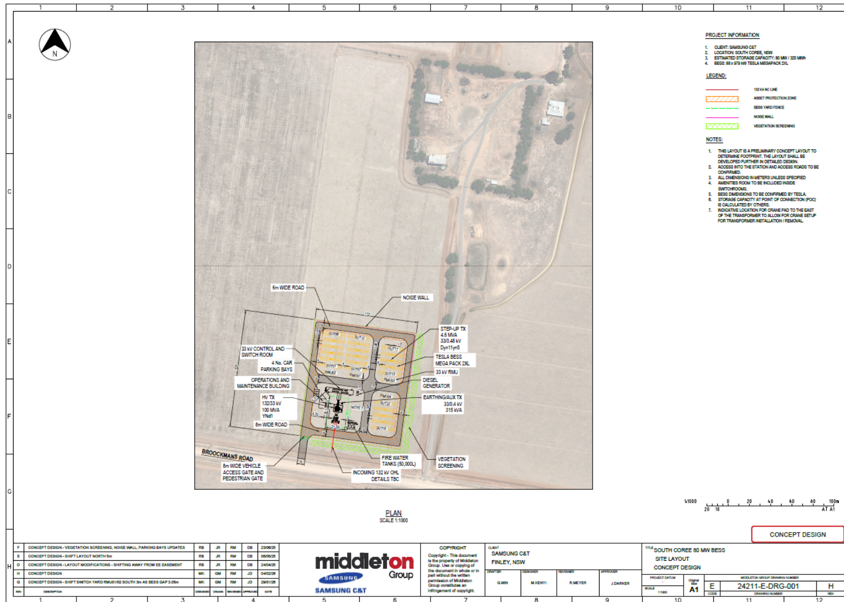
Figure 3-2 Project site layout concept design (source: the Applicant)
