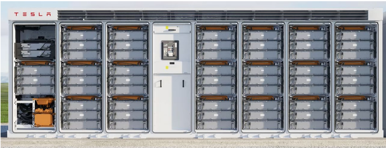
Figure 3-4 Battery module and inverter example (source Tesla.com)
