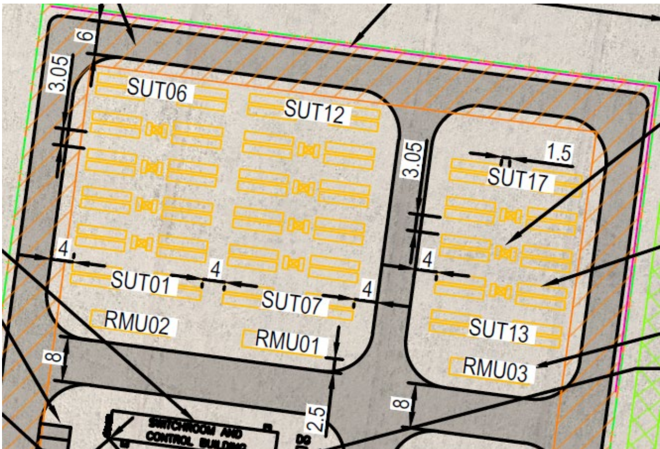
Figure 3-5 BESS separation distances (source: the Applicant)
